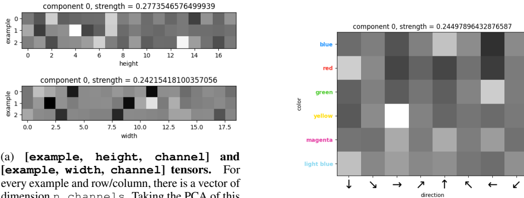
(b) [direction, color, channel] tensor. A similar style PCA decomposition: the graph shows the top principal component for this tensor. The four brightest pixels identify blue with up, green with left, red with down, and yellow with right. This tensor tells each direction which color to use for the opposite edge's box. The top principal component is 829 times stronger than the next principal component.
