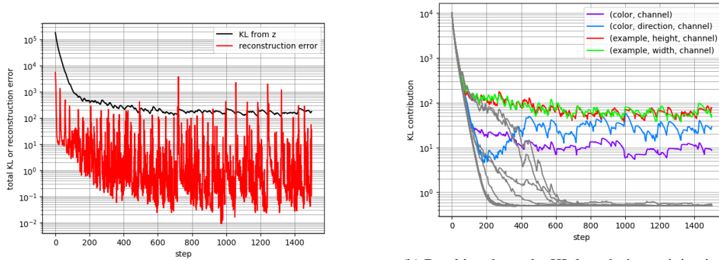
(b) Breaking down the KL loss during training into contributions from each individual shaped tensor in the multitensor z . Four tensors dominate, indicating they contain information, and the other 14 fall to zero, indicating their lack of information content.
