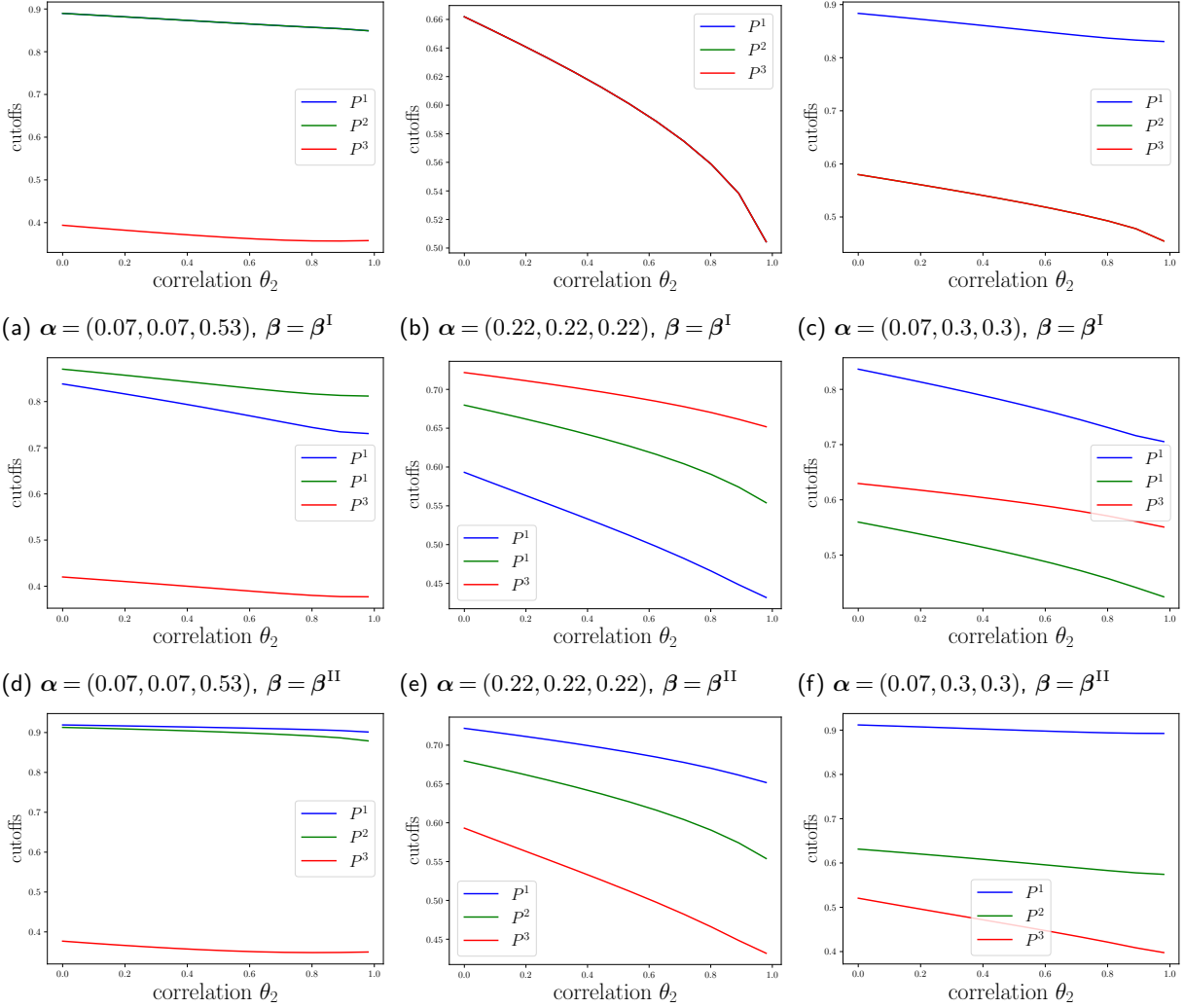
Figure 9 Variations of the cutoffs for three colleges.
