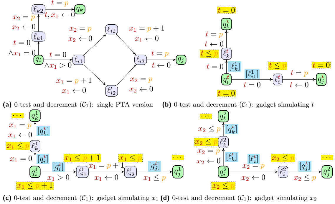
■ Figure 4 0-test and decrement gadget
