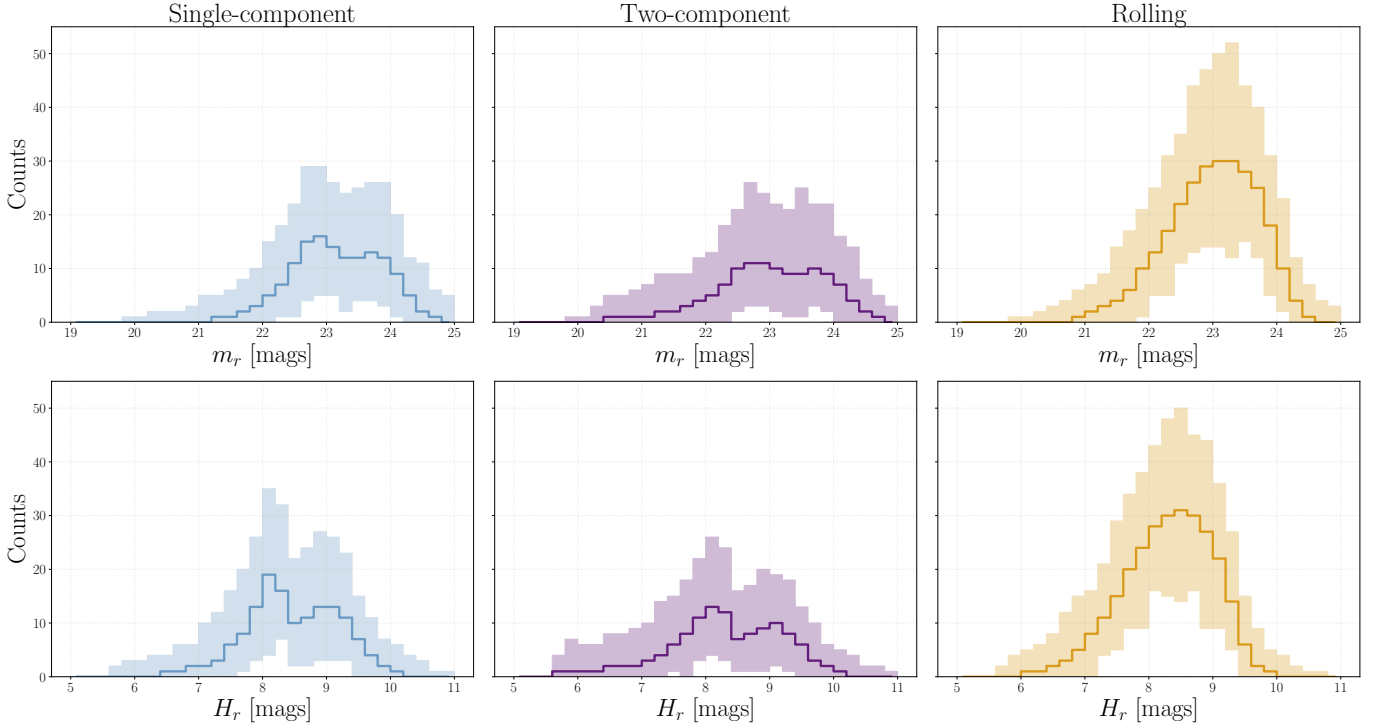
Figure 8. Final ten yr differential histograms of ( top row ) the median apparent magnitude distribution in r band at time of linkage of detected NTs for the three input models, and ( bottom row ) the median absolute magnitude in r band of all detected NTs. The shaded region on each represents the uncertainty on all 10^3 simulations.
