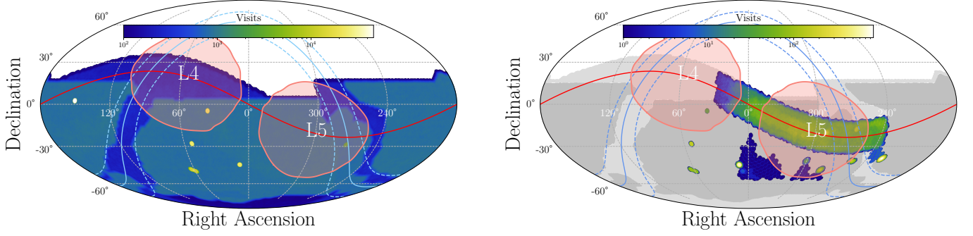
Figure 1. Sky maps of the number of visits across all filters of ( left ) the 10 year LSST survey cadence based on the one snap v4.3.1 simulation (SCOC 2024) and ( right ) the Science Validation survey based on the lsstcam.20250930 simulation (C. Claver et al. 2025; NSF-DOE Vera C. Rubin Observatory 2025) —note the difference in color scale between the two. The main wide-fast-deep survey makes up \sim 80\% of the total main LSST survey time, receiving on average \sim 800 visits per pointing. Also of note are the Northern Ecliptic Spur (NES) mini-survey (dark blue region, +10^\circ ecliptic latitude) and the Deep Drilling Fields (yellow-white circles, regions with high temporal sampling cadence). For full details of the survey strategy, see SCOC (2024). Overplotted on both in solid red is the ecliptic plane. In solid blue is the galactic plane, with the corresponding dashed cyan lines representing \pm 10^\circ . On top of all of this in pink are the positions of both L4 and L5 clouds at the beginning of the survey for context.
