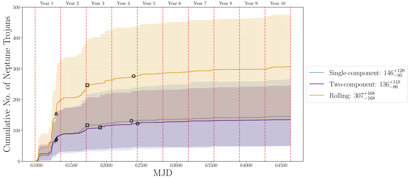
Figure C2. Cumulative histogram (with a bin size of one day) of the discovery rates over the 10 year LSST lifetime for the single-component (blue), two-component (purple), and rolling power law (orange) models. The points of 50% (open triangle) 80% (open square), and 90% (open circle) completion are shown for each model. Red dashed vertical lines represent survey year start/end points. The ranges here represent the upper and lower estimate for the scaling parameters used in each model, described in Section 2.3.1.
