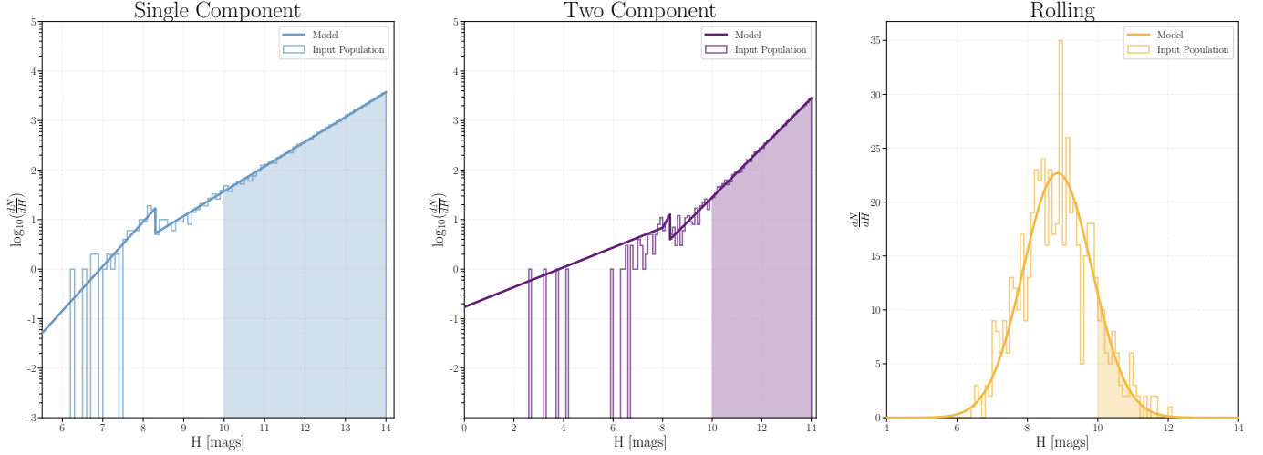
Figure 2. Differential histograms of all 3 absolute magnitude H distributions used in modeling the NT population in this work. In all cases, the solid line represents the analytical model for the distribution, whilst the histograms are the uniformly sampled N_{NT} objects from that model. The shaded regions in all cases represent the region beyond the LSST’s nominal single-visit detection threshold ( H_r \approx 10 ) for an object at Neptune’s orbit. Represented here are ( left panel ) the single-component model, ( middle ) the two-component model, and ( right ) the rolling power law model. Note that the single- and two-component models have a logarithmic y-axis scale, whilst the rolling power law model is linear.
