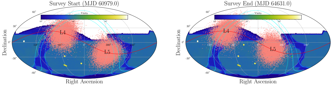
Figure 7. Sky coverage of an entire input intrinsic NT orbital model (pink scatter points) at the beginning of the survey (left) versus at the end of the survey (right) showing the bulk movement of the underlying clouds. In both projections, the L4 cloud is labeled on the left, whereas the L5 cloud is labeled on the right. The red solid line shows the ecliptic plane, and in light blue the galactic plane, with dashed lines marking \pm 10^\circ off of it.
