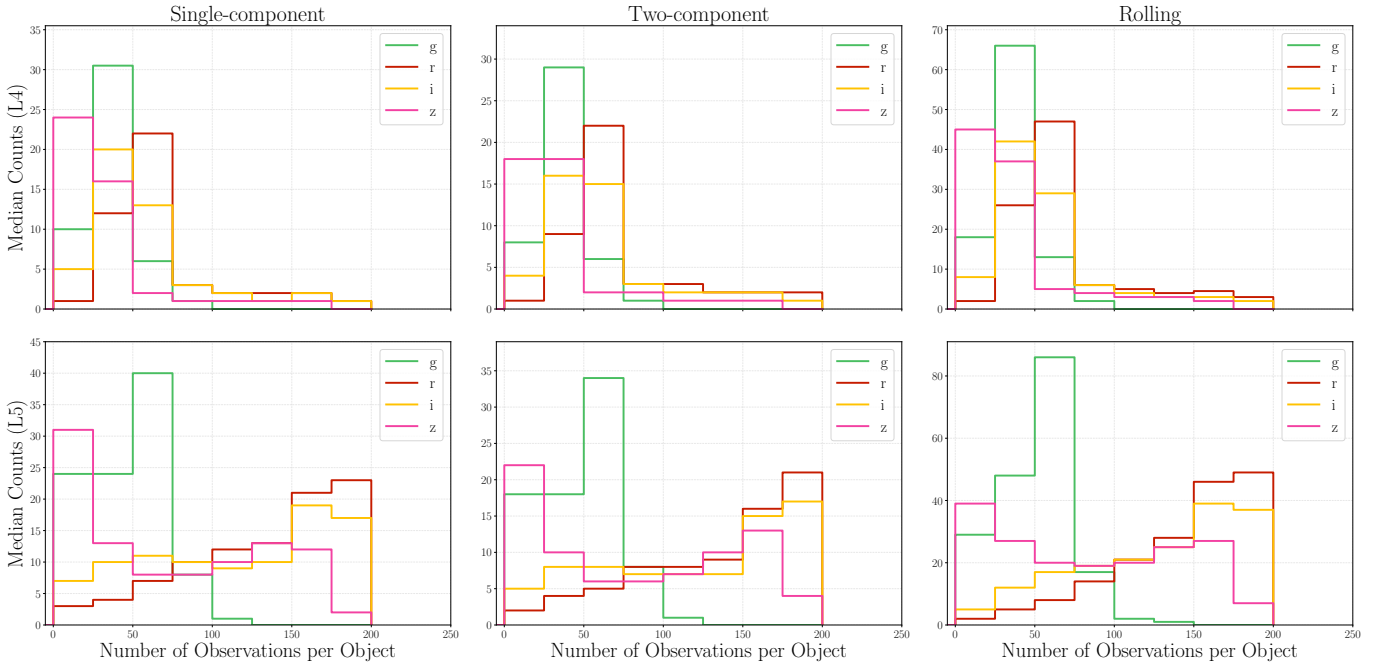
Figure 9. Histograms of the number of detections per object, broken down per filter for the three input models (columns) and by Lagrange cloud (L4 top row, L5 bottom row). All exclude any observations that fall within a DDF.
