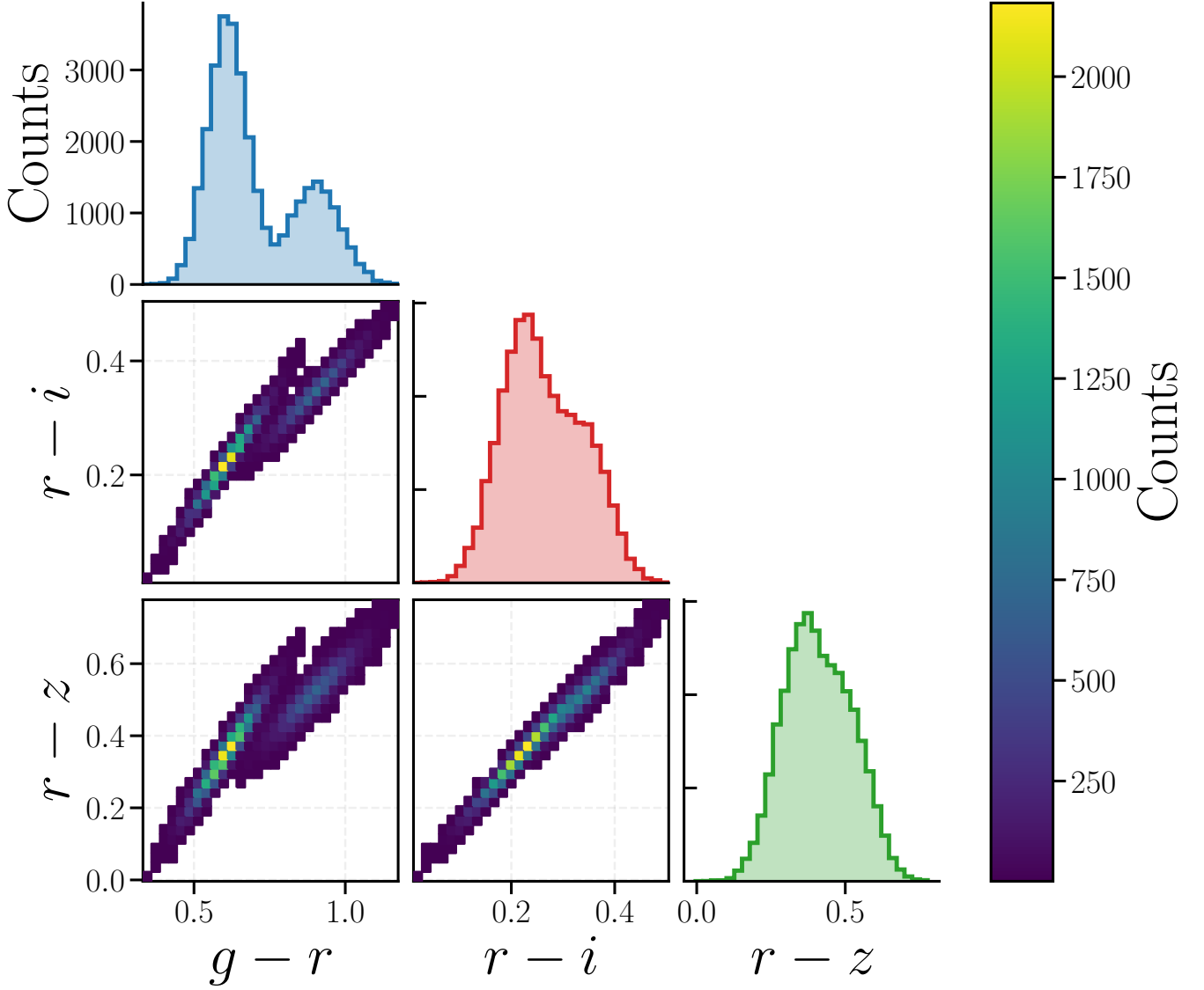
Figure 3. g-r , r-i , and r-z color histograms for the input model produced from GMM parameters in Table 1. The leading diagonal represents the individual 1D histograms of each color, whilst the middle left, bottom left, and bottom middle 2D histograms highlight their correlation. Samples are drawn to ensure this correlation is kept.
