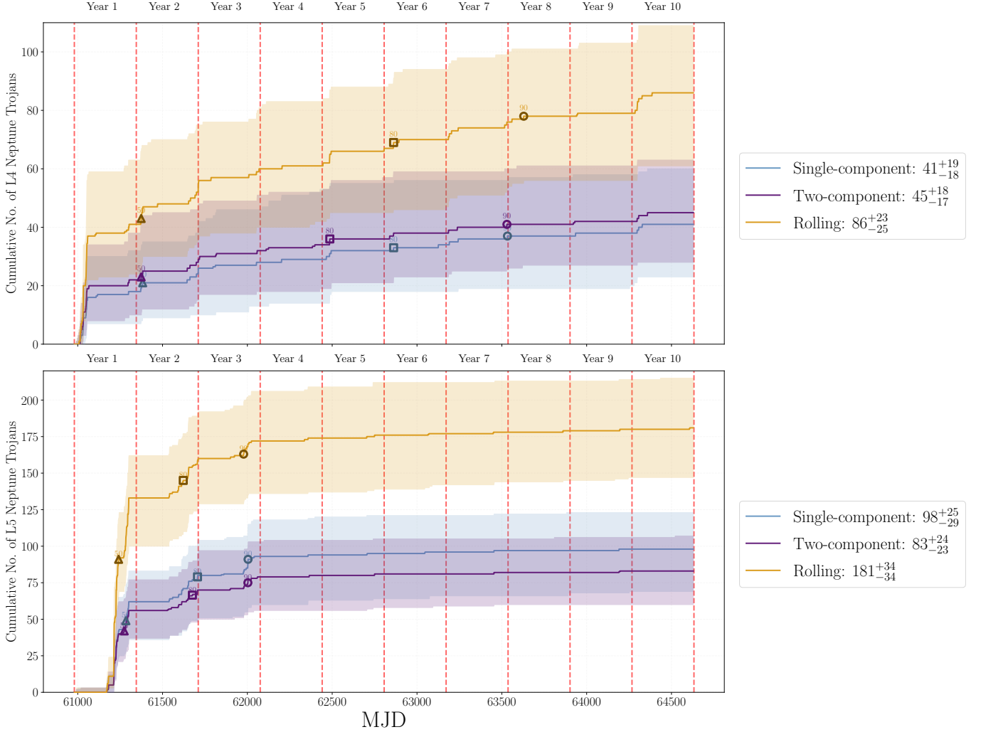
Figure 6. Cumulative histogram (with a bin size of one day) of the discovery rates over the 10 year LSST lifetime for the single-component (blue), two-component (purple), and rolling power law (orange) models. These are further split by ( top row ) L4 discoveries and ( bottom row ) L5 discoveries, with L5 discovery delayed until the cloud is observable in the survey. The points of 50% (open triangle) 80% (open square), and 90% (open circle) completion are shown for each model. Red dashed vertical lines represent survey year start/end points. The pronounced plateau in year 1 discoveries corresponds to an early surge of L4 detections, followed by a lull until sky rotation bring the L5 cloud into an observable airmass.
