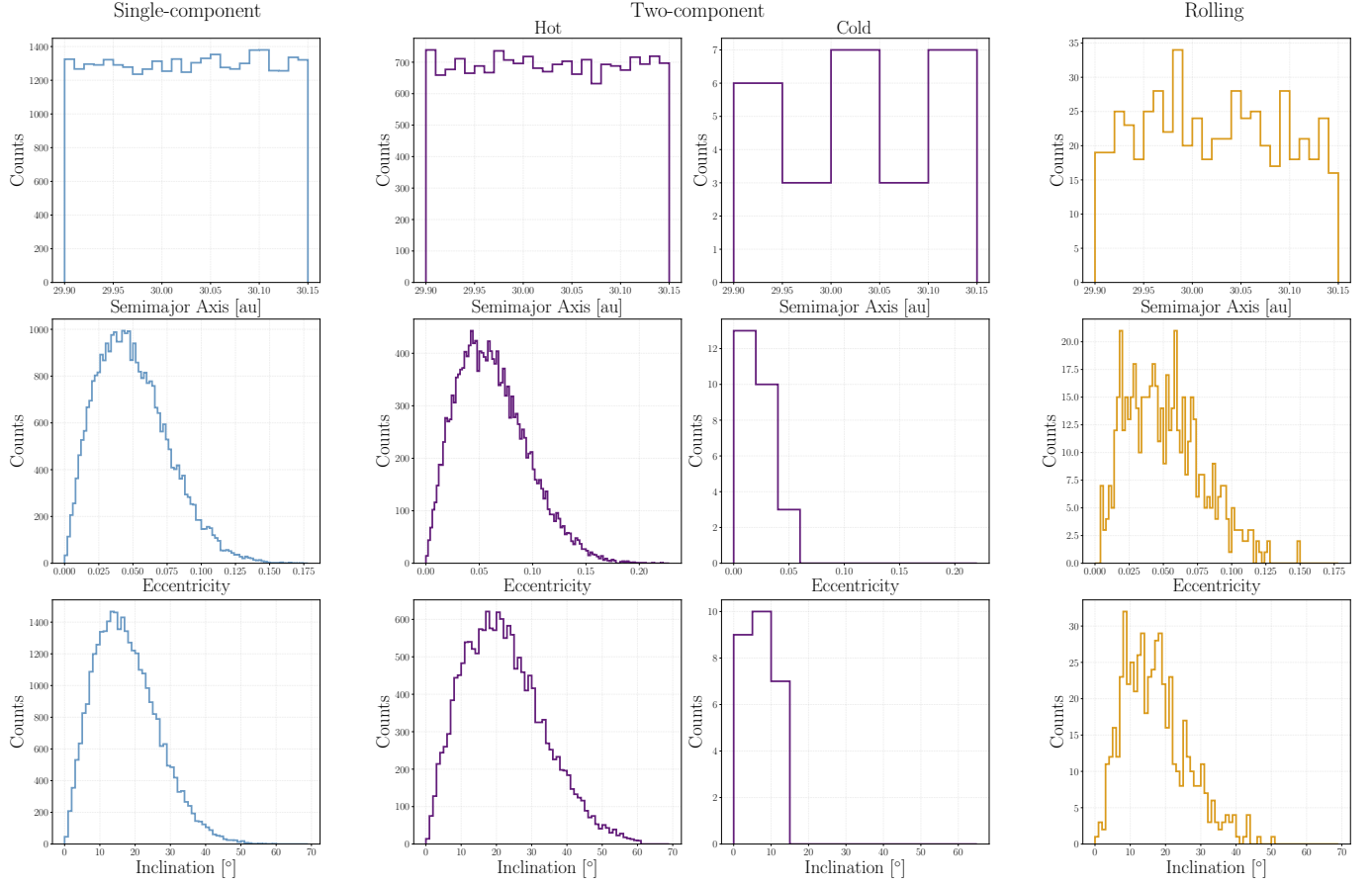
Figure 4. Orbital distributions in ( top row ) semimajor axis a , ( middle row ) eccentricity e , and ( bottom row ) inclination i for the ( left column ) single-component, ( middle column ) two-component, and ( right column ) rolling power law models respectively.
