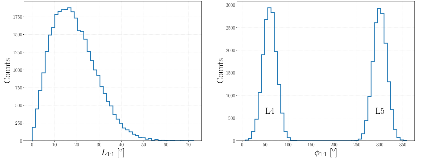
Figure 5. Example distributions of libration angle L_{1:1} and resonance argument \phi_{1:1} used for all 3 H models. All three H models share the same shape of distributions for L_{1:1} and \phi_{1:1} , only differing in the number of objects sampled from them.
