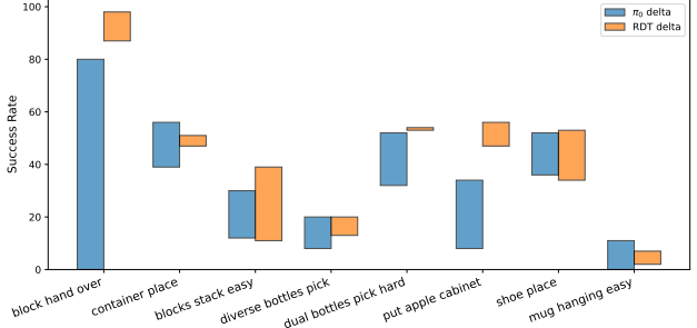
Figure 1 Illustrative Example: We fix the initial noise for the denoising process of \pi_0 to noise 1 and evaluate the success rate. Then we fix the initial noise for the denoising process of \pi_0 to another noise value noise 2 and evaluate the success rate under the same scenarios. We plot the two resulting success rates using a floating bar chart. The same procedure is applied to RDT.
