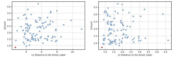
Figure 3 We performed 100 action samples for a single observation from the test set in each of the stamp seal (left), move can pot (right) tasks, and scored them using the pseudo-counter. The red points indicate the actions with the highest Count values, which generally correspond to the actions with the smallest L_2 distance to the action labels.
