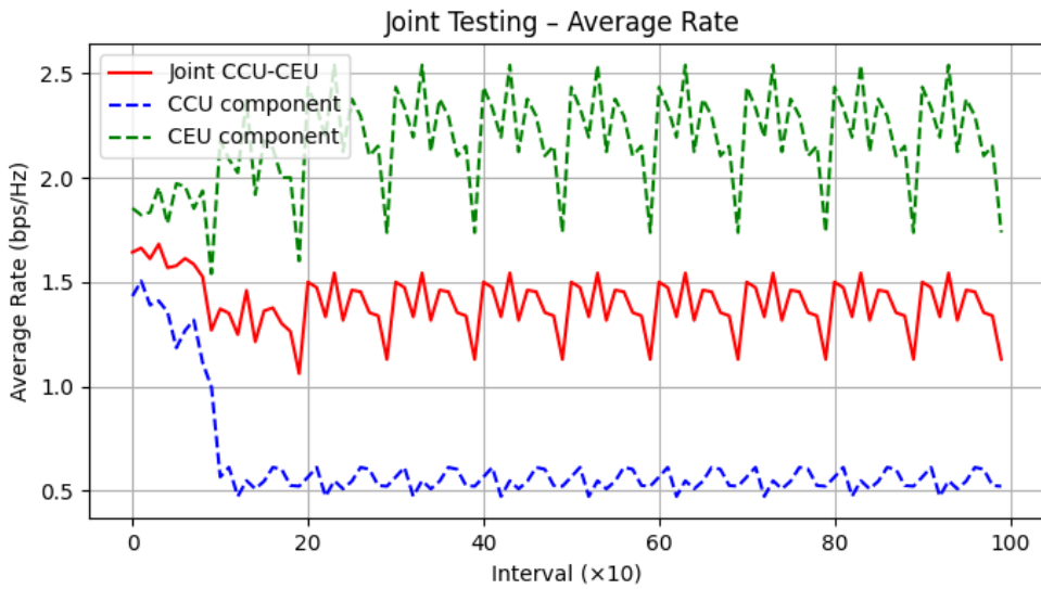
Figure 3. Testing - Average rate vs time intervals
