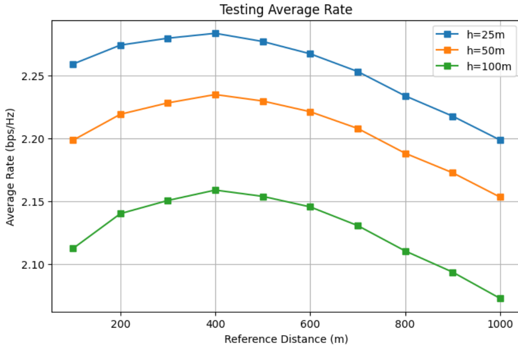
Figure 4. Average rate vs reference distance
