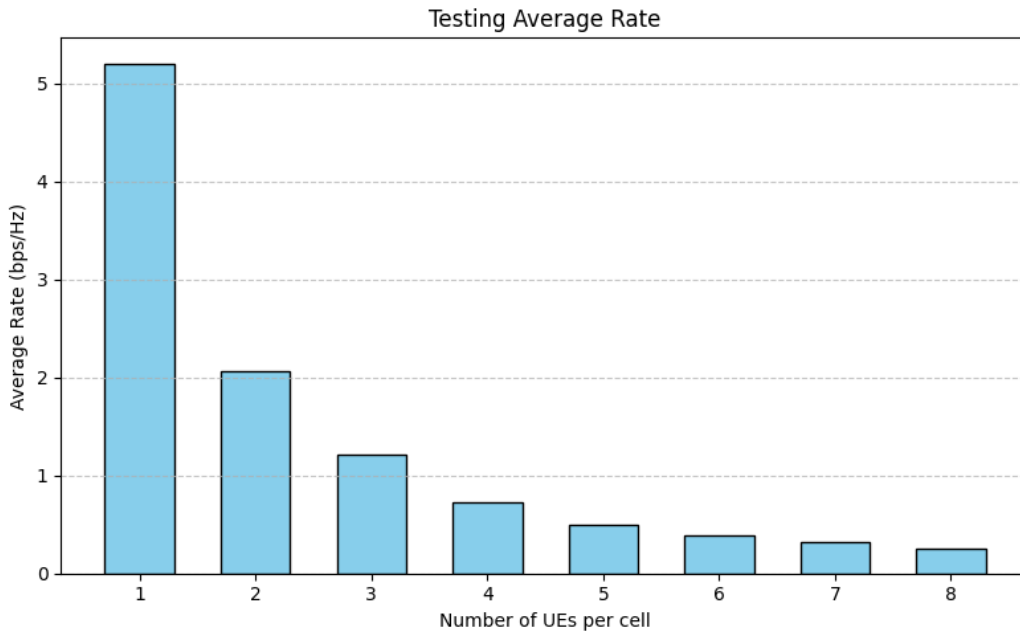
Figure 5. Average rate vs number of users
