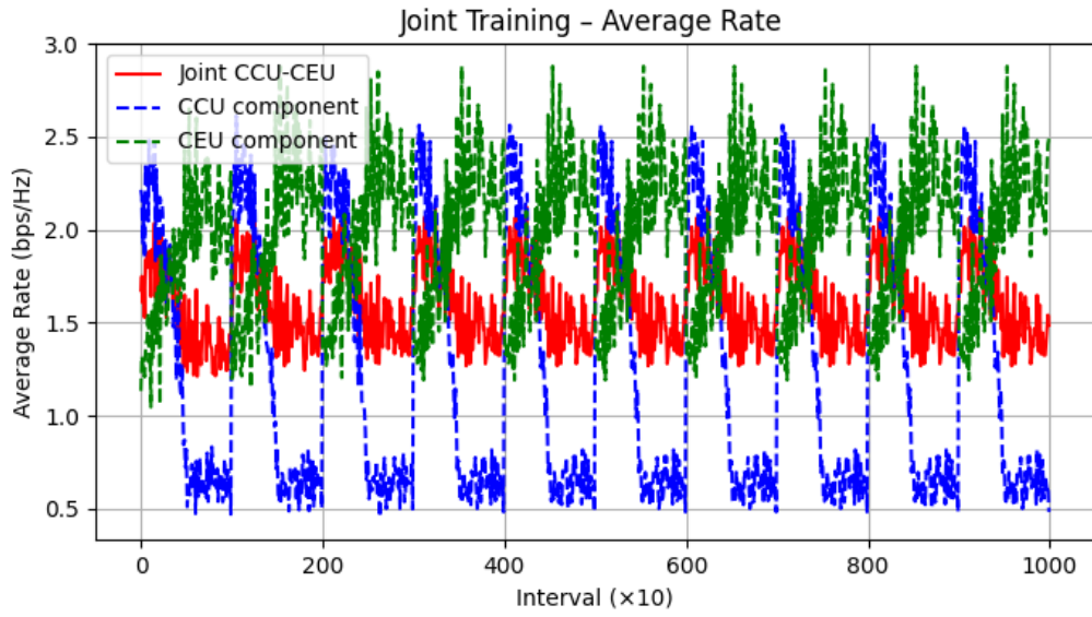
Figure 2. Training - Average rate vs time intervals
