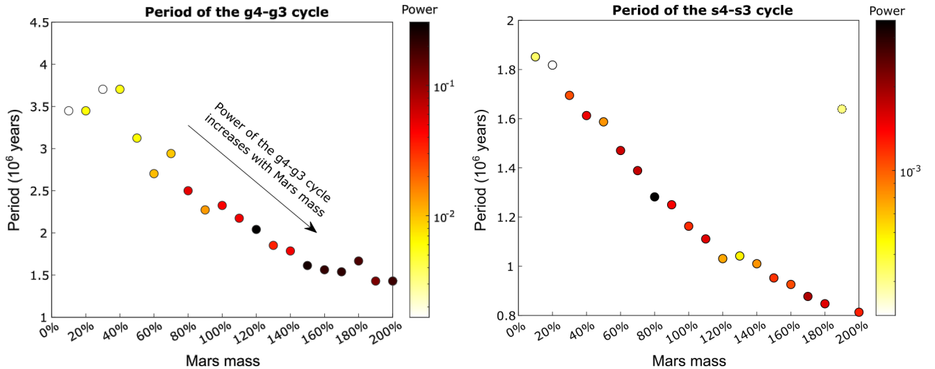
Figure 6. Left: The period and relative Fourier power (normalized to the strongest 400 kyr eccentricity cycle) of the g_4 - g_3 cycle as a function of the mass of Mars. Right: The period and relative Fourier power (normalized to the strongest 41 kyr primary obliquity cycle) of the s_4 - s_3 cycle as a function of the mass of Mars.
