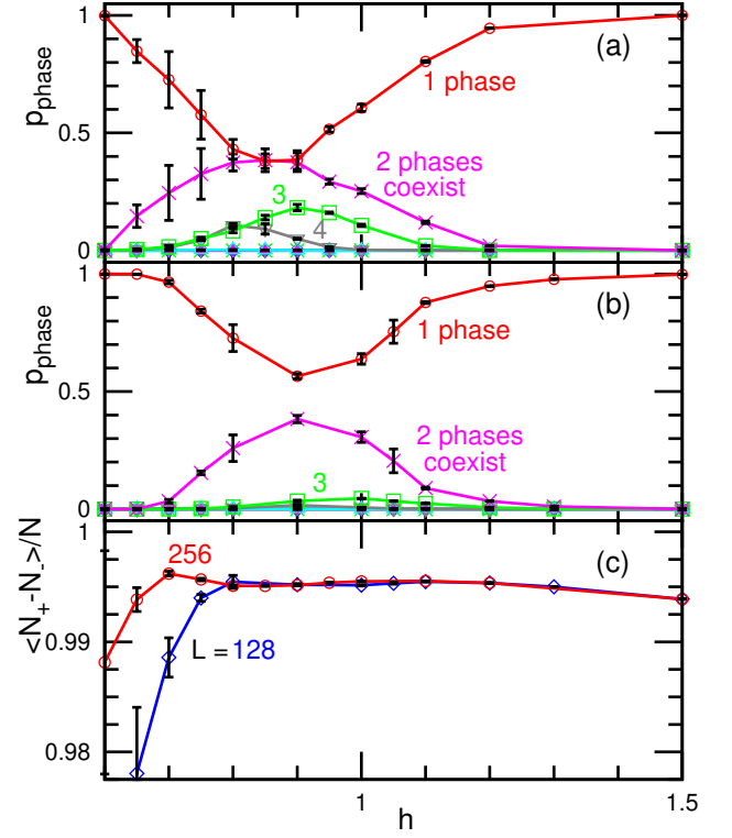
FIG. 14. Dependence on the flip energy h in the active Potts model with the cubic network [Fig. 10(b)]. (a)–(b) Phase ratios p_{\text{phase}} at (a) L = 256 and (b) L = 128 . (c) Mean number differences \langle N_+ - N_- \rangle / N between even- and odd-numbered states at L = 256 and 128, where N_+ = N_0 + N_2 + N_4 + N_6 and N_- = N_1 + N_3 + N_5 + N_7 .
