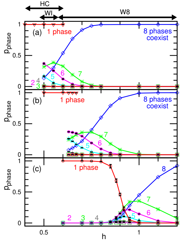
FIG. 9. Phase ratios p_{\text{phase}} as functions of h at (a) L = 512 , (b) L = 256 , and (c) L = 128 in the active Potts model with the square-antiprism network [Fig. 1(d)]. The red down-pointing triangles in (a) and (b) represent the ratio of the single-state dominant phase in the HC mode, whereas the ratios of multiple-state coexisting phases in the HC mode are omitted for clarity. The bidirectional arrows at the top of (a) represent the modes at L = 512 .
