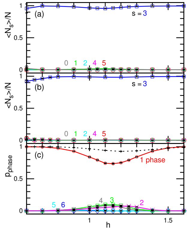
FIG. 12. Dependence on the flip energy h in the active Potts model with two four-state cycles [Fig. 10(a)]. (a)–(b) Mean numbers of states \langle N_s \rangle / N at (a) L = 256 and (b) L = 128 . (c) Phase ratios p_{\text{phase}} . The solid lines represent the data at L = 256 . The dashed line represents the ratio of the single-state dominant phase at L = 128 , whereas the ratios of multiple-state coexisting phases at L = 128 are omitted for clarity.
