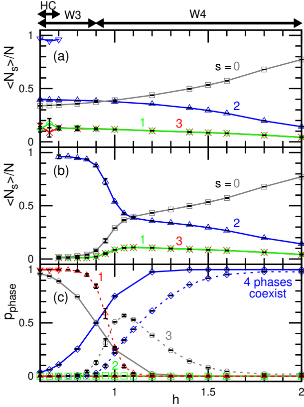
FIG. 4. Dependence on the flip energy h in the active Potts model with two three-state cycles [Fig. 1(a)]. (a)–(b) Mean number density \langle N_s \rangle / N at (a) L = 256 and (b) L = 128 . The blue down-pointing triangles in (a) represent s = 2 in the HC mode. (c) Time fractions p_{\text{phase}} of phases at L = 256 (solid lines) and L = 128 (dashed lines). The red down-pointing triangles represent the ratio of the single-state dominant phase in the HC mode at L = 256 , whereas the ratios of multiple-state coexisting phases in the HC mode are omitted for clarity. The bidirectional arrows at the top of (a) represent the ranges of three modes at L = 256 .
