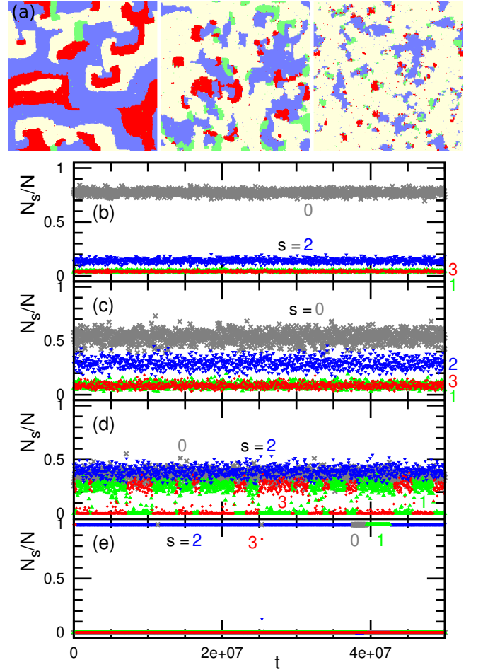
FIG. 3. Active Potts model with two three-state cycles [Fig. 1(a)] at L = 256 . (a) Snapshots at h = 0.7, 1.5, and 2 (from left to right). The light yellow, green, blue, and red sites (light to dark in grayscale) represent s = 0, 1, 2, and 3 , respectively. (b)–(e) Time development of the number of each state at (b) h = 2 , (c) h = 1.5 , and (d),(e) h = 0.7 . Two three-state spiral waves ( s = 0 \rightarrow 1 \rightarrow 2 \rightarrow 0 , and s = 3 instead of s = 1 ) spatially coexist (W4) at h \gtrsim 0.9 , and the s = 0 state becomes dominant at high h . The three-state spiral waves (W3) and homogeneous cycling (HC) are obtained at h = 0.7 , depending on the initial state. In W3, the two types of waves temporally coexist.
