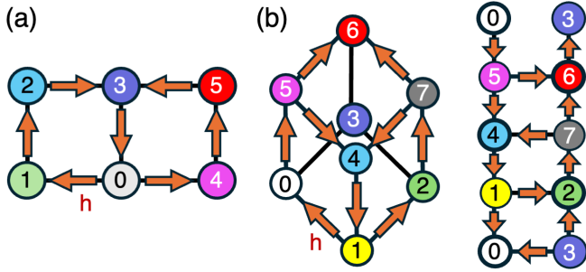
FIG. 10. Flip networks comprising multiple four-state cycles in active Potts models. The arrows for backward flips are omitted. (a) Six-state model with two four-state cycles. (b) Eight-state model with the cubic network. The unfolded graph is shown in the right panel.
