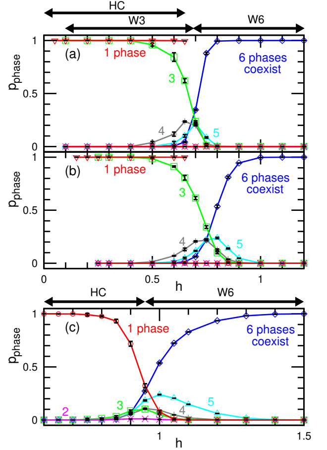
FIG. 7. Phase ratios p_{\text{phase}} as functions of h at (a) L = 512 , (b) L = 256 , and (c) L = 128 in the active Potts model with the octahedral network [Fig. 1(c)]. The red down-pointing triangles in (a) and (b) represent the ratio of the single-state dominant phase in the HC mode, whereas the ratios of multiple-state coexisting phases in the HC mode are omitted for clarity. The bidirectional arrows at the tops of (a) and (c) represent the modes at L = 512 and 128 , respectively.
