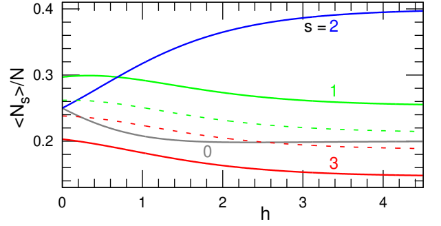
FIG. 2. Flip energy h dependence of the state densities N_s/N for the tetrahedron network [Fig. 1(b)]. The gray, green, blue, and red lines represent the data at s = 0, 1, 2 , and 3 , respectively. The solid and dashed lines for s = 1 and 3 represent the data at h_a = 1 and 0.2 , respectively.
