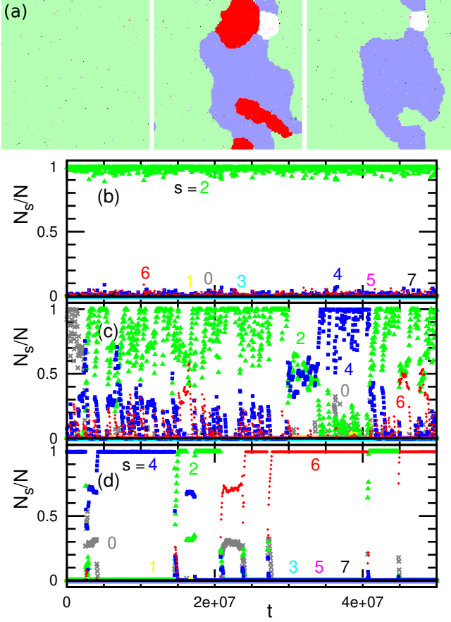
FIG. 13. Active Potts model with the cubic network [Fig. 10(b)] at L = 256 . (a) Sequential snapshots with a time interval of \Delta t = 40000 at h = 0.9 . (b)–(d) Time development of the number of each state at (b) h = 1.1 , (c) h = 0.9 , and (d) h = 0.7 .
