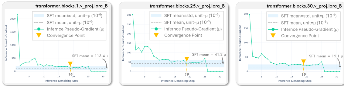
Figure 7: Gradient-based analysis of training–inference alignment on GPQA (sequence length 128, second diffusion block). The curve shows the RMS pseudo-gradients \tilde{G}_{t,B} across denoising steps, compared against the SFT gradient mean (dashed) and variance band (shaded). The convergence point (yellow ▼) occurs at the 19-th step, after which pseudo-gradients oscillate stably around the SFT mean. This alignment indicates that terminating at \sim 20 steps per block maintains fidelity comparable to full denoising while reducing computation, consistent with Table 2 (40.3 steps for two blocks).
