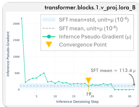
Figure 1: Gradient-based analysis of training-inference alignment on GPQA (seq. 128, 2nd block). Root mean square (RMS) pseudo-gradients \tilde{G}_{t,B} across steps are compared with the SFT gradient mean (dashed) and variance band (shaded). The convergence point (yellow \blacktriangledown ) occurs at step 19, after which pseudo-gradients stabilize near the SFT mean, indicating that \sim 20 steps per block preserve fidelity while reducing computation (Table 2, 40.3 steps for two blocks).
