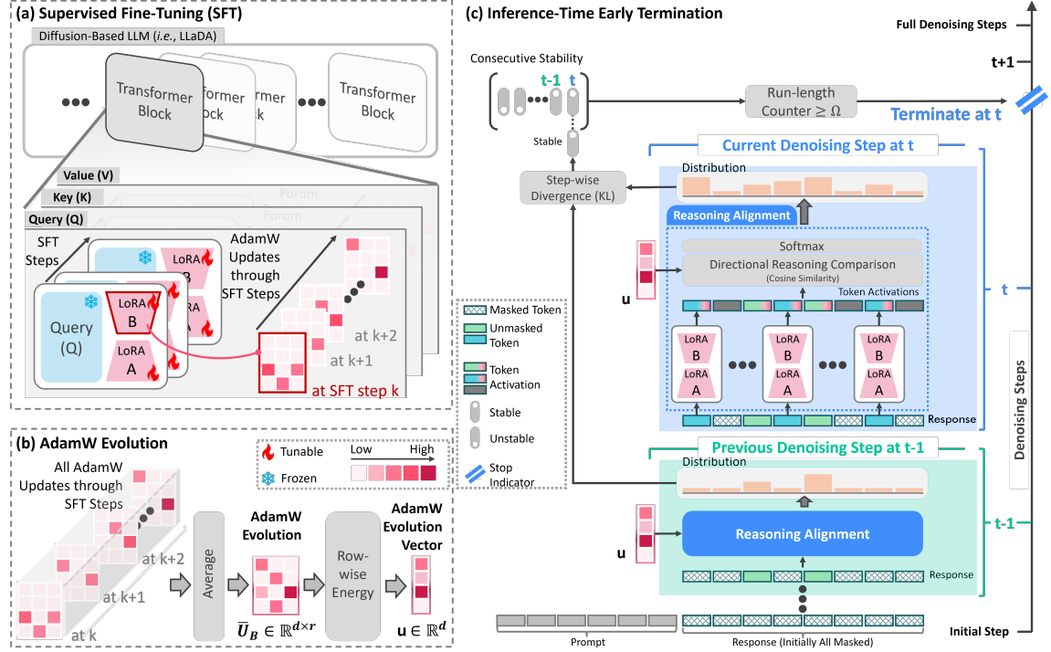
Figure 6: Overview of EDIT. (a) Supervised Fine-Tuning (SFT) : AdamW moment estimates track LoRA-B updates across steps, where some parameters consistently receive strong, directionally-aligned updates that encode reasoning patterns. (b) AdamW Evolution : Aggregating these updates yields a compact evolution vector \mathbf{u} that encodes reasoning-relevant parameter importance. (c) Inference-Time Early Termination : At inference, token activations are compared with the preserved evolution vector \mathbf{u} ; reasoning alignment is monitored via cosine similarity and KL divergence across steps. Once stability persists for consecutive steps, termination occurs before full denoising, reducing cost without loss of quality.
