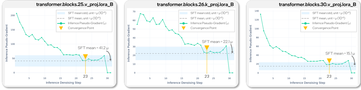
Figure 11: GSM8K (sequence length 128, second diffusion block). The convergence point (yellow ▼) occurs at the 23-rd step. Terminating at \sim 22 steps per block maintains fidelity comparable to full denoising while reducing computation, consistent with Table 2 (42.8 steps for two blocks).
