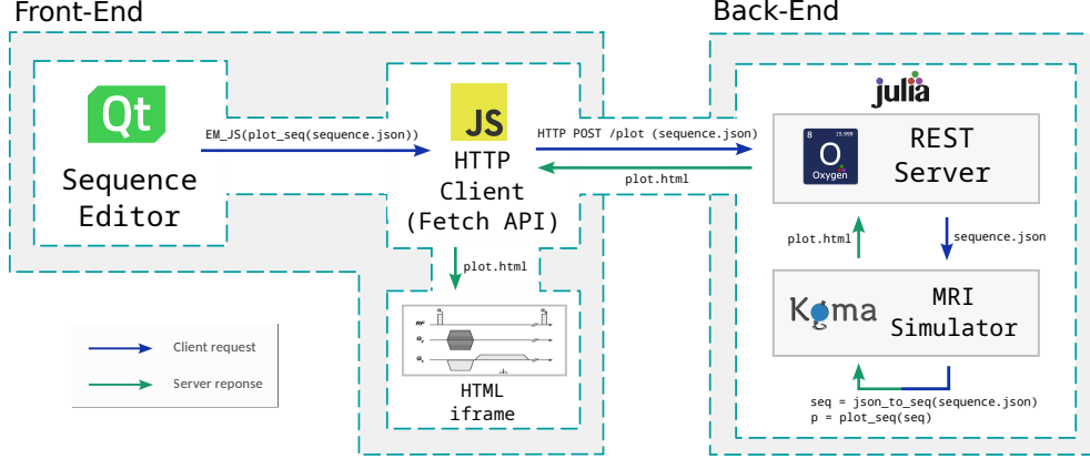
Fig. 1: General operation of the web application. The web browser is responsible for both rendering the front-end and acting as an HTTP client to communicate with the server. The HTTP server, in turn, provides a REST API to the web browser for accessing the back-end functionalities. Blue arrows represent client-side requests; green arrows represent server responses.
