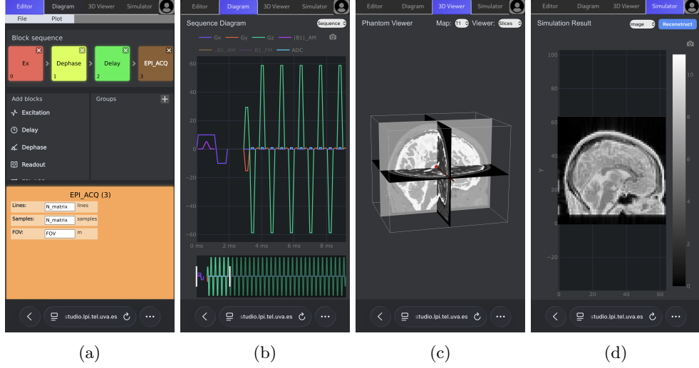
Fig. 3: Screenshots of the application running in a mobile browser. The example corresponds to the design and simulation of a GRE-EPI sequence. The slice-selection gradient applied along the x -axis produces a sagittal slice on the 3D brain phantom. (a) Sequence editor. (b) Sequence diagram visualizer. (c) 3D Phantom visualizer. (d) Simulation result.
