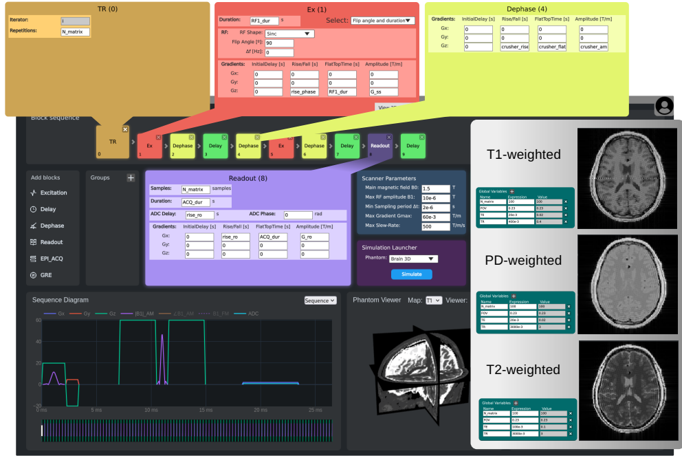
Fig. 6: Application GUI displaying the design of a spin-echo sequence. The sequence is organized into a block group that repeats every TR, along with RF, dephasing, crusher, readout, and delay blocks. Four block configuration panels are shown. The right panel presents the results of three simulation experiments in which TE and TR values were varied.
