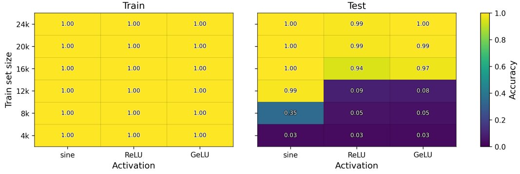
Figure 6: Train and test accuracy on modular addition for a 1-layer, 1-head decoder-only Transformer with FFN activations sine , ReLU , and GeLU .
