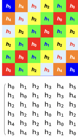
FIGURE 1. The approximation of h(|x - y|) and the reflected Toeplitz matrix (by symmetry with respect to the x axis).
