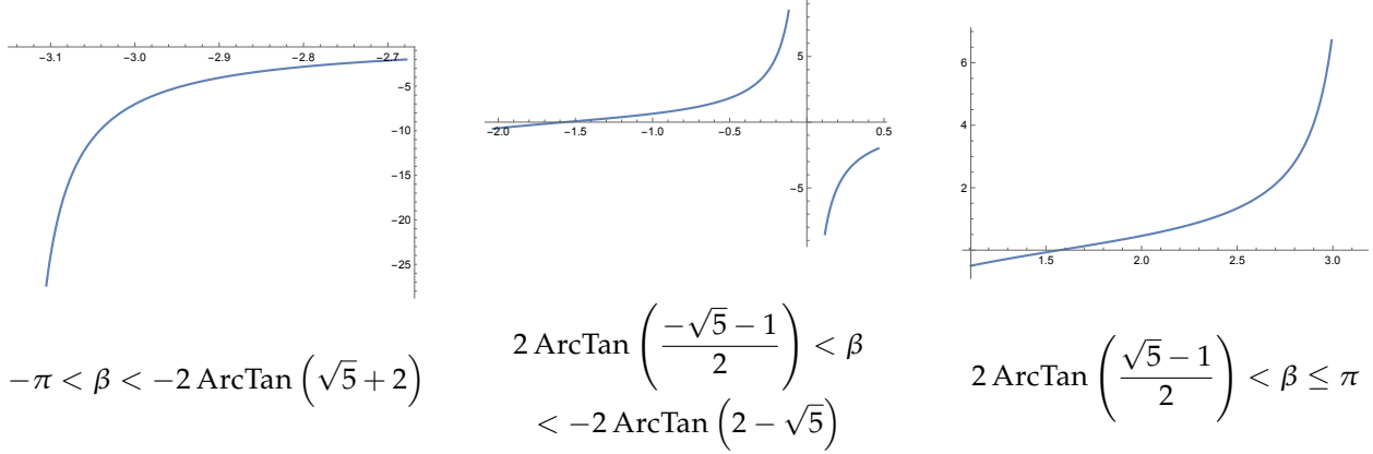
FIGURE 3. Three conditions on \beta illustrated with corresponding graphs.
