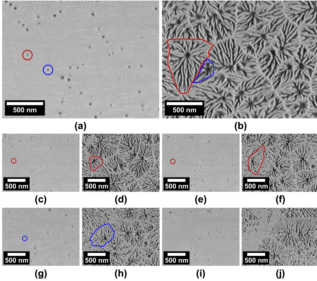
Figure 4: Reconstructed plan-view images as a function of depth, derived from serial-section FIB-SEM tomography of the 5-pair porous GaN-on-Si DBR etched at 5 V. Images are extracted positioned at a) onset of layer 1, b) layer 1, c) onset of layer 2, d) layer 2, e) onset of layer 3, f) layer 3, g) onset of layer 4, h) layer 4, i) onset of layer 5 and j) layer 5. 'Dislocation 1' is highlighted in red throughout, alongside 'dislocation 2' in blue.
