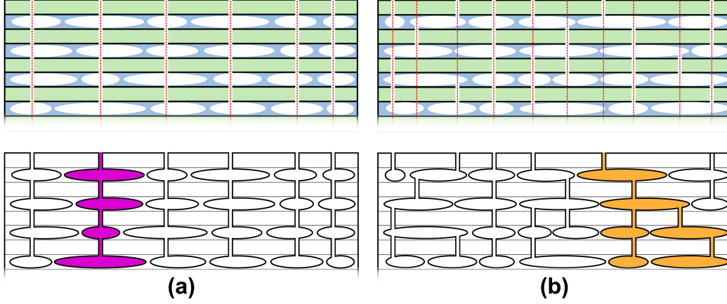
Figure 8: A schematic diagram of a) the conventional ‘kebab model’, as contrasted to b) the improved ‘cascade model’, for the proliferation of defect-driven etching. Red lines represent threading dislocation cores, and blue and green layers represent highly Si-doped layer and NID layers, respectively. Pore structures are highlighted below the schematics, with coloured structures demonstrating the differences between the models.
