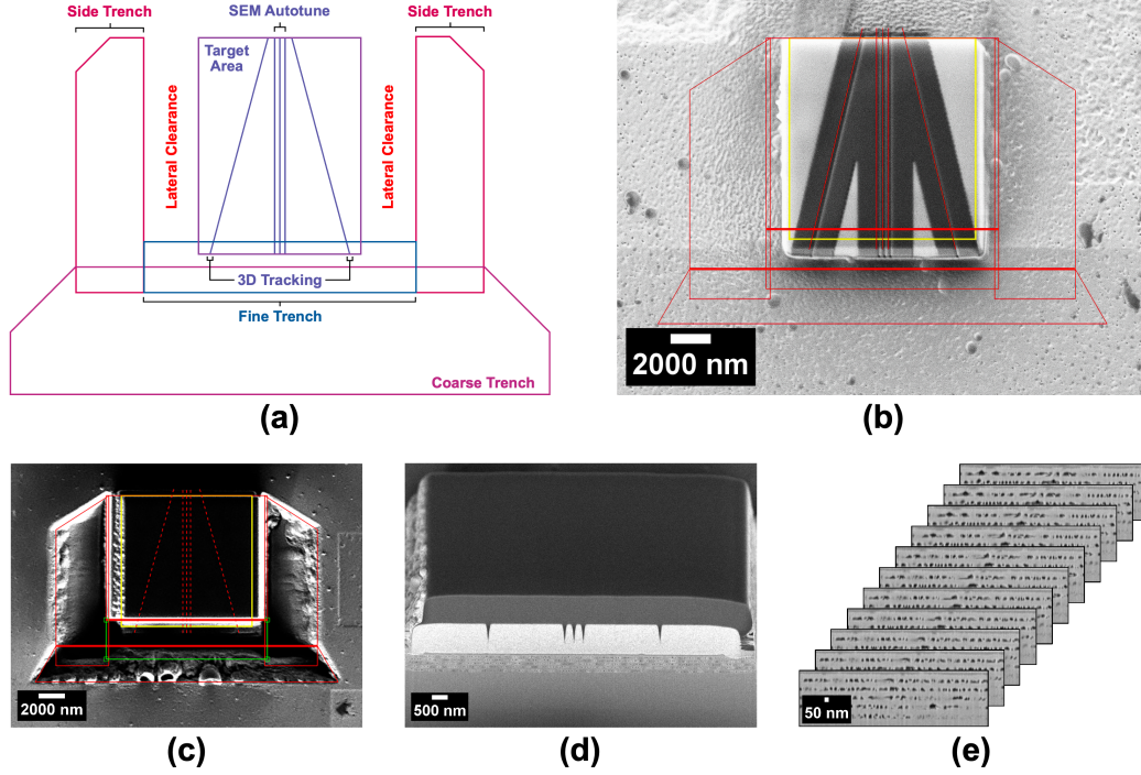
Figure 2: Outline of the serial-section FIB-SEM tomography procedure, showing a) a simplified schematic representation of the sample preparation step, b) the five lines hosted by the platinum and carbon deposited in the target area that are used for 3D tracking and SEM autotune of focus and stigmatism, c) the coarse, side, and fine trenches, milled after tracking and protection are prepared, d) cross-sectional SEM of the 5-pair porous GaN-on-Si DBR etched at 5 V with three parallel lines in the centre as well as two converging lines on either side, hosted by the protective platinum pad and backfilled with carbon and e) 11 serial-sections from the same DBR, where the sections are related to each other with an average 5.1 nm ion slicing thickness (Z dimension) for voxel dimensions of (2.0 \times 2.0 \times 5.1) nm owing to the use of 3D tracking and slice thickness interpolation.
