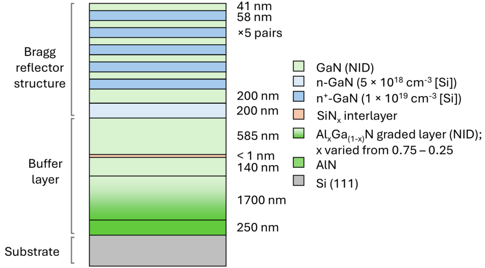
Figure 1: Simplified schematic of the as-grown epitaxial structure, prior to electrochemical porosification for the fabrication of 5-pair porous GaN-on-Si DBRs etched at 5 V, 8 V, and 10 V.
