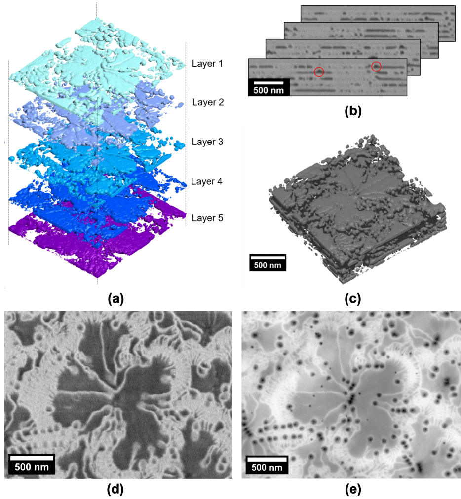
Figure 3: Serial-section FIB-SEM tomography example workflow with input serial-sections, output reconstructed plan-view images, and segmented tomograph 3D renders, shown for the 5-pair porous GaN-on-Si DBR etched at 10 V. a) Orthographic perspective 3D renders after tomograph segmentation with exaggerated inter-layer spacing, b) example serial-sections showing the porous region of interest, with two etched dislocation cores highlighted in red. Each of the scanning electron micrographs is captured with a 2.3 \text{ nm} \times 2.3 \text{ nm} X and Y pixel size. The sections are related to each other with an 8.8 \text{ nm} Z ion slicing thickness for tomographic voxel dimensions of (2.3 \times 2.3 \times 8.8) \text{ nm} , c) orthographic perspective 3D render of the porous layers with their real spacing, d) reconstructed plan-view of the first porous layer and e) sub-surface BSE-SEM micrograph of the first porous layer, depicting the target region of interest prior to correlative microscopy via serial-section tomography.
