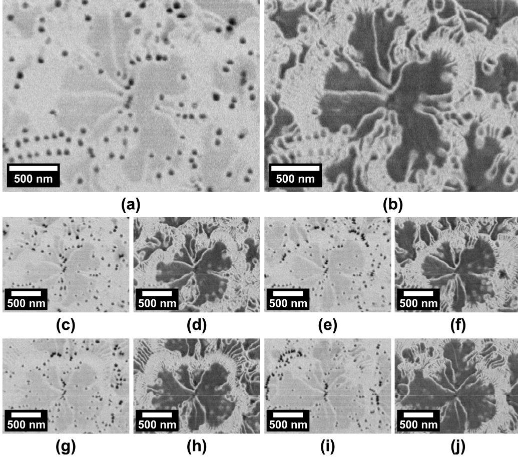
Figure 6: Reconstructed plan-view images as a function of depth, derived from serial-section FIB-SEM tomography of the 5-pair porous GaN-on-Si DBR etched at 10 V. Images are extracted positioned at a) onset of layer 1, b) layer 1, c) onset of layer 2, d) layer 2, e) onset of layer 3, f) layer 3, g) onset of layer 4, h) layer 4, i) onset of layer 5 and j) layer 5.
