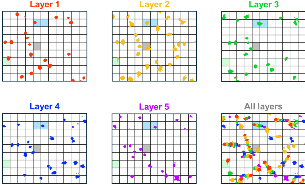
Figure 7: A series of images cropped and recoloured from the plan-view reconstructions of the 5-pair porous GaN-on-Si DBR etched at 8 V first shown in Figure 5 and derived from serial-section FIB-SEM tomography. All grid line separations are 100 nm. The onset of five porous layers is individually shown, with an additional sixth image that overlays all layers. Highlighted squares show regions containing threading dislocations with different activation behaviours during defect-driven electrochemical etching.
