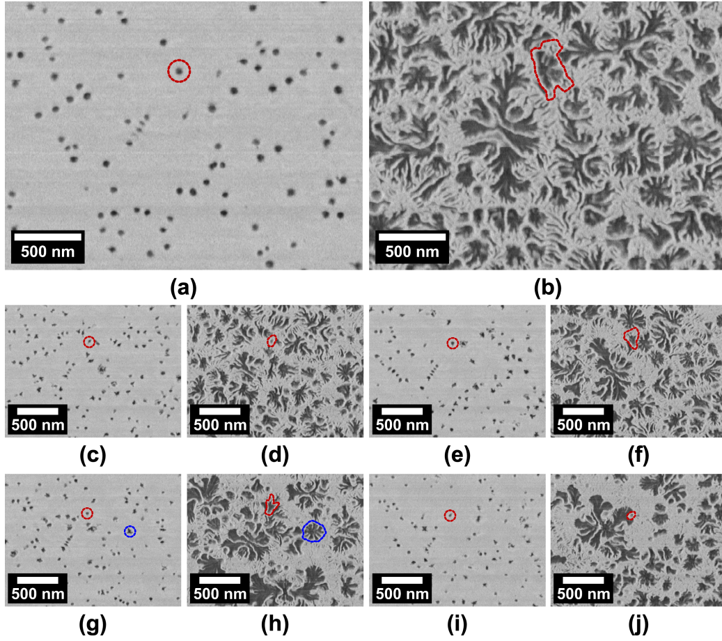
Figure 5: Reconstructed plan-view images as a function of depth, derived from serial-section FIB-SEM tomography of the 5-pair porous GaN-on-Si DBR etched at 8 V. Images are extracted positioned at a) onset of layer 1, b) layer 1, c) onset of layer 2, d) layer 2, e) onset of layer 3, f) layer 3, g) onset of layer 4, h) layer 4, i) onset of layer 5 and j) layer 5. 'Dislocation 3' is highlighted in red throughout, alongside 'dislocation 4' in blue.
