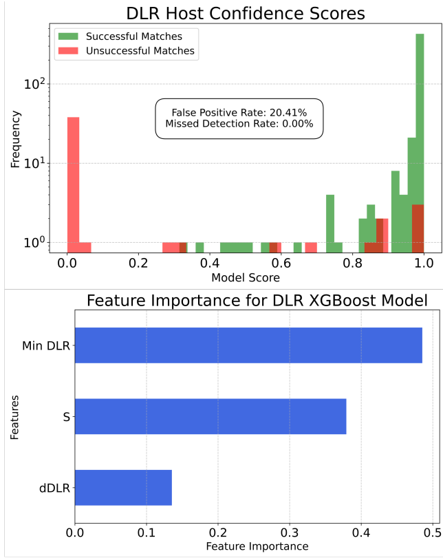
Figure 13. Score distribution of successful/unsuccessful matches by the DLR Confidence model.
