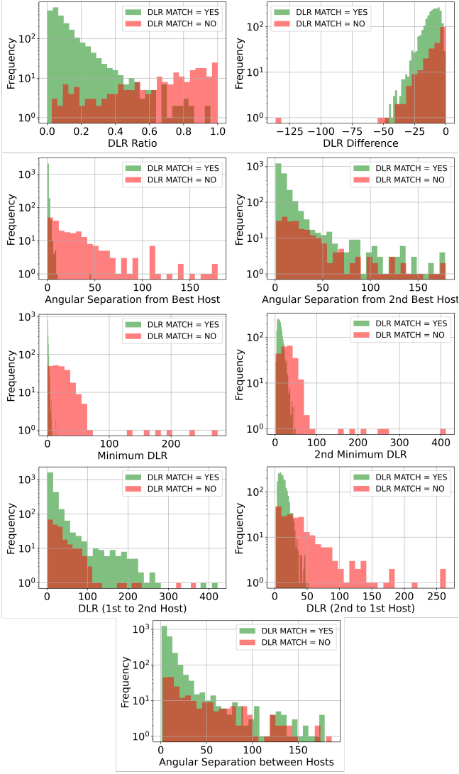
Figure 11. Feature distributions of successful/unsuccesful matches made by the DLR method.
