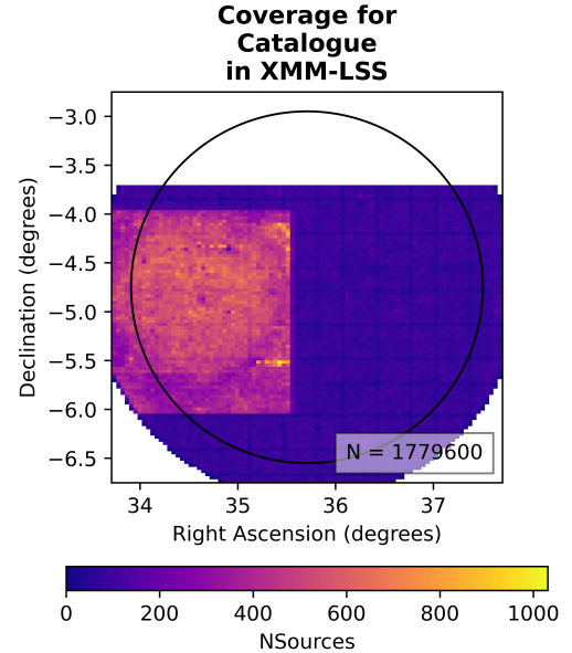
Figure 5. Primary catalogue coverage for XMM-LSS.
