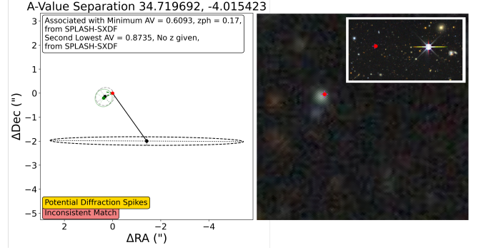
Figure 7. Diffraction spike source identified in an A-Value match. Note the large bright source along the axis of the diffraction spike (inset); a rotating variable (BD-04 376) with magnitude V = 10.05 .
