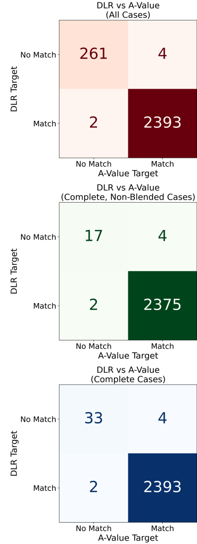
Figure 9. Confusion matrices comparing DLR and A-Value approaches for DES transients in XMM-LSS on catalogues where more extreme diffraction spikes have been culled.
