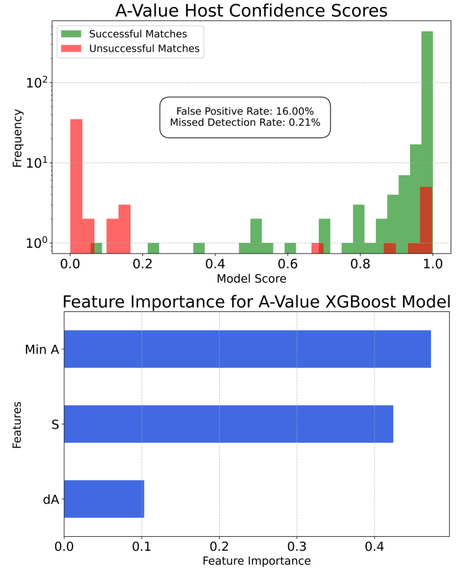
Figure 14. Score distribution of successful/unsuccessful matches by the A-Value Confidence model.
