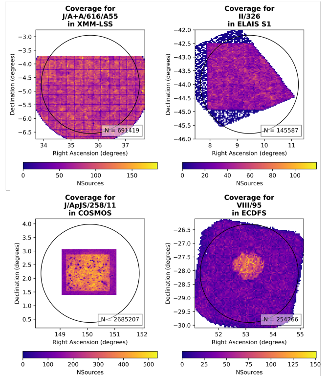
Figure 3. Example field coverage plots for a DDF catalogue in four of the fields. Lestrade performs a conesearch in the region surrounding the central pointing for each catalogue to identify subsets of data for each field. Top left: the CFHQSIR survey (S. Pipien et al. 2018) in XMM-LSS. Top right: Revised SWIRE Photometric Redshift Catalogue in ELAIS S1 (M. Rowan-Robinson et al. 2013). Bottom left: The COSMOS2020 Catalogue in COSMOS (J. R. Weaver et al. 2022). Bottom right: The Herschel Multi-tiered Extragalactic Survey catalogue (Hermes Team et al. 2017) in ECDFS.
