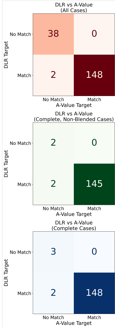
Figure 10. Confusion matrices comparing DLR and A-Value approaches for DES transients in ECDFS on catalogues where more extreme diffraction spikes have been culled.
