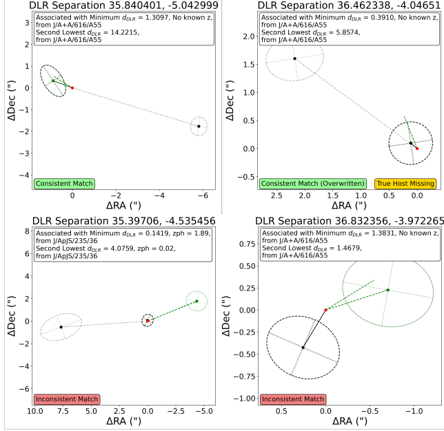
Figure 6. Lestrade visual aid plots for transient-host matching with the DES sample in XMM-LSS. The red marker denotes the transient location, with the DLR method’s identified best host (black) and second-best host (grey). A green dashed line links to the true host coordinates in the DES sample, and the morphology if the host exists within the catalogue. Top left: A consistent match by the DLR method to the host identified by DES. Top right: A consistent match by the DLR method. In this case, the match has been manually labelled as correct following visual inspection. Bottom left: An inconsistent match by the DLR method where the true host was neither identified as the best nor the second-best candidate host. Bottom right: An inconsistent match by the DLR method where the true host was identified as the second-best host.
