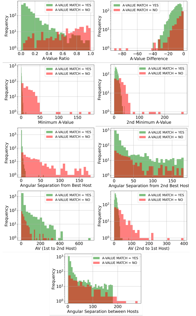
Figure 12. Feature distributions of successful/unsuccesful matches made by the A-Value method.
