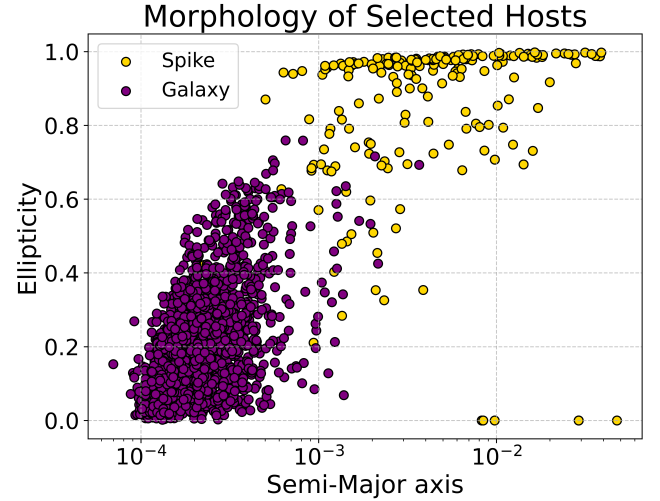
Figure 8. Diffraction spike sources identified in initial application of the DLR and A-Value methods.
