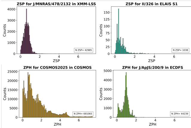
Figure 4. Example redshift coverage plots for a DDF catalogue in four of the fields. Top left: Spectroscopic redshifts in the XMM-SERVS survey (C. T. J. Chen et al. 2018) in XMM-LSS. Top right: Spectroscopic redshifts in the Revised SWIRE Photometric Redshift Catalogue in ELAIS S1 (M. Rowan-Robinson et al. 2013). Bottom left: Photometric redshifts in the COSMOS2025 Catalogue in COSMOS (M. Shuntov et al. 2025). Bottom right: Photometric redshifts in the ACS-GC catalogue (R. L. Griffith et al. 2012) in ECDFS.
