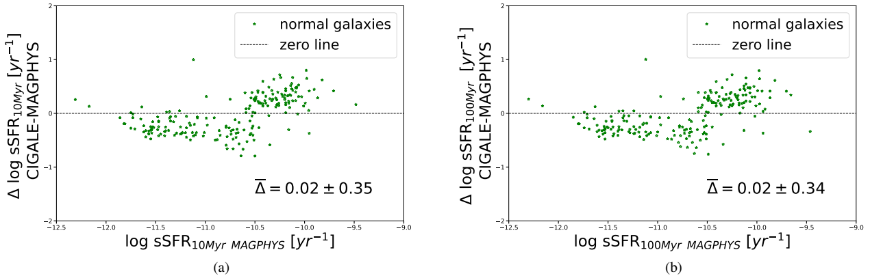
Figure 8. Differences ( \Delta ) between CIGALE and MAGPHYS estimates for normal galaxies (without AGN component) for sSFR averaged over the past (a) 10 and (b) 100 Myr (test B). The remark from Fig. 6 caption applies to these panels as well.
