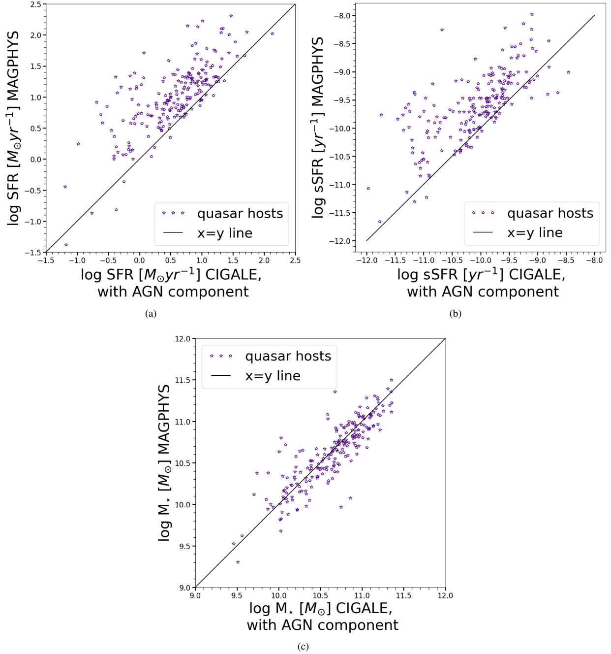
Figure 5. Results for comparison test A. Comparison between the GAMA archival data (MAGPHYS SED fitting results with no AGN component) and our CIGALE SED fitting results (including an AGN component) for (a) SFR, (b) sSFR, and (c) stellar mass for the sample of quasar host galaxies. The SFR and sSFR estimates differ significantly when an AGN contribution is included in the SED analysis, prompting us to derive anew the star formation property estimates for the quasar sample.
