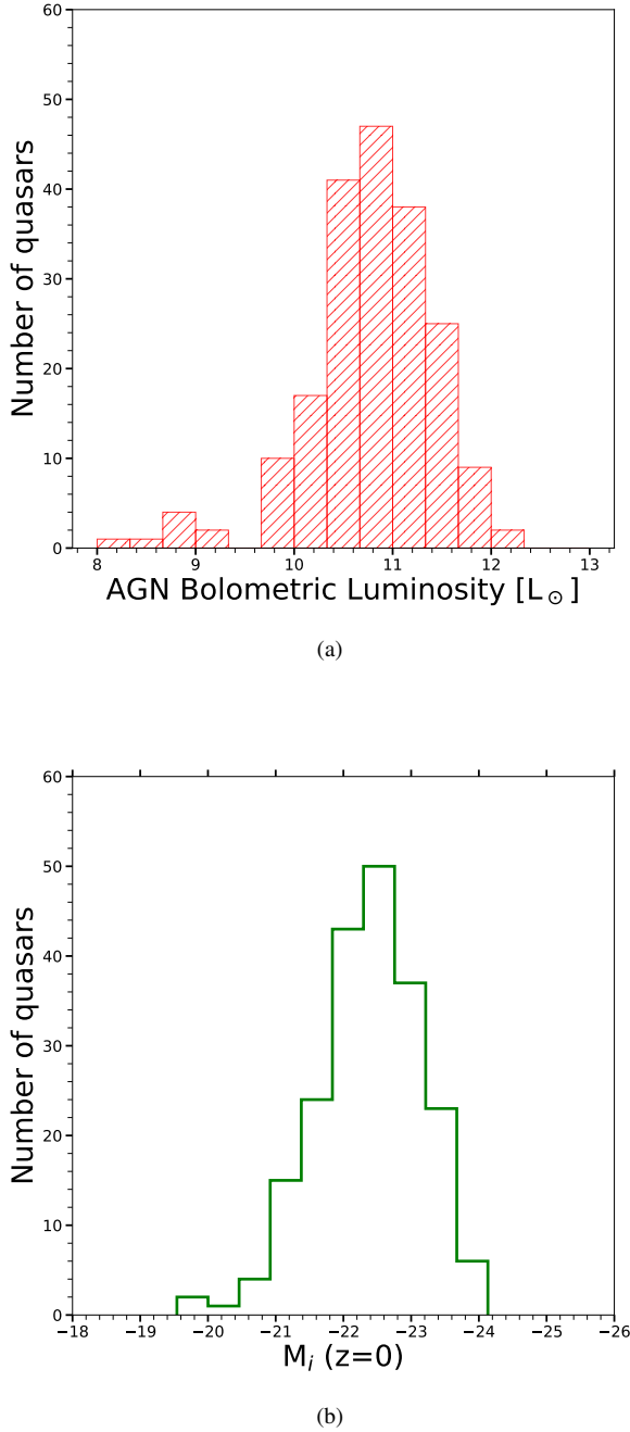
Figure 1. (a) Distribution of bolometric luminosities for quasars derived from CIGALE fits. This excludes 8 quasars (3.9 % of quasar sample) where CIGALE did not return a quasar luminosity. (b) Distribution of absolute SDSS i band magnitude ( k -corrected and extinction corrected based on GAMA survey data).
