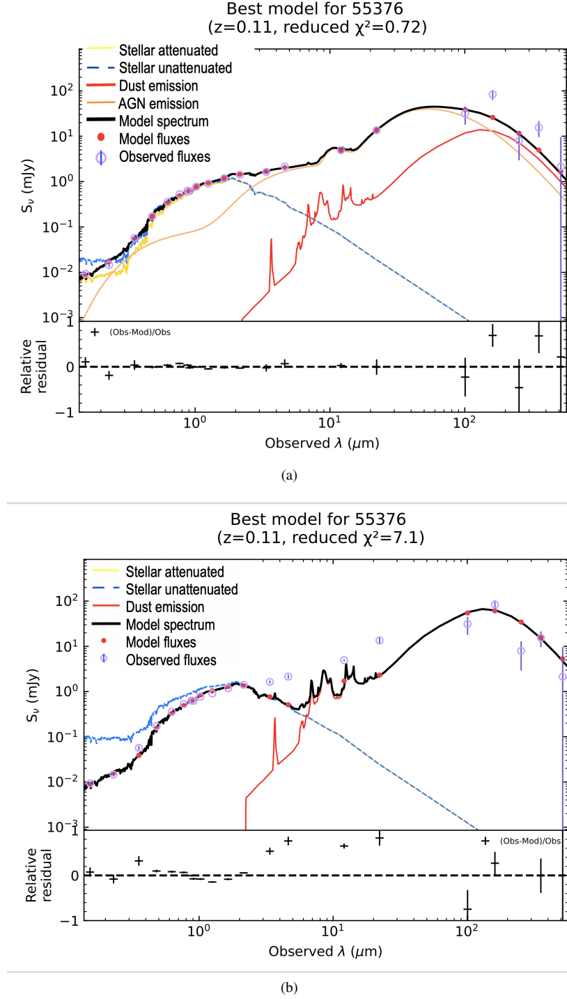
Figure 4. SED analysis result with CIGALE for one quasar in our sample. (a) Top panel shows the result which included AGN into consideration. AGN emission is represented by the solid orange line. (b) Bottom panel shows the best model without inclusion of the AGN module. Note the reduced \chi^2 value is much lower when AGN is considered, indicating a better fit.
