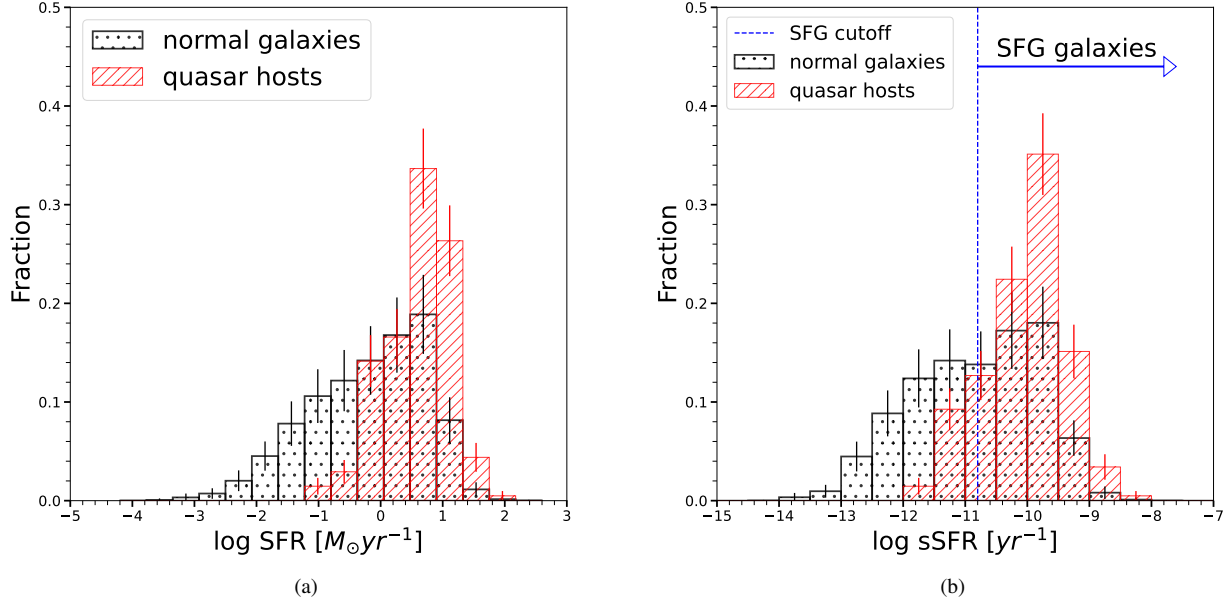
Figure 10. Histograms of SF properties with Poisson error bars: (a) SFR, (b) sSFR. Data for comparison galaxies are from GAMA archive, for quasar hosts from CIGALE SED fits. For quasar hosts, CIGALE SFR and sSFR estimates are corrected to MAGPHYS baseline and the error bar represents the Poisson error. For comparison galaxies, the plotted fraction in each bin is the average fraction from all 200 realizations, and the error bar represents the standard deviation. In each case, the distribution of values for quasar sample lies in the peak of the normal galaxy distribution. However, there are few quenched AGN hosts.
