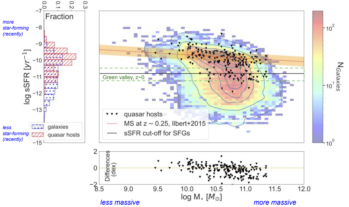
Figure 9. Top left Distribution of sSFR for quasars and comparison galaxies. Top right Stellar mass vs. sSFR for quasars (black triangles) and for comparison galaxies (contours and heatmap). The contour lines enclose 1/10/30/50/70/90 % of comparison galaxies. The heatmap colors go blue to red corresponding to low to high values of comparison galaxy population counts, as indicated by the colorbar. The main sequence (MS) relation for SFGs from Ilbert et al. (2015) is given here in orange dotted line, where the orange shaded area indicates the typical \sigma value of 0.3 dex (Katsianis et al. 2019). The black solid line indicates the cutoff between SFGs and passive galaxies, \log(\text{sSFR}) = -10.8 \text{ yr}^{-1} . The redshift value for the MS was adopted to be the median redshift of the SFGs in this sample of comparison galaxies, as discussed in Stone et al. (2023). For reference, the green valley transition region is marked per Salim (2014) with a green dashed box (for z \sim 0 ). Bottom Residuals which show the logarithmic difference (dex) between the quasar sSFR values and the sSFR values from the reference MS relation (orange dotted line), \Delta(\text{dex}) = \log_{10}(\text{sSFR}_{\text{quasar}}/\text{sSFR}_{\text{ref}}) . The plotted sSFR and stellar mass data for comparison galaxies come from the GAMA survey MAGPHYS SED analysis, while for quasar hosts from CIGALE SED fits. For quasar hosts, the sSFR values from CIGALE were corrected to MAGPHYS baseline.
