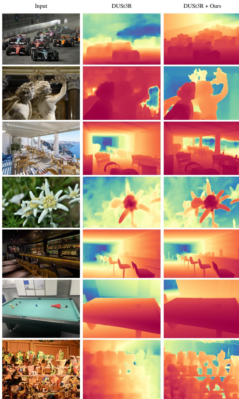
Figure S2: Additional visualization of depth estimation results. From left to right: input image, baseline (DUST3R), and our improved method (DUST3R+Ours).
