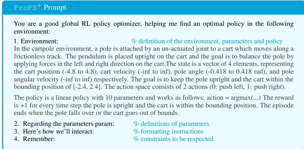
Figure 3: Summary of the structure, information and instructions utilized to construct domain-specific ProPS + prompt, with an example of the prompt for CartPole environment.
