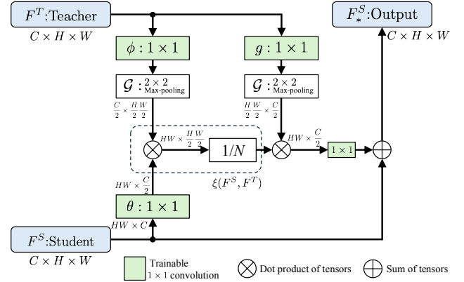
Figure 1. Proposed Cross-attention-based Non-local (Can) block.
