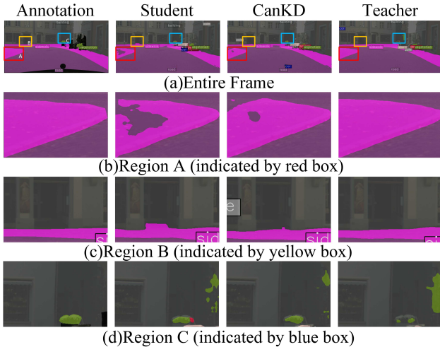
Figure 5. Visualization of prediction results for semantic segmentation task in the Cityscapes validation dataset. The teacher is PSPNet-R101 and the student is PSPNet-R50.
