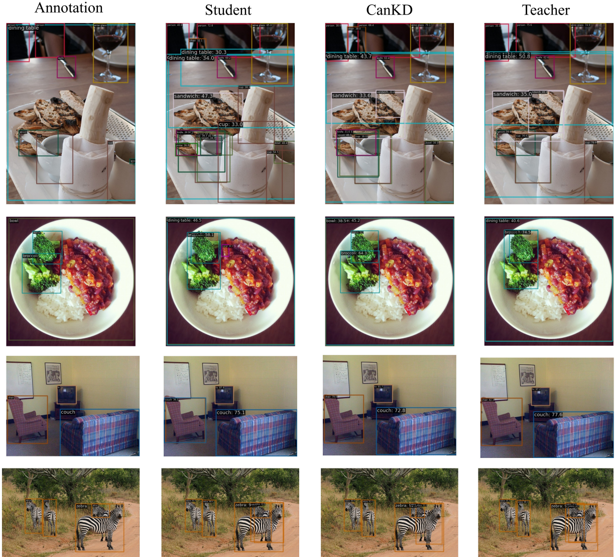
Figure 5. Additional sampling from RepPoints-R50, distilled RepPoints-R50 with CanKD and RepPoints-X101. All of these figures are selected from COCO val 2017 dataset.
