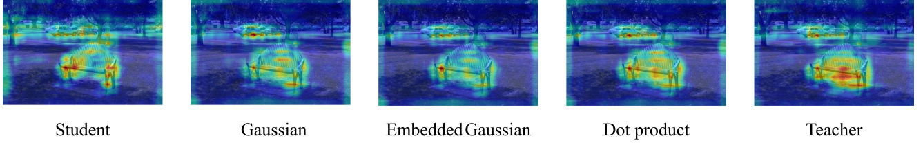
Figure 3. Visualization heatmaps for different affinity functions. We use RepPoints-X101 [49] as the teacher and RepPoints-R50 as the student. These heatmaps are generated from P6 in the FPN layers
