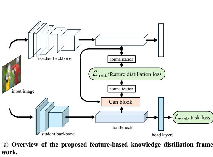
Figure 2. Proposed feature-based knowledge distillation using the Cross-Attention-based Non-local operation
