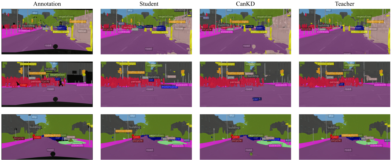
Figure 4. Additional sampling from PSPNet-R18[25], distilled PSPNet-R18 with CanKD and PSPNet-R101. All of these figures are selected from Cityscapes val dataset.
