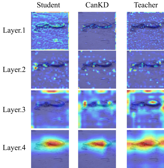
Figure 7. Heatmaps from ResNet-18, distilled ResNet-18 with CanKD and ResNet-32. These figures are generated from Layer.1 to Layer.4 in backbone.
