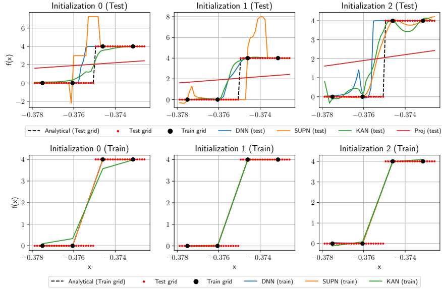
FIG. SM4.7. Plot of zoomed in discontinuity at x = -0.375 for the step function target. The network approximations shown are drawn from the largest width/depth or M/N models shown in Figures SM4.1 to SM4.3 , i.e., along the diagonal, for three different model initializations.
