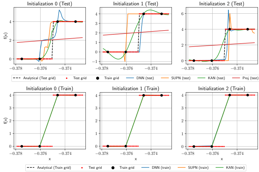
FIG. SM4.6. Plot of zoomed in discontinuity at x = -0.375 for the step function target. The network approximations shown are drawn from the 3rd largest width/depth or M/N models shown in Figures SM4.1 to SM4.3 , i.e., along the diagonal, for three different model initializations.
