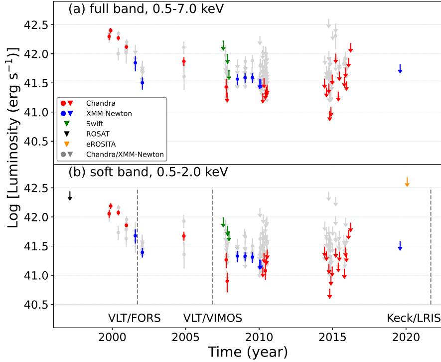
Figure S5: Month-bin X-ray light curves of XID 935. (a) Light curve in the rest-frame 0.5–7.0 keV band (full band, containing 768.9 \pm 43.3 and 905.0 \pm 84.0 Chandra and XMM-Newton net counts, respectively). (b) Light curve in the rest-frame 0.5–2.0 keV band (soft band, containing 595.9 \pm 28.5 and 680.7 \pm 62.6 Chandra and XMM-Newton net counts, respectively). Red, dark blue, green, black, and orange data are from Chandra, XMM-Newton, Swift, ROSAT, and eROSITA, respectively. Grey data represent individual observations of Chandra and XMM-Newton. Arrows indicate 90%-confidence-level upper limits. Dashed lines denote the observation times of optical spectra.
