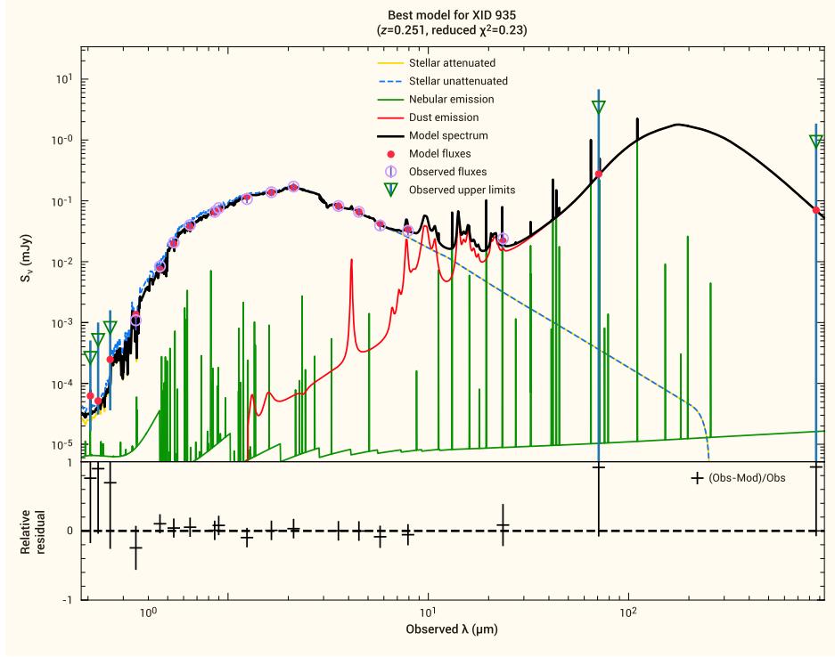
Figure 2: SED fitting result for XID 935 using CIGALE. The stellar mass M_{\star} = (3.1 \pm 0.6) \times 10^{10} M_{\odot} and the star-formation rate \text{SFR} < 1.3 \times 10^{-2} M_{\odot}/\text{year} (90% confidence level) were obtained. Note that an AGN component is not required in the fitting.
