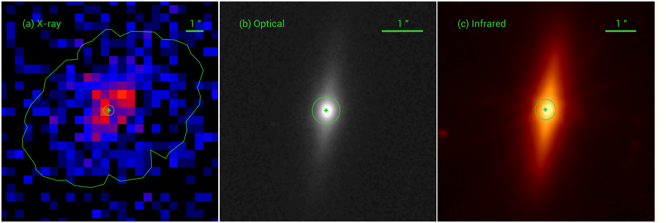
Figure 4: Multi-wavelength images of XID 935. (a) 7 Ms CDF-S image in the observed 0.5–7.0 keV band, with total net counts of 768.9 \pm 43.3 . The green polygon is the 90% encircled-energy fraction region, centered at the source position (green plus; with a 1\text{-}\sigma positional accuracy of 0.3 arcsec, indicated by the green circle, corresponding to 0.99 kpc at z = 0.251 ). (b) GOODS z band image. (c) JWST-NIRCam F227W band image. The green pluses and circles in Panels (b) and (c) are the same as that in Panel (a). The position of XID 935 is consistent with the nucleus of its host galaxy.
