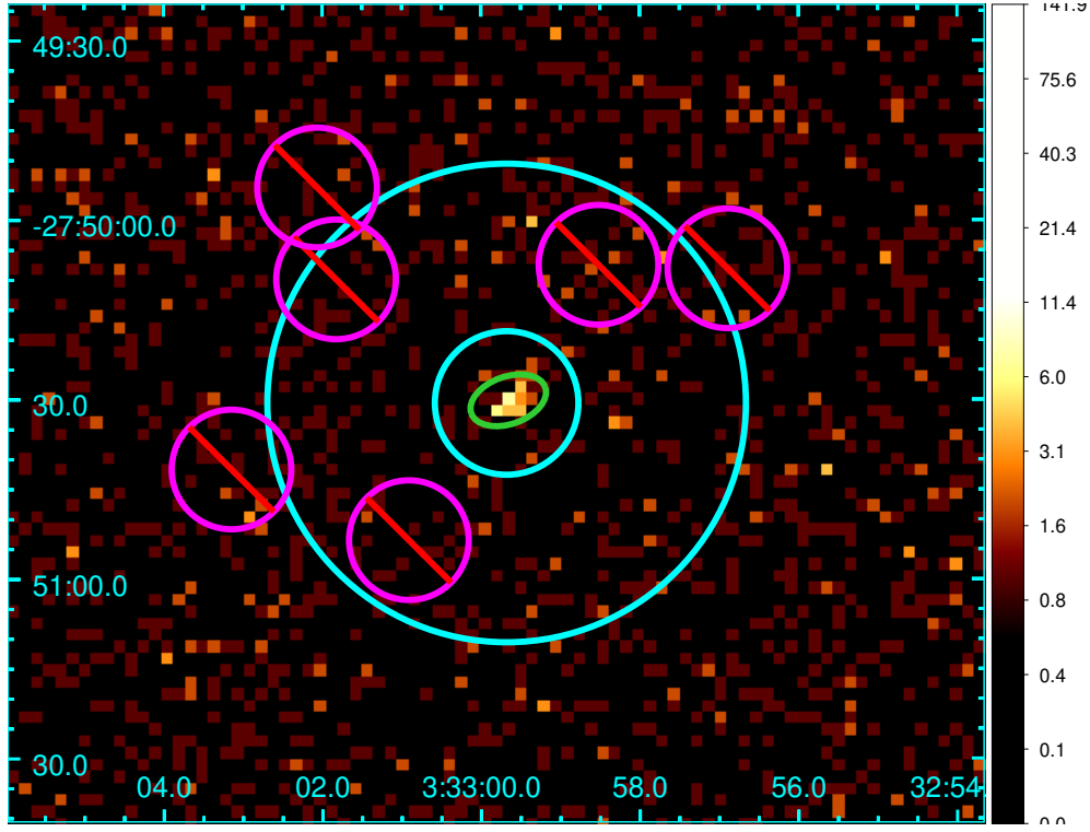
Figure S2: Extraction region for XID 935 in the CDF-S. The green ellipse is the source region. The cyan annulus is the background region, with 6 adjacent sources masked using magenta circles.
