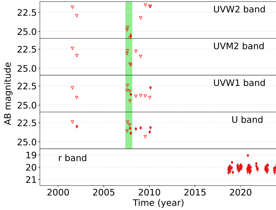
Figure S1: Optical/UV light curves of XID 935. From top to bottom, the bands are rest-frame UVW2, UVM2, UVW1, U, and r bands, respectively. For UVW2, UVM2, UVW1, and U bands, the Swift/UVOT data are green-shaded; outside the shaded region are the XMM-Newton/OM data. The r-band data are from the ZTF. Error bars correspond to 1\text{-}\sigma uncertainties. Triangles are 90%-confidence-level upper limits.
