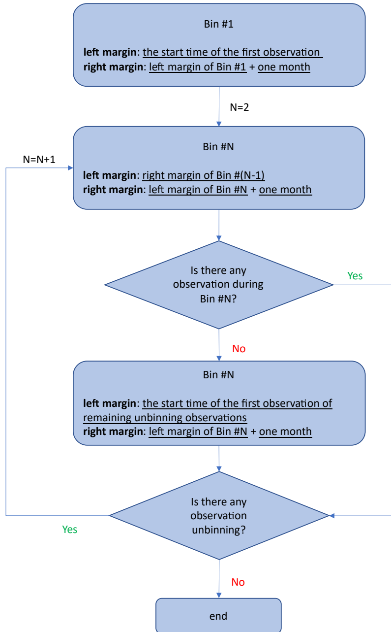
Figure S4: Month-bin flow diagram.
