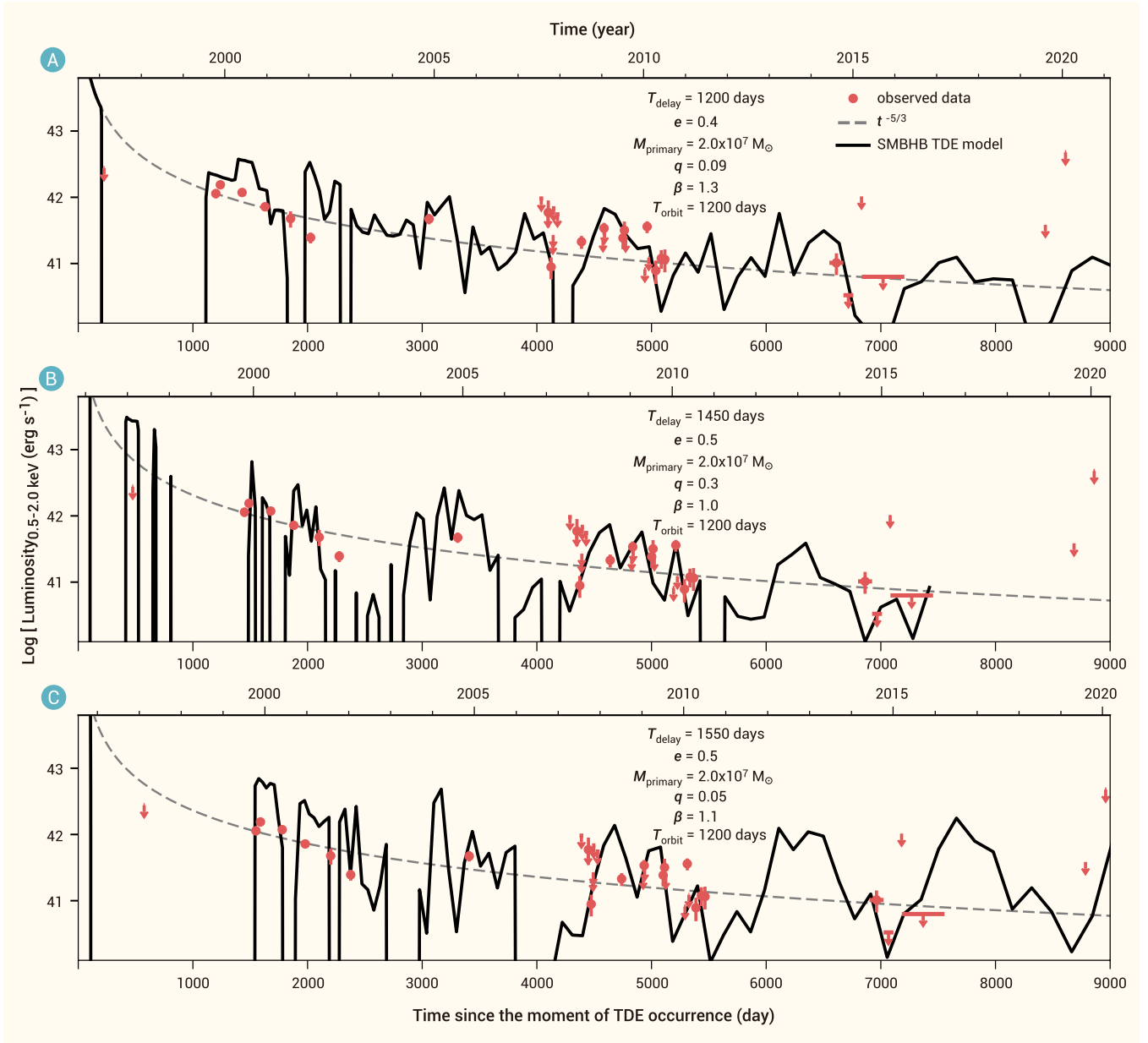
Figure 6: SMBHB TDE model fits for XID 935. In each panel, the rest-frame 0.5–2.0 keV light curve is shown with red symbols. Error bars correspond to 1- \sigma uncertainties. Downward arrows are 90%-confidence-level upper limits. The dashed grey curve represents the canonical t^{-5/3} decay law. The gapped black solid curve is the SMBHB TDE model fitting result, with the following model parameters annotated: T_{\text{delay}} , the time delay between the first observed detection data point and the moment of TDE occurrence; e , the ellipticity of SMBHB orbit; M_{\text{primary}} , the mass of the primary black hole; q , the mass ratio between the secondary and primary SMBHs; \beta , the penetration factor; T_{\text{orbit}} , the orbital period of SMBHB. (A) T_{\text{delay}} = 1200 days, e = 0.4 , q = 0.09 , \beta = 1.3 . (B) T_{\text{delay}} = 1450 days, e = 0.5 , q = 0.3 , \beta = 1.0 . (C) T_{\text{delay}} = 1550 days, e = 0.5 , q = 0.05 , \beta = 1.1 . (A),(B), and (C) share identical values of M_{\text{primary}} = 2.0 \times 10^7 M_{\odot} and T_{\text{orbit}} = 1200 days.
