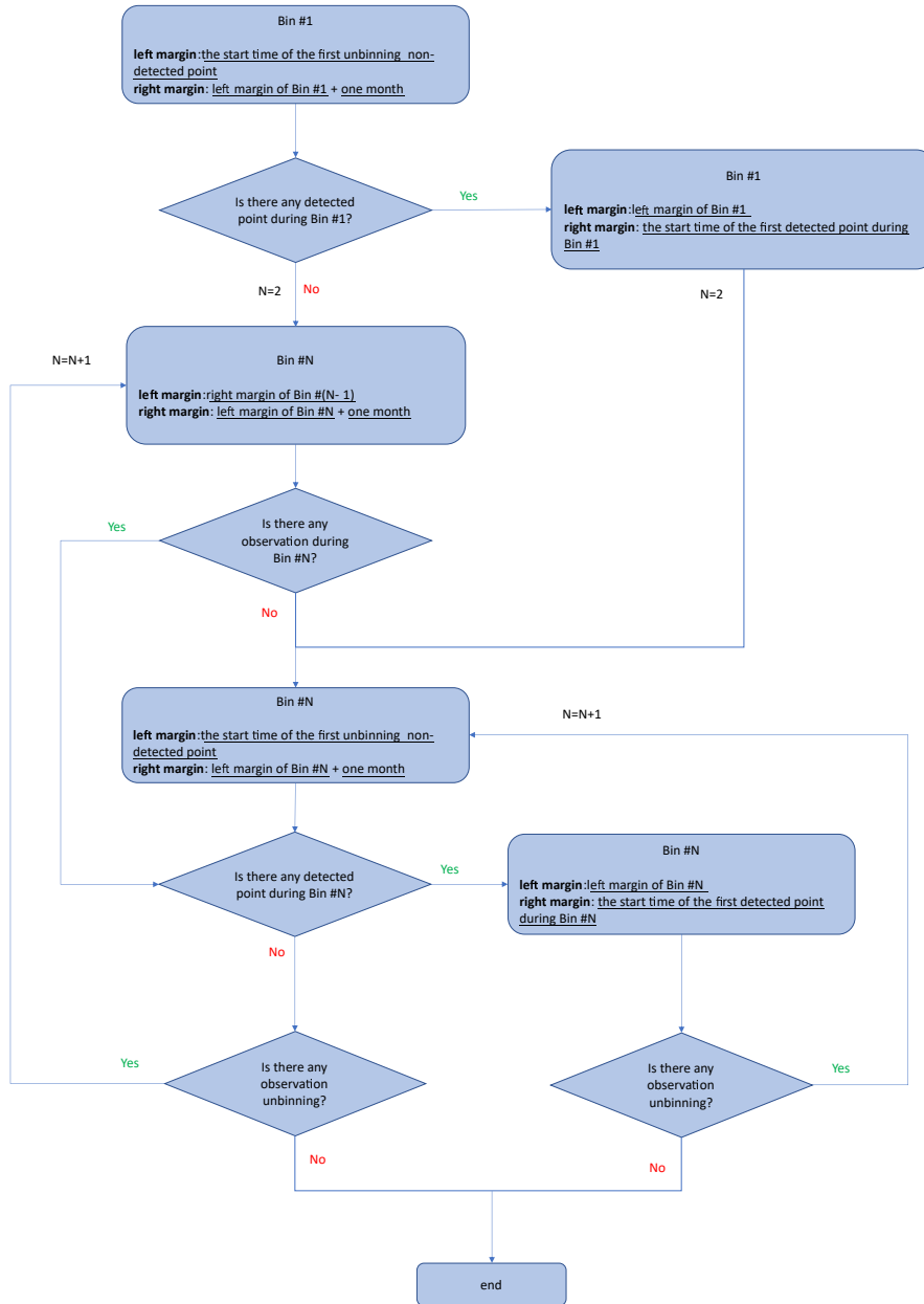
Figure S6: Adaptive-bin flow diagram.
