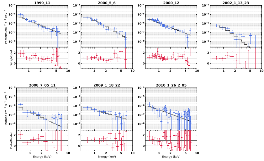
Figure S7: X-ray spectra of XID 935. Each panel displays the fitted spectrum and data-to-model ratio for time bins with net counts exceeding 60.
