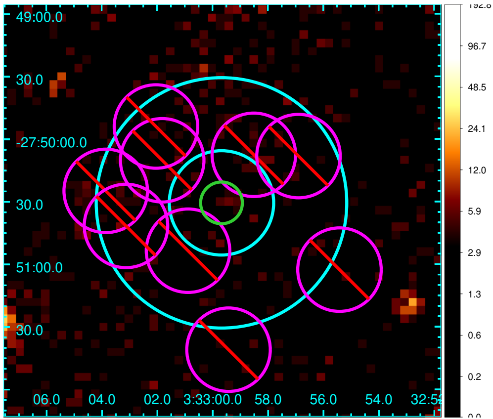
Figure S3: Extraction region for XID 935 in the XMM-CDFS. The green circle is the source region, and the cyan annulus is the background region, with 9 adjacent sources masked using magenta circles.
