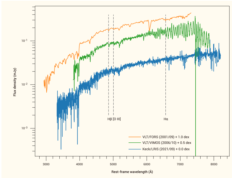
Figure 3: Optical spectra of XID 935. The spectral analysis of the Keck/LRIS spectrum (blue), performed on 8 September 2021, shows that the host galaxy of XID 935 has no significant AGN characteristics. The flux upper limit of the [O III] emission line is 10^{-16.68} erg s -1 cm -2 and the stellar velocity dispersion is 138 \pm 31 km/s. The VLT/VIMOS spectrum (green) was obtained on 30 October 2006 (Balestra et al. 2010). The VLT/FORS spectrum (orange) was observed on 18-20 September 2001 (Szokoly et al. 2004).
