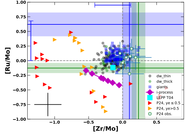
Fig. 3. [Ru/Mo] for the stellar sample presented in this work, shown with respect to [Zr/Mo]. For comparison, the metal-poor stars from Honda et al. (2007); Hansen et al. (2012, 2014); Aoki et al. (2017) and Psaltis et al. (2024) are shown as white squares with green contours. The ratios from the s -process GCE simulations by Bisterzo et al. (2014) (green line and error range) and from the r-II star CS 22892-052 (Sneden et al. 2003) (green line and error range) are included as references. The production range derived from a collection of r-II stars is indicated by the blue horizontal and vertical error bars for [Zr/Mo] and [Ru/Mo], respectively (see the text for details). We also report the LEPP prediction by Travaglio et al. (2004) (large cyan square), the ratios from different neutrino-driven ejecta conditions in Psaltis et al. (2024) with Y_e > 0.5 (orange triangles, \nu p -process) and with Y_e < 0.5 (red squares, weak r -process), along with i -process predictions for mild neutron exposures, characterized by production peaking in the Zr-Ru region, and no relevant production at the Ba peak (magenta-lined squares; see text for more details). The typical observation error for our stars is given in the lower left corner of the plot (black error bar).
