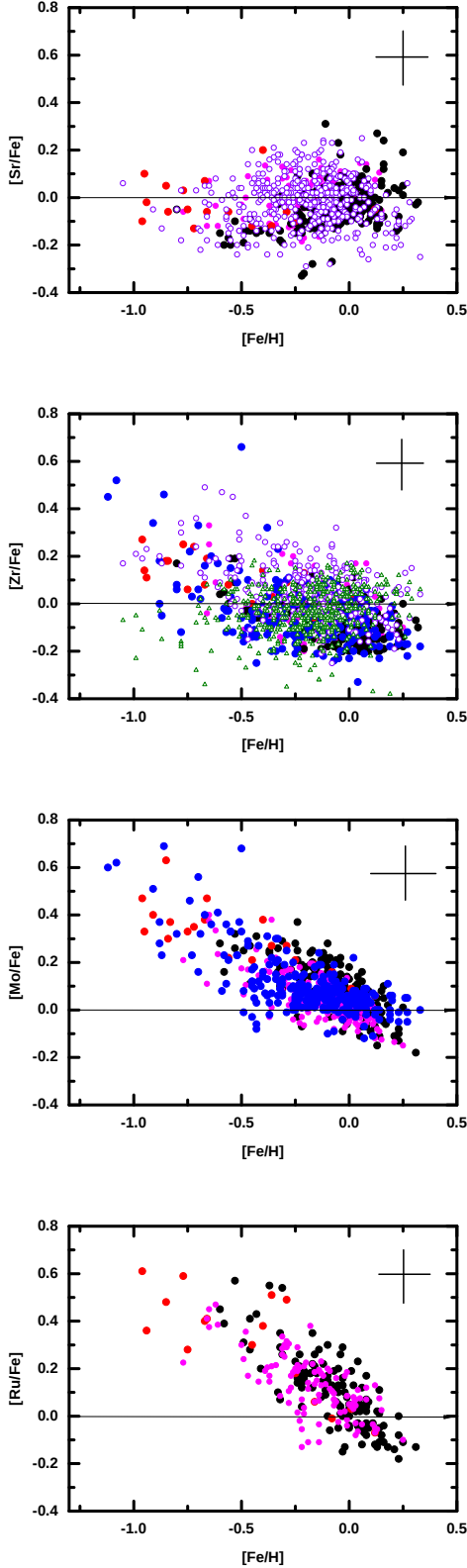
Fig. 2. [Sr/Fe], [Zr/Fe], [Mo/Fe], and [Ru/Fe] with respect to [Fe/H] given for the giant stars in our sample (magenta points), the dwarf stars by Mishenina et al. (2019b,a, 2013) (thin disk stars as black points, and thick disk stars as red points). The data from Forsberg et al. (2019) (Zr) and Forsberg et al. (2022) (Mo) are shown as blue points, while those from Tautvaišienė et al. (2021) – Sr and Zr I – are shown as open purple circles, and Zr II as open green triangles.
