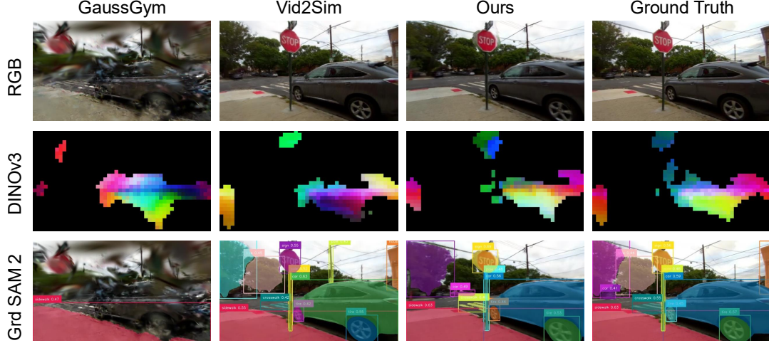
Figure 6. Photorealism and semantic consistency for sensor simulation. We show extrapolated view synthesis results from different frameworks, and their inference results from the DINOv3 [85] and Grounded SAM 2 models [86]. The DINOv3 visualization shows the first three PCA components on each patch feature. The foreground is filtered by a small linear classifier on DINOv3 features.
