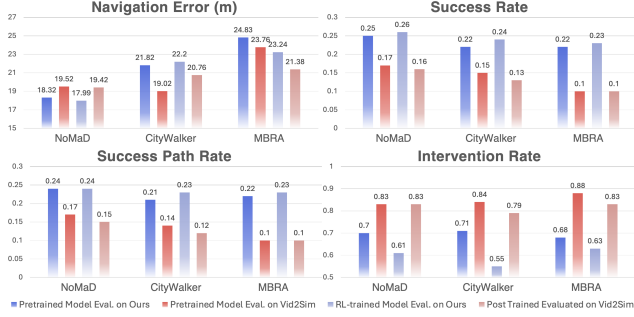
Figure 7. Geometrically grounded environment for evaluation. We compare evaluation results of the same models on different environments. Results are evaluated on the WANDERLAND test split. Comparison should be made between different evaluation environments (different colors) for same models.
