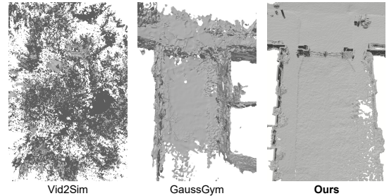
Figure 5. Mesh qualitative comparison. All results are reconstructed from the same data in the WANDERLAND dataset. Our framework extracts complete and smooth mesh.
