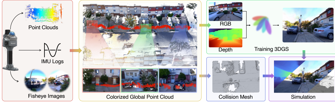
Figure 4. Data Processing Pipeline. Our pipeline begins with multi-sensor capture using the MetaCam device in real-world urban spaces. MetaCam Studio processes the raw data via LIV-SLAM to produce a colorized, globally consistent metric point cloud and accurate camera poses. We then initialize 3D Gaussians from the metric point cloud and render per-view depth maps from this initialization. The 3DGS model is optimized with both photometric and depth losses. In parallel, we extract a reliable collision mesh from the same global point cloud. Finally, we integrate the trained 3DGS model and the collision mesh into a single Universal Scene Description (USD) scene, which can be directly loaded into Isaac Sim for training and evaluating navigation policies
