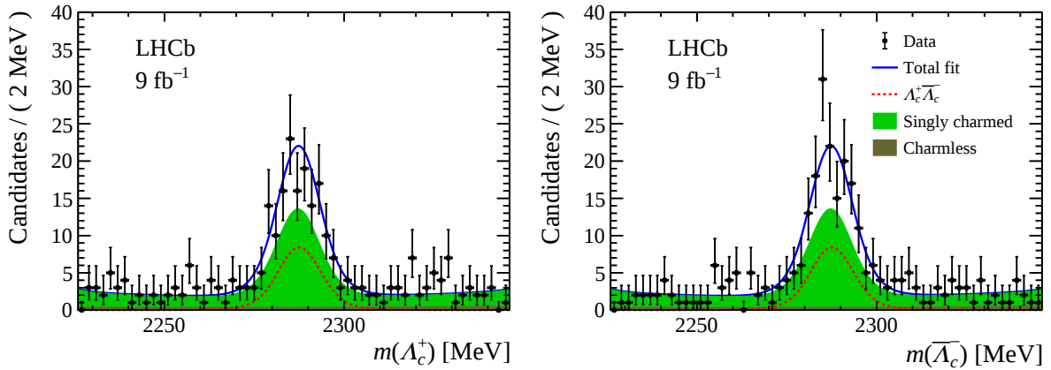
Figure 3: Distributions of the (left) \Lambda_c^+ and (right) \bar{\Lambda}_c^- mass for the signal sample. Also shown is the projection of the two-dimensional fit (solid blue line) integrated over all m(\Lambda_c^+ \bar{\Lambda}_c^-) bins, along with the contributions from doubly charmed (dashed red), singly charmed (filled green), and charmless (filled brown) decays.
