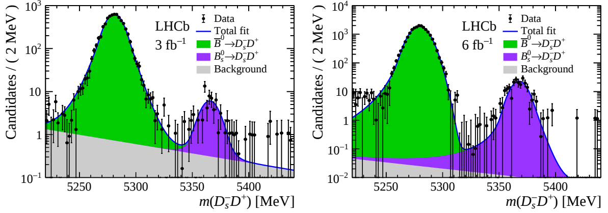
Figure 4: Mass distribution of the D_s^- D^+ system, with singly charmed and charmless backgrounds subtracted, shown for (left) Run 1 and (right) Run 2 data-taking periods. The fit projection (solid blue line) is shown together with the signal components from \bar{B}^0 \rightarrow D_s^- D^+ (filled green) and B_s^0 \rightarrow D_s^- D^+ (filled purple) decays, and the background contribution (filled gray).
