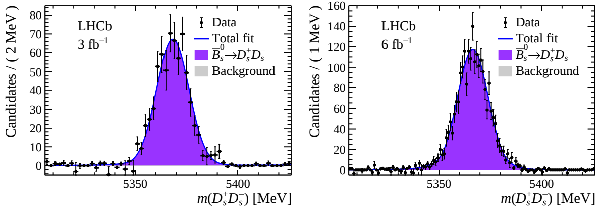
Figure 5: Mass distribution of the D_s^+ D_s^- system, with singly charmed and charmless backgrounds subtracted, shown for (left) Run 1 and (right) Run 2 data-taking periods. The fit projection (solid blue line) is shown together with the \bar{B}_s^0 \rightarrow D_s^+ D_s^- signal (filled purple) and the background (filled gray).
