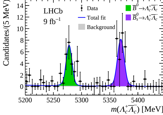
Figure 2: Mass distribution of the \Lambda_c^+ \bar{\Lambda}_c^- system with singly charmed and charmless backgrounds subtracted. The fit result (blue curve) is shown together with the signal components from \bar{B}^0 \rightarrow \Lambda_c^+ \bar{\Lambda}_c^- (filled green) and \bar{B}_s^0 \rightarrow \Lambda_c^+ \bar{\Lambda}_c^- (filled purple) decays, and the nonresonant background contribution (filled gray).
