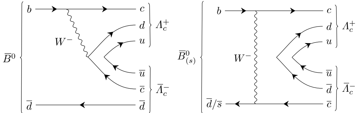
Figure 1: Tree-level Feynman diagrams for \bar{B}_{(s)}^0 \rightarrow \Lambda_c^+ \bar{\Lambda}_c^- decays. The left diagram shows the contribution from the W -emission process, while the right one depicts the W -exchange process.
