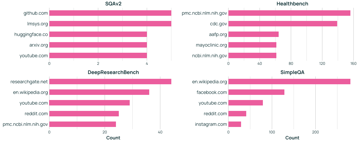
Figure 9 Distribution of domains among web search results for SQA v2 (science), HealthBench (healthcare), DeepResearchBench (general domain) and SimpleQA (factoid, short-form QA). We show top domains returned by the google_search tool. Calculations are based on 100 samples from each task. These top domains match the evaluation domain; e.g., when evaluating on HealthBench, DR Tulu searches more for medical domain websites.
