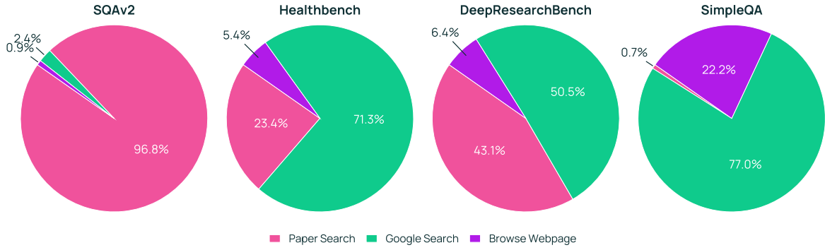
Figure 8 Distribution of tool calls for SQA v2 (science), HealthBench (healthcare), DeepResearchBench (general domain) and SimpleQA (factoid, short-form QA). DR Tulu can adaptively choose effective tools for different tasks, relying more on paper_search for scientific questions (SQA v2), and more on google_search for general-domain questions (SimpleQA).
