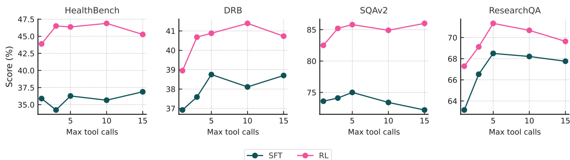
Figure 28 Ablations on maximum tool calls. We evaluate DR Tulu (SFT) and DR Tulu (RL) on four long-form datasets while varying the maximum number of allowed tool calls from 1 to 15, and report how performance changes under these caps.
