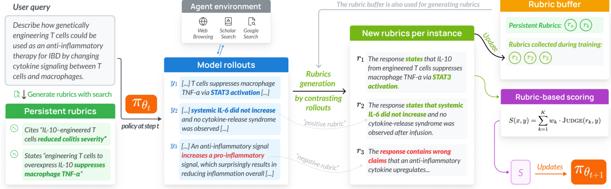
Figure 3 Training with RLER. Given a training instance, the policy LM \pi_{\theta_t} generates multiple rollouts via interacting with the environment. We then invoke another LM to create new rubrics based on those rollouts and the current rubrics in the rubric buffer. We score each generation against those rubrics and use that score to update model weights. We then add the new rubrics to the rubric buffer and filter it to retain only a fixed number of rubrics with the highest variance among rollouts.
