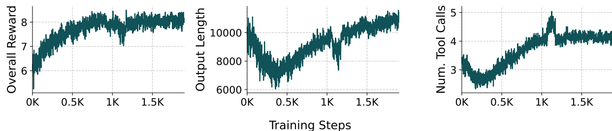
Figure 27 Overall reward, output length (in tokens, including tool outputs), and average number of tool calls during RL training. Note that during the run, we ran out of serper credits, causing a rise tool errors until we refilled the account, causing a drop in reward and output length, and a rise in tool calls (as the model retried the failed calls).
