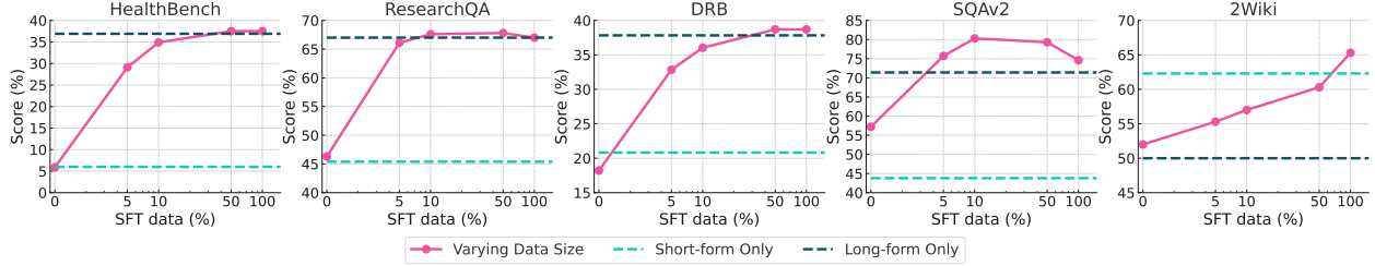
Figure 6 Ablation of SFT training data. We ablate SFT training data in terms of the mixture of data and scale of training data. We train models with varying sizes of SFT data (5%, 10%, 100%; 0% indicates the Qwen3-8B + dr-agent-lib results) as well as two SFT subsets, long-form data only (LF only) and short-form data only (SF only).
