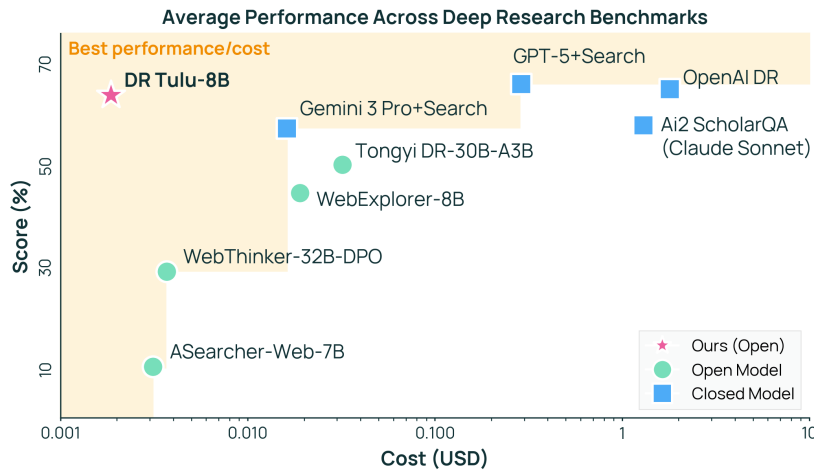
Figure 1 Performance vs. cost of deep research models. We report average performance over 4 long-form DR benchmarks (ScholarQA-CSv2, HealthBench, ResearchQA, and DeepResearchBench) against inference cost (USD per query on ScholarQA-CSv2). DR Tulu-8B lies on the Pareto frontier, outperforming larger open models and matching more expensive proprietary models. Full results in Table 2.
