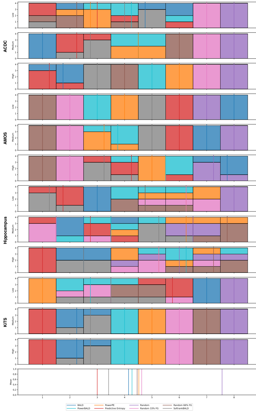
Figure 20: Leave-One-Out Detailed Results of Main Study for Final Dice. Ranking of methods according to AUC for each dataset and its Label Regimes (Low, Medium & High). A specific colored field of height 1 at x-axis x denotes that for one of the four seeds the method corresponding to this color obtained in the leave-one-out (seed based) ranking place x .
