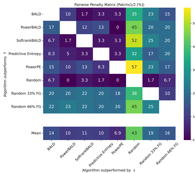
Figure 6: PPM for the \text{Patch} \times \frac{1}{2} configuration aggregated over all settings. Mean row results change compared to the \text{Patch} \times 1 (fig. 2).
