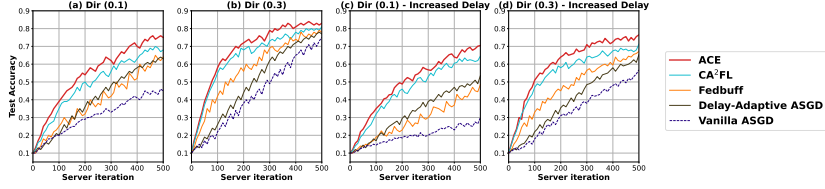
Figure 2: Impact of data heterogeneity (Dirichlet \alpha ) and client delay (Exponential mean \beta ) on CIFAR-10 test accuracy over 500 server iterations. (a) \alpha = 0.1 , low delay ( \beta = 5 ). (b) \alpha = 0.3 , low delay. (c) \alpha = 0.1 , increased delay ( \beta = 30 ). (d) \alpha = 0.3 , increased delay. ACE demonstrates robust performance toward various heterogeneity and delay. Extended results are in Appendix F.2.
