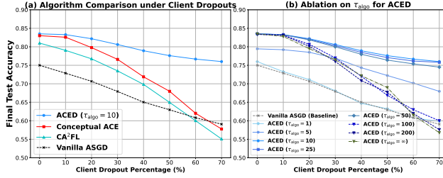
Figure 3: Final test accuracy ( T = 500 , \text{Dir}(\alpha = 0.3) , \beta = 5 ) vs. client dropout. (a) ACED ( \tau_{\text{algo}} = 10 ) shows superior dropout robustness compared to Conceptual ACE, CA 2 FL, and Vanilla ASGD. (b) Ablation on ACED’s \tau_{\text{algo}} : performance suffers if \tau_{\text{algo}} is too small (partial participation bias) or too large (staleness error), but is stable across moderate \tau_{\text{algo}} values.
