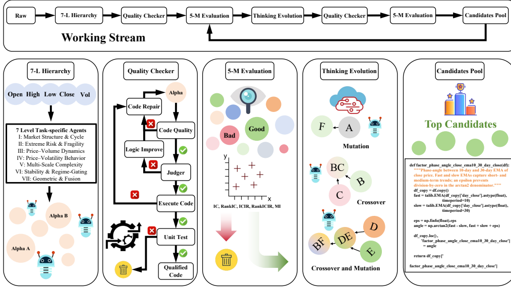
Figure 2: Overview of CogAlpha. The Seven-Level Agent Hierarchy produces initial alphas derived from the OHLCV data. The Multi-Agent Quality Checker verifies the validity and quality of each generated alpha code. The Filtering module evaluates all alpha codes using five predictive power metrics. Finally, the Thinking Evolution module iteratively refines and recombines qualified candidates through deeper reasoning by LLMs in each iteration.
