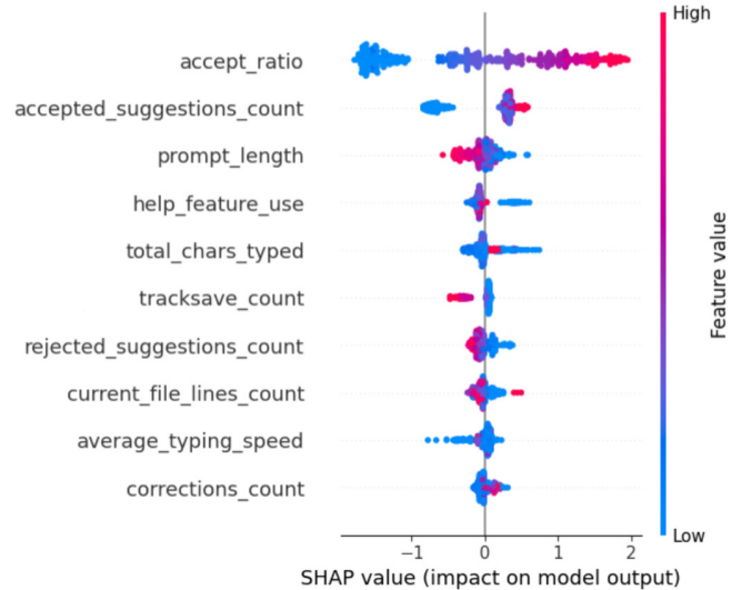
Fig. 1. SHAP value analysis for the CatBoost acceptance classifier.
