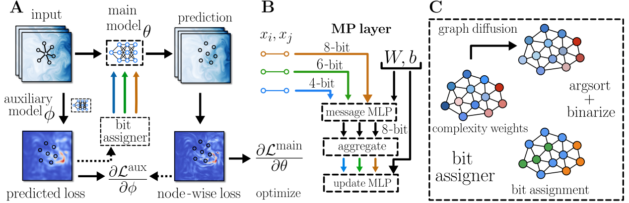
Figure 2: Overview of the training phase (A) . A lightweight auxiliary model assigns a complexity weight to every mesh node to guide the resource allocation of the large main message-passing model. Gradients do not flow through the dotted black arrows, i.e., backpropagation happens through the solid black arrows. (B) . The bit assignment process is schematically shown in (C) .
