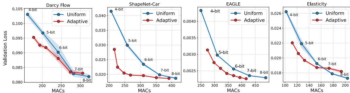
Figure 3: Validation loss vs cost (estimated in 10^9 MACs) for uniform vs adaptive (ours) quantization. The latter is obtained through increasing the fraction of Int8 nodes used, and includes the cost of the auxiliary model. Our framework demonstrates consistent Pareto improvements across all benchmarks. For Darcy, ShapeNet-Car and Elasticity, main models are MP-PDEs, for EAGLE - GraphViT.
