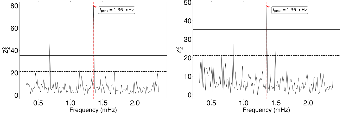
Figure 3. Z^2 soft X-ray (0.3–2 keV) periodograms. Left: combined MOS cameras. Right: PN camera. The red vertical line marks the most significant peak. The dashed and solid lines denote the 3\sigma and 5\sigma significance, respectively.
