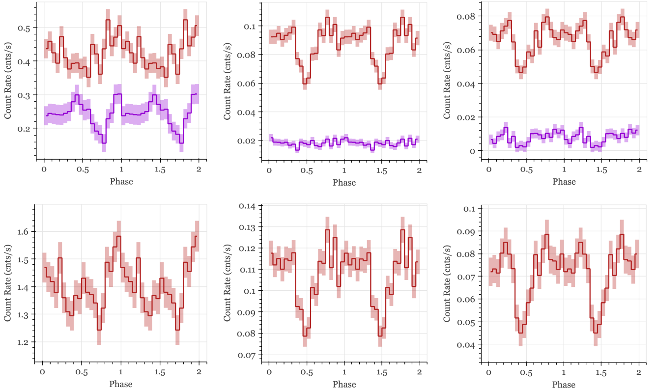
Figure 4. Folded lightcurve plots in the soft (0.3–4 keV for XMM-Newton and 1–4 keV for NICER ; red) and hard (4–10 keV; purple) X-ray band, with 1-\sigma error bars shown (left: NICER middle: XMM-MOS; right: XMM-PN). The bottom three figures show the combined folded lightcurves including photon energy up to 10 keV. All light curves are folded over the P = 12.26 min period, phase-aligned, and contain 20 bins per phase.
