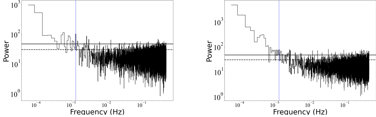
Figure 2. PDS periodograms obtained from the combined MOS (left) and PN (right) cameras. Blue vertical line marks the known optical periodicity P = 12.37 mins. Note that both axes are in log scale. The dashed and solid lines denote the 3\sigma and 5\sigma significance, respectively.
