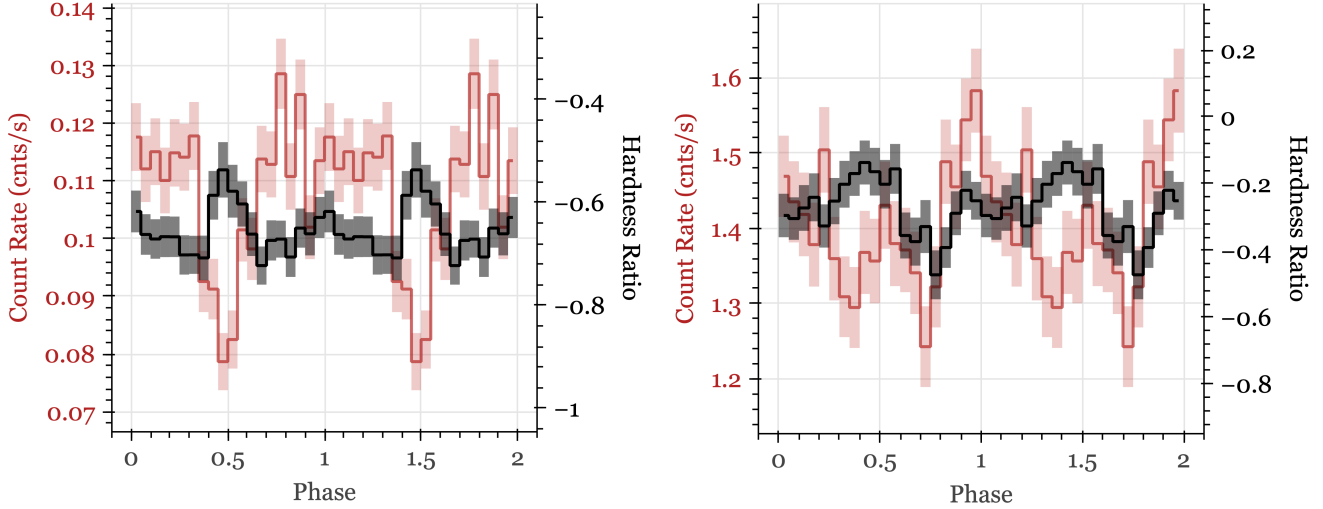
Figure 5. The hardness ratios (black) overlaid with the 0.3 – 10 keV (left: XMM-MOS) and 1 – 10 keV (right: NICER ) folded lightcurves, showing an anti-correlation. Both are folded at the P = 12.26 min period. Hardness ratio is defined as \frac{\text{hard} - \text{soft}}{\text{hard} + \text{soft}} , where the soft and hard energy bands are defined as E < 4 keV and E > 4 keV.
