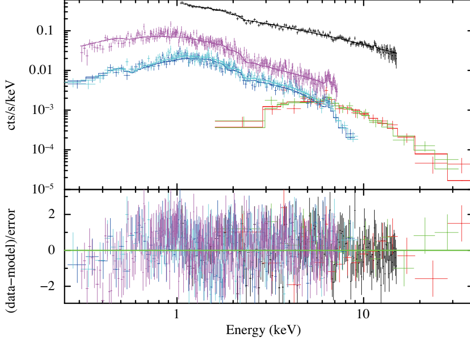
Figure 8. NICER (black), XMM-Newton (purple and blue), and NuSTAR (green and red) spectra of ZTF J1851 fit by the tbabs*(MCVSPEC+gauss) model with a Gaussian component fixed at 6.4 keV ( \chi^2_\nu = 1.00 ). For this particular case corresponding to the fractional accretion area fixed at f = 4 \times 10^{-4} , the best-fit WD mass is M = 1.25 \pm 0.01 M_\odot , with \dot{m} = 29.1 \text{ g cm}^{-2} \text{ s}^{-1} . While the statistical error is quoted for the WD mass measurement above, the systematic error is considered in our final results by considering a range of the fractional accretion area.
