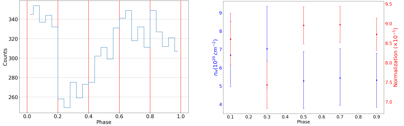
Figure 7. Results of phase-resolved spectroscopy. Left: The PN camera lightcurve folded at the 12.27 min period, with red lines demarcating the five phase bins ( \phi = 0.0 - 0.2, 0.2 - 0.4, 0.4 - 0.6, 0.6 - 0.8, 0.8 - 1.0 ). Right: The variation of the best-fit hydrogen column density n_H and flux normalization across phase bins, with fixed kT = 25.5 keV and Z = 1.0 Z_\odot .
