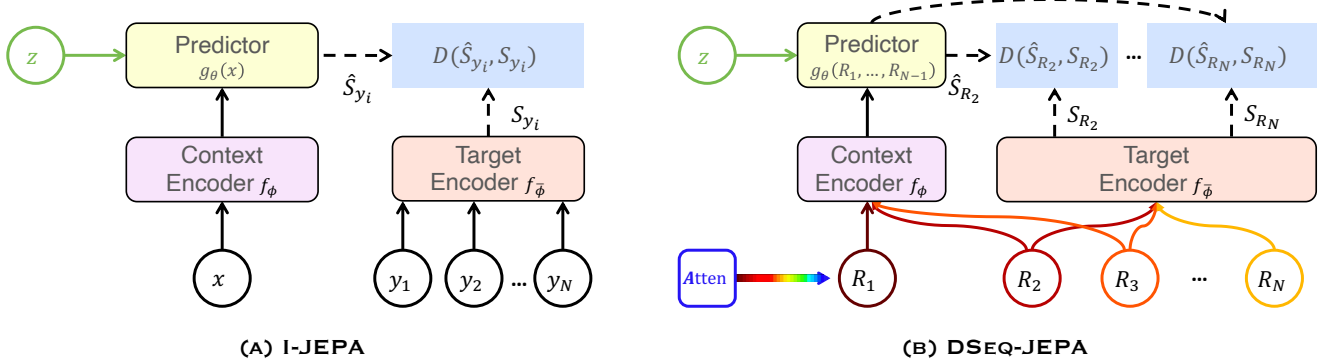
Figure 2. (A) I-JEPA learns to predict the embeddings of the target regions (y_1, \dots, y_N) from a single context region x , using a predictor network conditioned on latent variables z . While (B) DSeq-JEPA learns to predict the embeddings of the next discriminative regions \{R_2, \dots, R_N\} based on its sequence of pre-identified regions in a sequential manner, also using a predictor. The order of the discriminative regions is determined by the attention map of the image.
