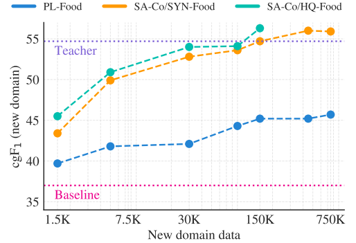
Figure 8 Domain adaptation via synthetic data. Synthetic (SYN) data generated by SAM 3 + AI verifiers (teacher system) achieves similar scaling behavior as human-annotated (HQ) data.
