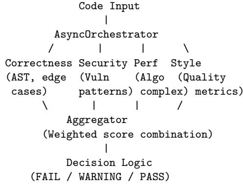
Figure 1: System architecture: parallel multi-agent analysis.
