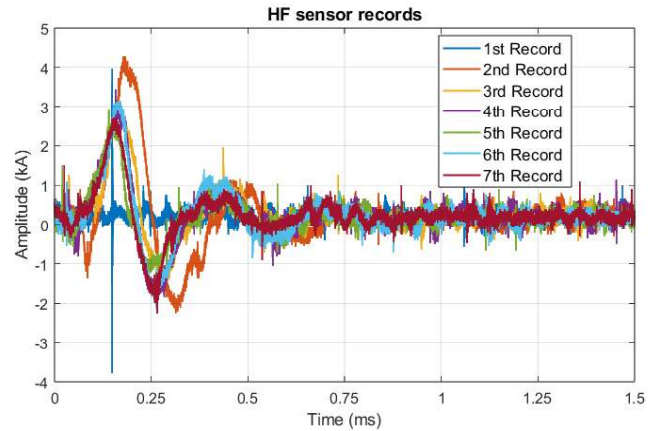
Fig. 7. HF sensor records of electromagnetic transients caused by the December 11 th lightning flash to WTG6, aligned to time zero.
