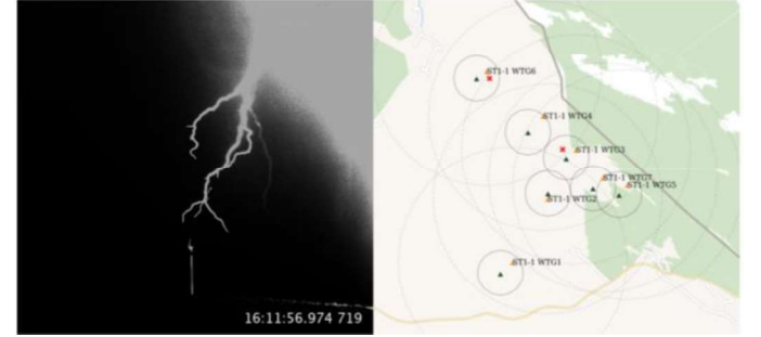
Fig. 3. HS camera frame when the luminance suddenly increased (left); Lightning flash activity recorded by LLS in that area at that exact time (right).
