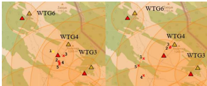
Fig. 9. September 3 rd , 2024, lightning flash (Figure 9a, left): April 25 th , 2023, lightning flash (Figure 9b, right).
