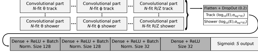
Figure 8: Details of the classifier network architecture. All convolutional blocks are connected in parallel to the feed-forward part.
