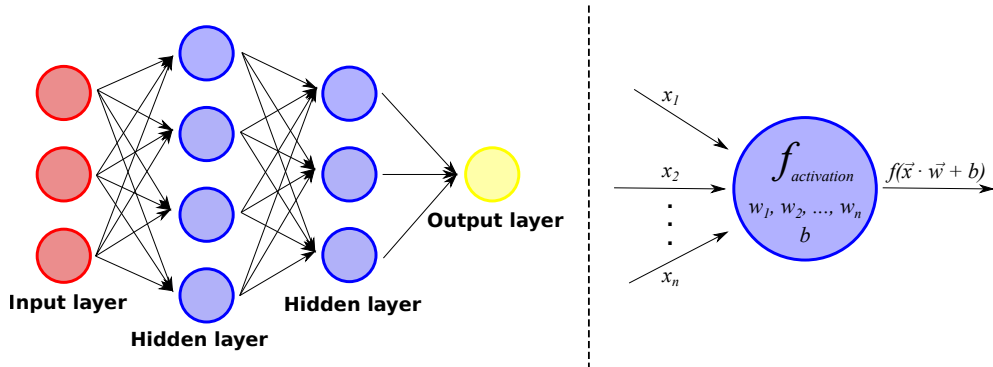
Figure 2: Schematic diagram of a simple feed-forward neural network. Circles represent neurons, and arrows represent synaptic connections. In general, more than a single output can be considered.
