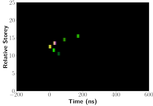
Figure 3: Example of a normalized RGB image from a track-like event ( \bar{\nu}_\mu^{\text{CC}} ).
