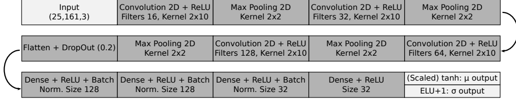
Figure 4: Details of the direction neural network architecture. Note that for the \theta prediction, we scaled the hyperbolic tangent activation function for \mu_\theta , so that its values lay in [0, \pi] radians. No scaling was necessary for the prediction of \phi since its estimation was derived from the Cartesian \{X, Y\} components of the unit vector.
