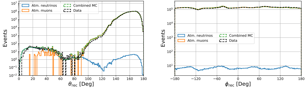
Figure B.23: Comparison between data and MC simulations using a cut of \sigma_{\Omega} < 21^{\circ} .
