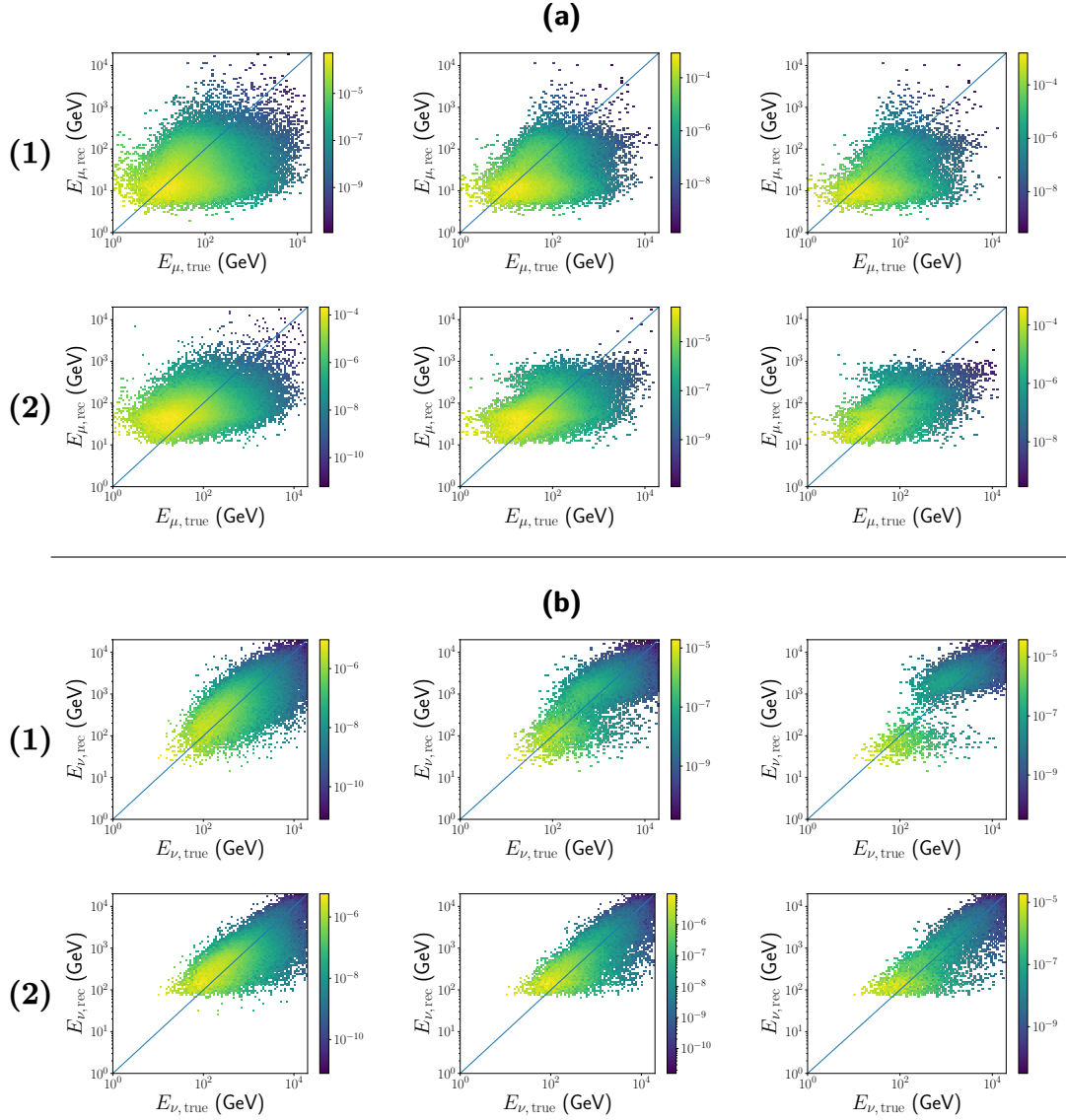
Figure 12: 2D density histograms of reconstructed vs. true energy values for the pre-selected test dataset (left), the 50% lowest values of \sigma (mid) and the 25% (right). (a) Track branch. (b) Shower branch. (1) Benchmark reconstruction. (2) Final reconstruction approach. The diagonal represents the ideal fit.
