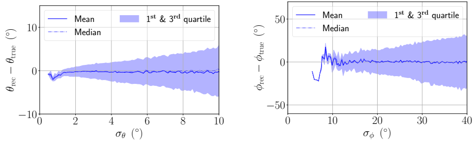
Figure 5: The error on angles \theta (left) and \phi (right) as a function of the predicted uncertainty for the track branch. The mean and median error stay close to zero with no significant bias. The first and third quartiles behave as expected for a Gaussian distribution, especially for \theta .
