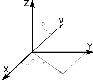
Figure 1: Schematic representation of the angles \theta and \phi that define the direction of a neutrino, \nu , in the ANTARES coordinate system.
