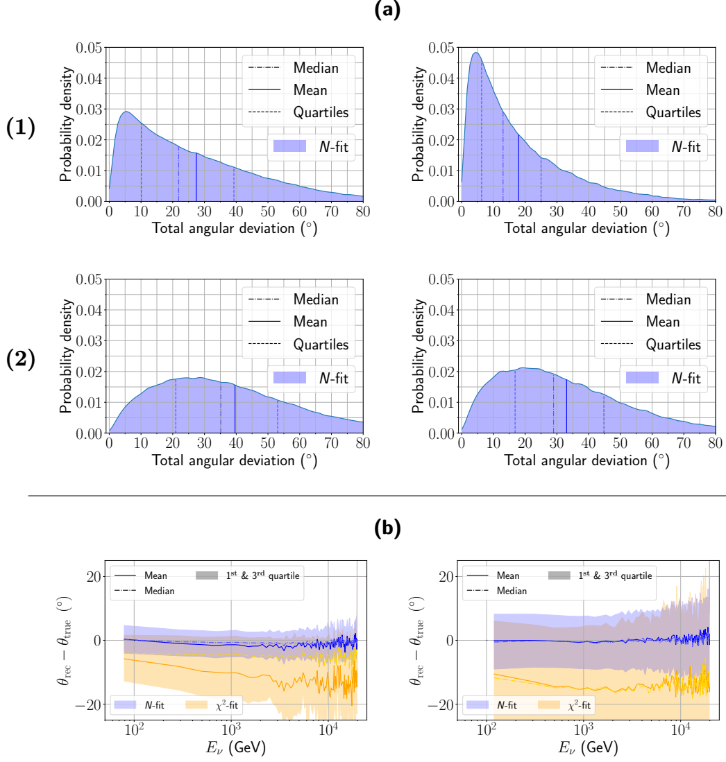
Figure 10: (a) Total angular deviation distribution for tracks (1) and showers (2) of all test dataset events (left) and of the 50% events with lowest value of \sigma_\Omega (right). (b) Angle \theta error as a function of the true neutrino energy for tracks (left) and showers (right).
