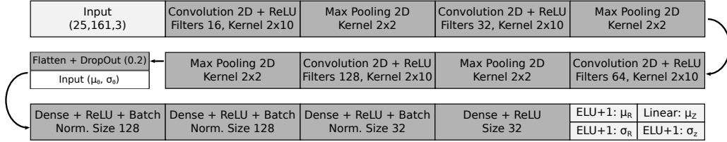
Figure 6: Details of the closest point and interaction vertex network architecture.
