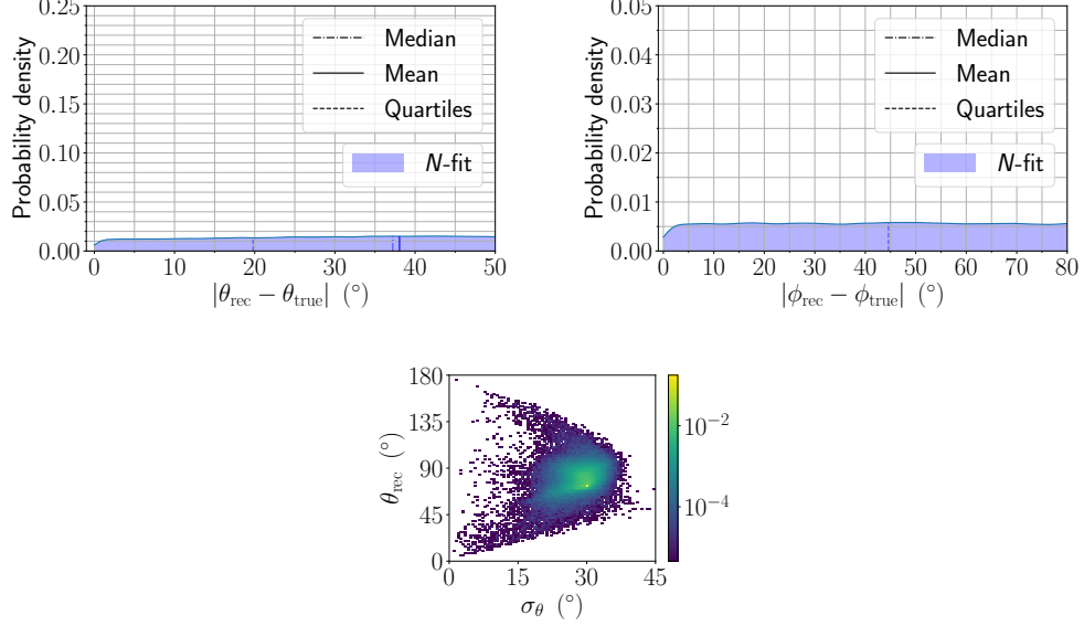
Figure B.21: Error distributions if the input of the networks is background noise in the track branch.
