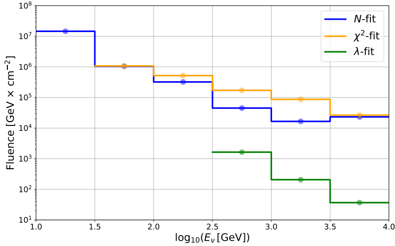
Figure 14: 90% confidence upper limits on the neutrino fluence as a function of the energy for N -fit, \chi^2 -fit and \lambda -fit from PKS 0735+17 over \pm 1 day around 20:02:51.1 UT on December 8, 2021. The values of the study performed with the \lambda -fit reconstruction are taken from [34], while the values for \chi^2 -fit –using only SL events– were computed just for comparison purposes.
