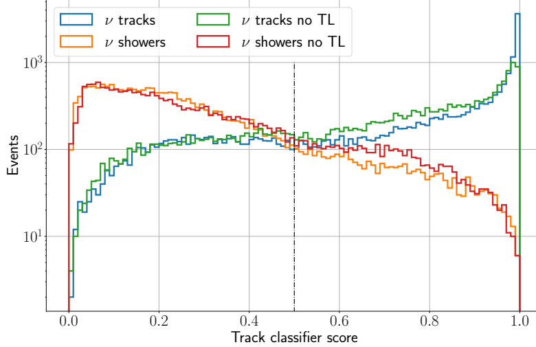
Figure 13: Distributions of the track score according to the N -fit classifier, with and without Transfer Learning (TL), for tracks and showers.
