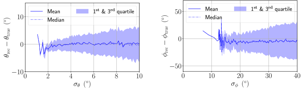
Figure A.15: The error on angles \theta (left) and \phi (right) as a function of the predicted uncertainty for the shower branch. The mean and median error stay close to zero with no significant bias. The first and third quartiles behave as expected for a Gaussian distribution, especially for \theta .
