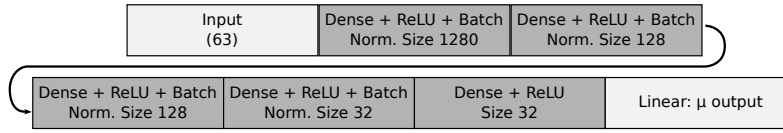
Figure 7: Details of the energy network architecture.
