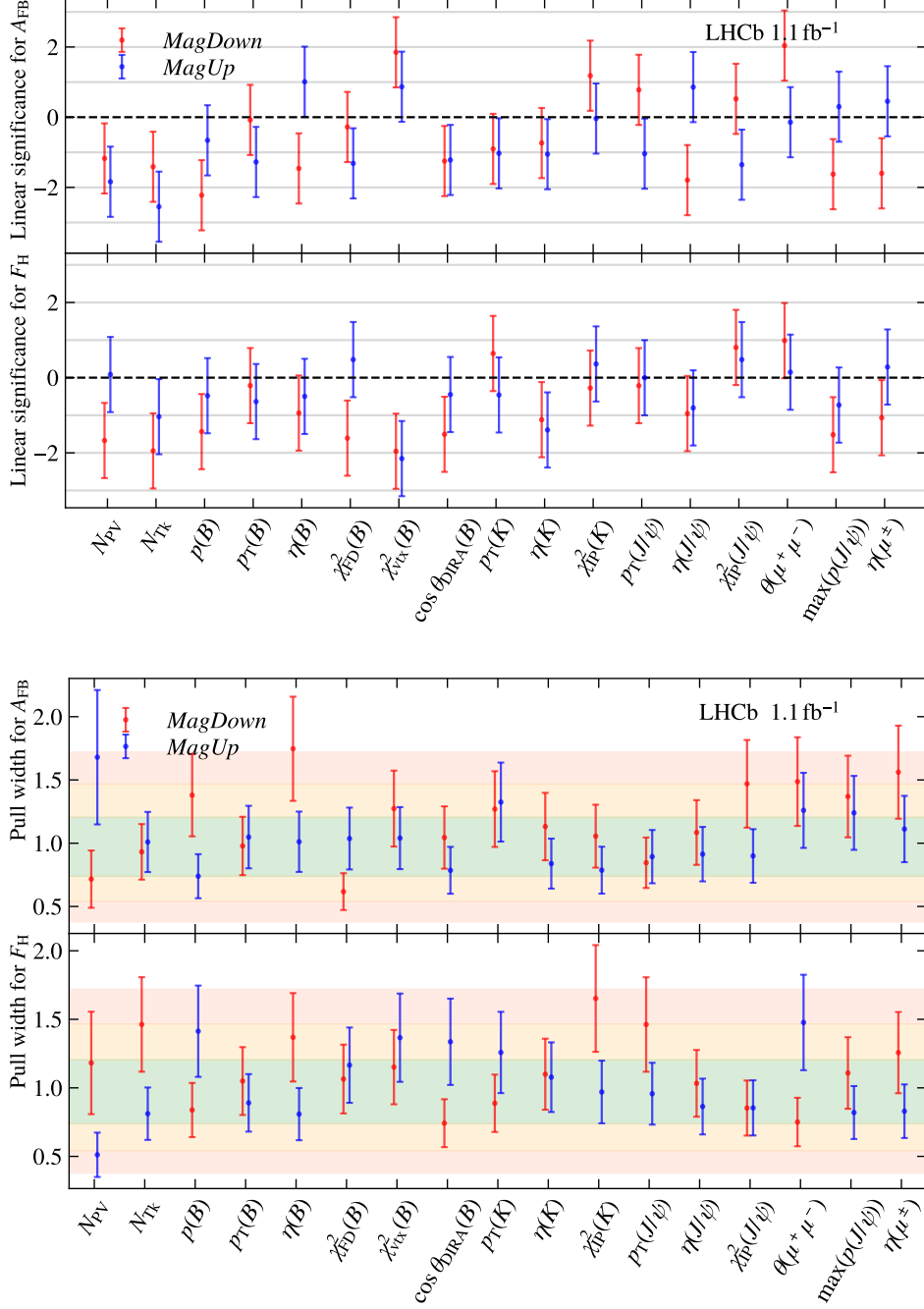
Figure 5: (Top) Significance of the linear parameter obtained from a \chi^2 fit of the differential variation of the observables A_{\text{FB}} and F_{\text{H}} as a function of all 17 variables considered. (Bottom) Standard deviation of the pull distribution obtained for the observables A_{\text{FB}} and F_{\text{H}} across the same 17 variables. The green, orange, and red bands indicate the 68.27%, 95.45%, and 99.73% confidence intervals for the width of the pull distribution, derived from pseudoexperiments in which pseudodata is randomly split into ten equally populated bins.
