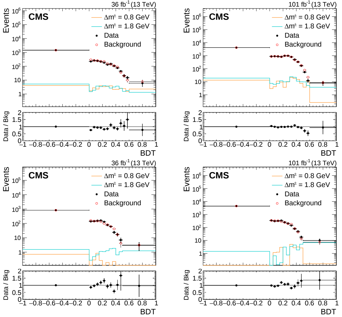
Figure 5: Prefit expected and observed distributions of the event BDT output score in the SRs for the muon + exclusive track category (upper), and the electron + exclusive track category (lower), shown separately for Phase 0 (left) and Phase 1 (right). In the lower panel, the vertical black bars represent the total uncertainty, including both statistical and systematic components. Example signal benchmark scenarios are also shown as colored lines.
