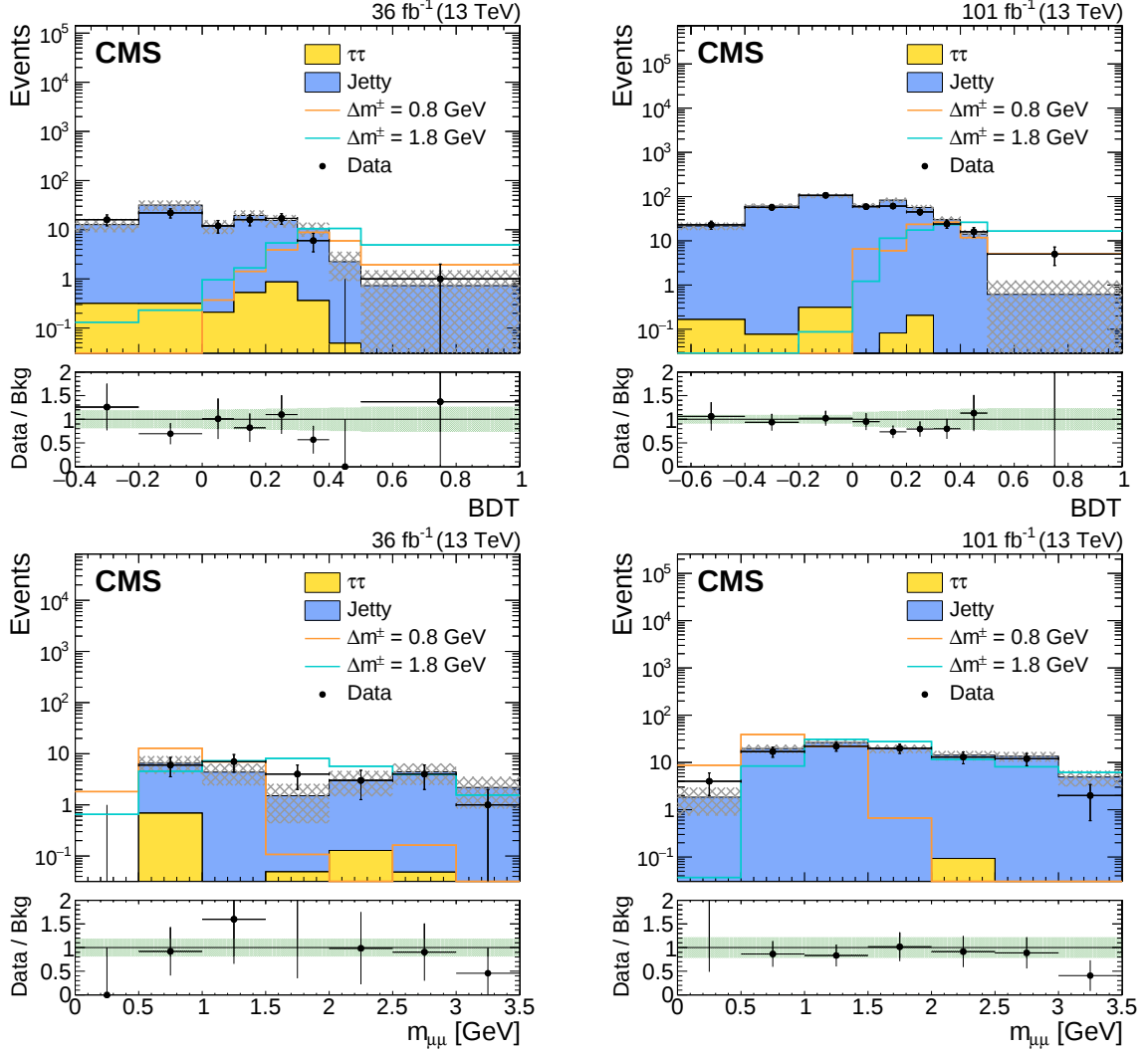
Figure 4: Prefit expected and observed distributions of the event BDT output score in the SRs for the dimuon category (upper) and of the dimuon invariant mass for events with event classifier scores greater than 0.1 (lower), shown separately for Phase 0 (left) and Phase 1 (right) configurations. The gray hatching shows the statistical uncertainty in the background prediction. In the lower panel, the green band indicates the relative systematic uncertainty in the predicted background, while the black bars represent the total uncertainty, including both statistical and systematic components. Two example signal scenarios are also shown as colored lines.
