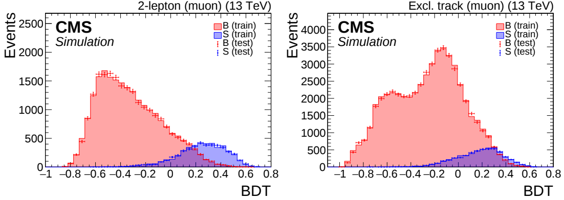
Figure 2: Unweighted distributions of the event-level BDT scores for events from the signal and background training samples in the dimuon category (left) and the muon+track category (right), based on the Phase 1 detector configuration.
