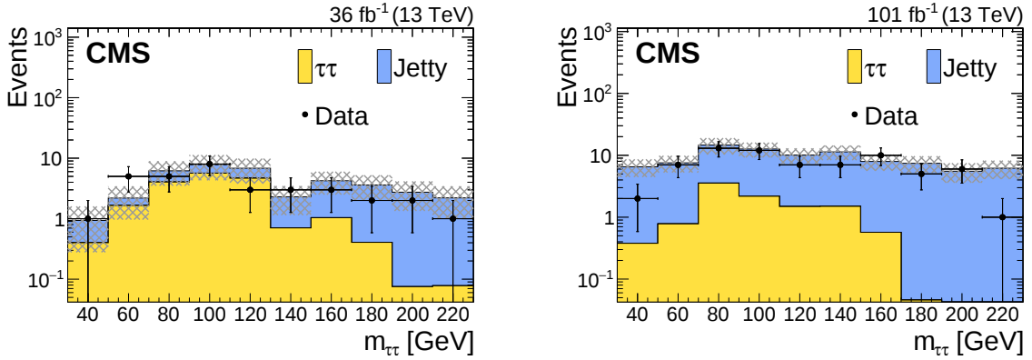
Figure 3: Distributions of the reconstructed ditau invariant mass ( m_{\tau\tau} ) in the BDT sideband CR, shown for Phase 0 (left) and Phase 1 (right) detector configurations. The non- \tau\tau background is estimated using the data-driven Jetty background method described in the text. The gray hatching shows the statistical uncertainty in the background prediction.
