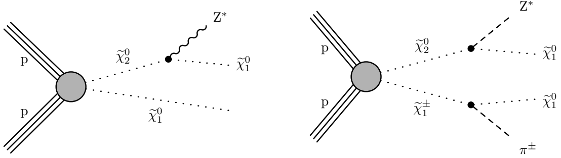
Figure 1: Diagrams illustrating the production and decay of electroweakinos in the Higgsino simplified model via the \tilde{\chi}_2^0 \tilde{\chi}_1^0 (left) and \tilde{\chi}_2^0 \tilde{\chi}_1^\pm (right) processes.
