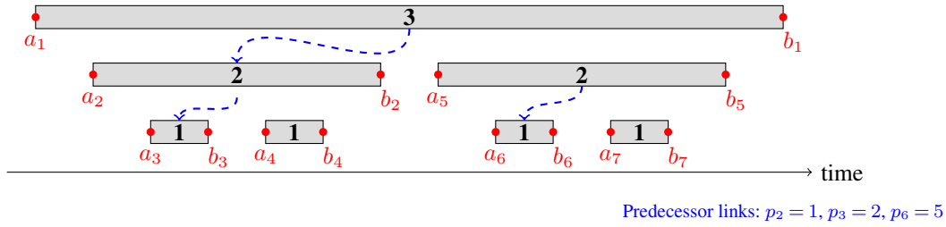
Figure EC.3 Example EC.2: A complete binary-tree hierarchy of seven intervals. Each parent fully contains its two children. Both endpoints (a_i, b_i) for each interval i are marked in red. The bold number inside each interval indicates its IAP assignment \hat{I}_i , and the blue dashed arrows illustrate the predecessor links p_j = i that define the partition satisfying PARTITION-MONOTONICITY .
