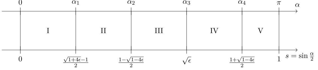
FIG. 14: As \alpha varies from 0 to \pi , J_\Lambda assumes 5 different expressions (Eqs. (A27)–(A31)). The corner points \alpha_n that separate these expressions are given by \sin \frac{\alpha_n}{2} = j_n(\epsilon) , where j_n(\epsilon) is given on the lower axis.
