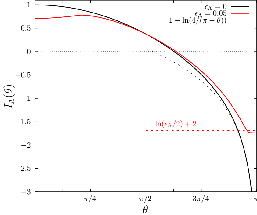
FIG. 2: Angular dependence of the function I_\Lambda appearing in \mathcal{A}_{\uparrow\downarrow} and f_{\uparrow\downarrow} . For \epsilon_\Lambda = 0 (black curve), the function displays a logarithmic divergence \sim \ln(\pi - \theta) + 1 - \ln 4 when \theta \rightarrow \pi (black dashed curve). For \epsilon_\Lambda \neq 0 (red curve) the divergence is regularized, and the function saturates at \ln(\epsilon_\Lambda/2) + 2 + O(\epsilon_\Lambda) in \theta = \pi (red dashed curve).
