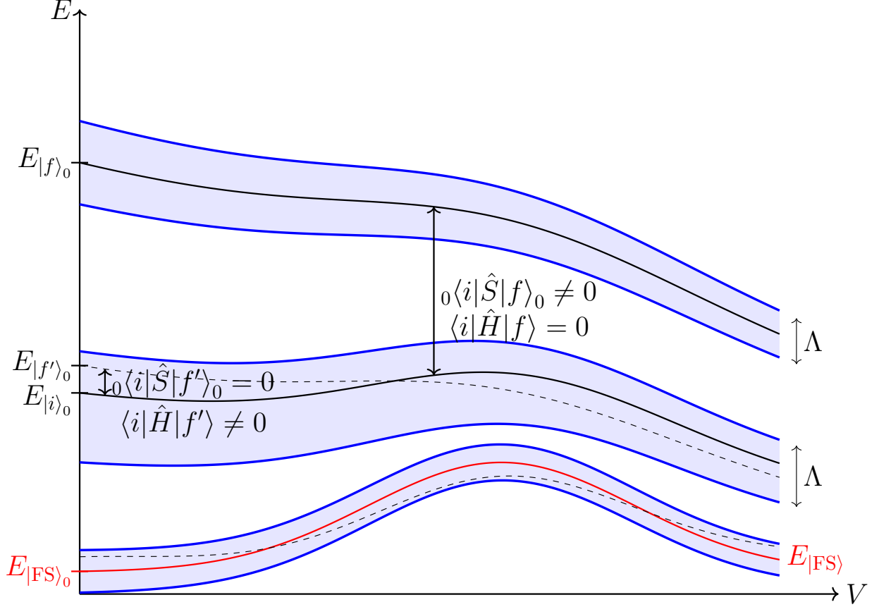
FIG. 1: Construction of the quasiparticle states within quasi-degenerate perturbation theory. An unperturbed Fock state |i\rangle_0 is dressed via the operator \hat{S} by its interactions with the off-resonant states |f\rangle_0 , whose unperturbed energy verifies |E_{|f\rangle_0} - E_{|i\rangle_0}| > \Lambda (here E_{|i\rangle_0} = {}_0\langle\psi|\hat{H}_0|\psi\rangle_0 ). The dressed state |i\rangle can then be followed adiabatically as the interaction strength V increases. However, due to its incomplete dressing, it is not an eigenstate of \hat{H} , and it remains coupled to the nearly degenerate states |f'\rangle of energies |E_{|f'\rangle} - E_{|i\rangle}| < \Lambda , (here E_{|i\rangle} = \langle\psi|\hat{H}|\psi\rangle ). This construction applies in particular to the particle Fermi sea |FS\rangle_0 , which evolves into a quasiparticle Fermi sea |FS\rangle (red curve). In general the quasiparticle Fermi sea is not the ground state of \hat{H} , and therefore not the ground state of our effective Hamiltonian.
