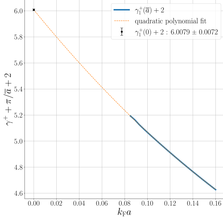
FIG. 16: The reduced speed of the collisionless density sound \gamma^+ + 2 + \pi/\bar{a} with \gamma^+ = \log((c_0^+ - 1)/2) . The blue curve is obtained by numerically solving (B2) in the range k_F a = 0.16, 0.085 . A quadratic polynomial fit (orange curve) provides the value extrapolated to k_F a = 0 : \gamma_1^+ + 2 = 6.0079 \pm 0.0072 .
