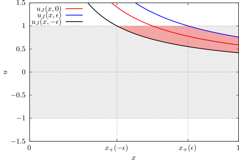
FIG. 12: The resonance angle u_J(x, \epsilon = 0) (red curve) and the forbidden band x \mapsto [u_J(x, -\epsilon), u_J(x, \epsilon)] (red area) inside the integration domain [0, 1] \times [-1, 1] (grey area) for J_\Lambda at \alpha = 0.4\pi and \epsilon = 0.1 .
