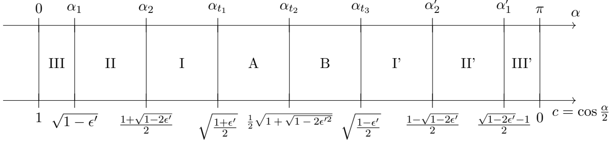
FIG. 13: As \alpha varies from 0 to \pi , I_\Lambda assumes 8 different expressions (Eqs. (A16)–(A23)). The corner points \alpha_n that separate these expressions are given by \cos \frac{\alpha_n}{2} = i_n(\epsilon') , where i_n(\epsilon') is given on the lower axis.
