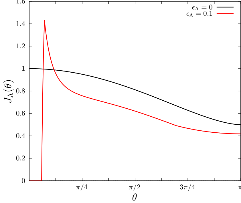
FIG. 3: Angular dependence of the function J_\Lambda appearing in both \mathcal{A}_{\uparrow\downarrow} , f_{\uparrow\downarrow} and \mathcal{A}_{\sigma\sigma} , f_{\sigma\sigma} . As \epsilon_\Lambda \rightarrow 0 , the function converges pointwise to J(\theta) (black curve) on (0, \pi] . It is however cancelled in an interval of width \simeq 2\epsilon_\Lambda about \theta = 0 (red curve).
