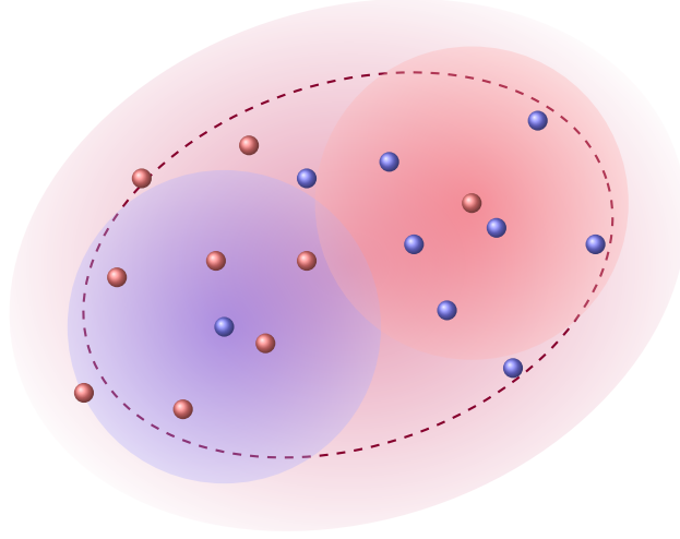
FIG. 11: Cooper pairs (dashed ellipse) in a Fermi superfluid are pairs of \uparrow and \downarrow Landau quasiparticles (red and blue clouds). To first order, the spin- \uparrow quasiparticle can be seen as a cloud of spin- \downarrow particles (blue dots) surrounding the original spin- \uparrow particle (red dot).
