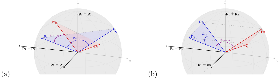
FIG. 5: (a) The angular parametrization where \mathbf{p}_1 + \mathbf{p}_2 is chosen as the polar axis of the spherical frame. This parametrization is used for W_E in Eq. (173). (b) The angular parametrization where \mathbf{p}_1 - \mathbf{p}_3 is chosen as the polar axis of the spherical frame. This parametrization is used for W_S in Eq. (174). The last parametrization where \mathbf{p}_1 - \mathbf{p}_4 is chosen as the polar axis is not shown here.
