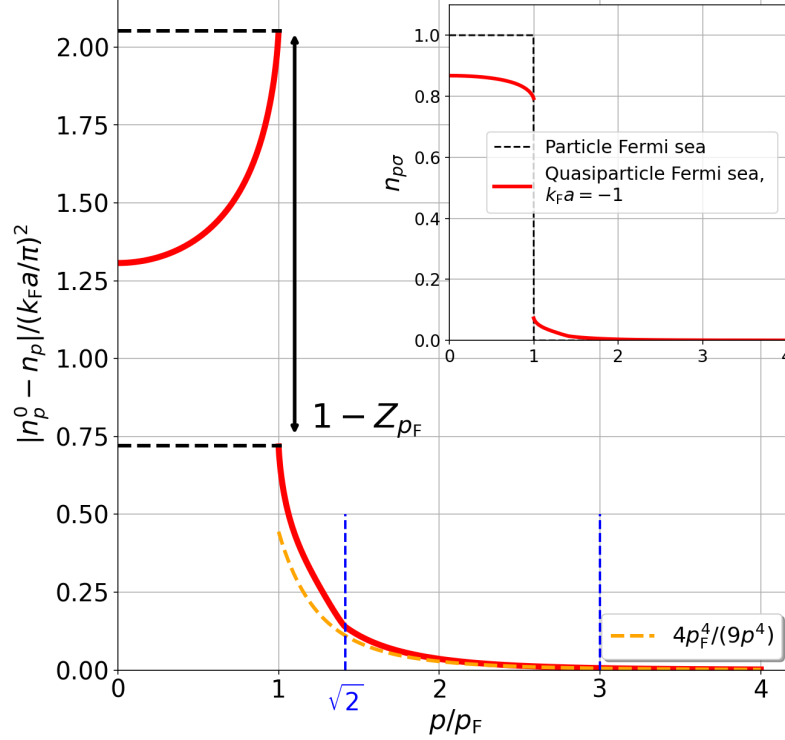
FIG. 4: (Main pannel) Difference between the particle momentum distribution n_p^{[\text{FS}]} = \langle \text{FS} | \hat{a}_{\mathbf{p}\sigma}^\dagger \hat{a}_{\mathbf{p}\sigma} | \text{FS} \rangle (see Eq. (100)) and the zero-temperature Fermi-Dirac distribution n_p^0 as a function of p/p_F . The difference is scaled to (k_F a / \pi)^2 so as to be independent of a in the weak-coupling limit. The discontinuity across the Fermi surface, i.e. between the asymptotic values in p_F - 0^- and p_F + 0^+ (black dashed lines), is given by 1 - Z_{p_F} . At large momenta, the distribution follows a 1/p^4 behavior, from which the contact C = 4\bar{a}^2/9\pi^2 can be extracted (orange dashed curve). (Inset) The bare distribution n_p^{[\text{FS}]} in function of p/p_F , evaluated in second-order perturbation theory at k_F a = -1 . The distribution displays the familiar shape of a depleted Fermi sea, with n_p < 1 down to p = 0 .
