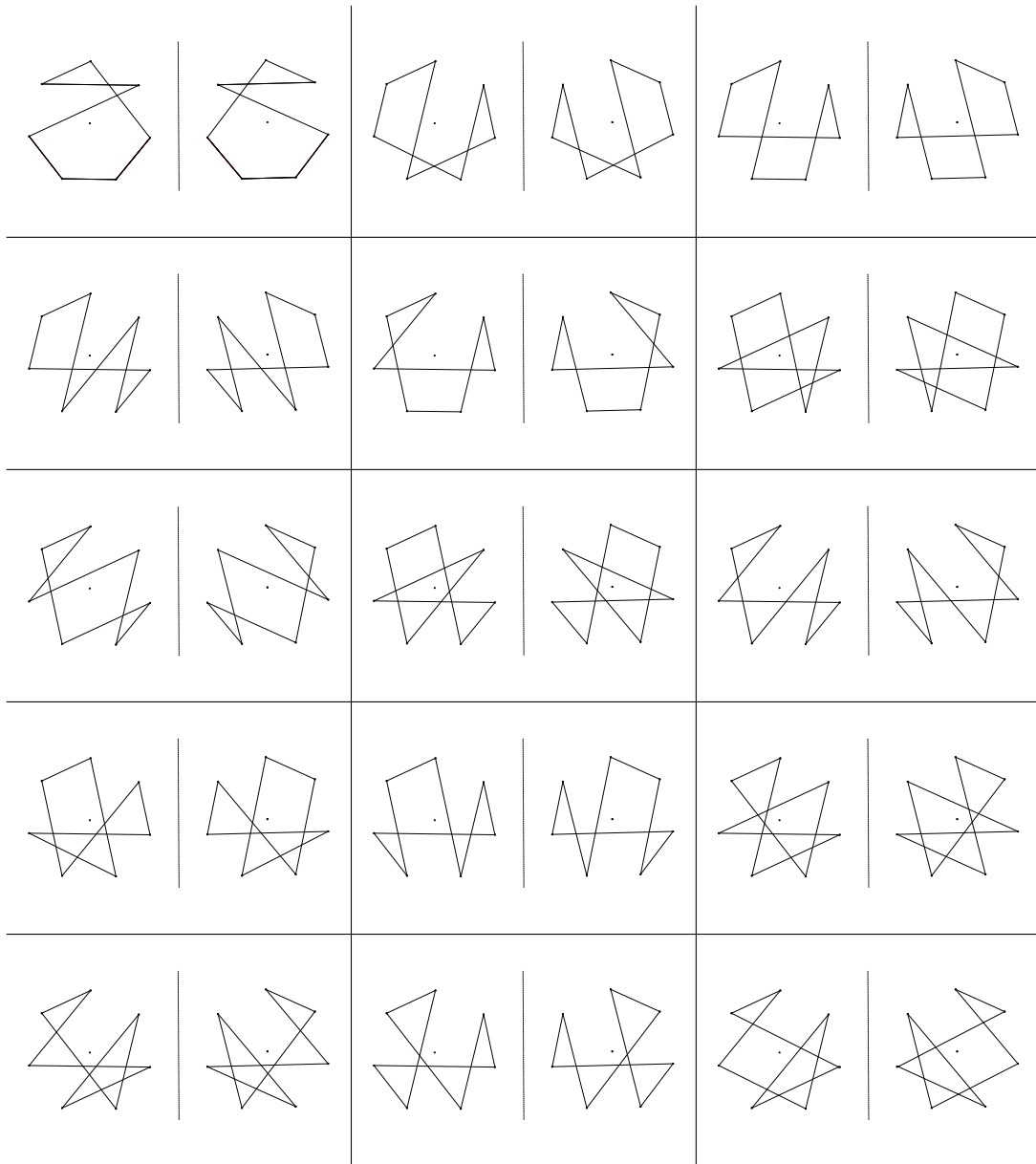
Figure 5: representatifs of the 30 equivalence-classes of asymmetrical 7-polygons
