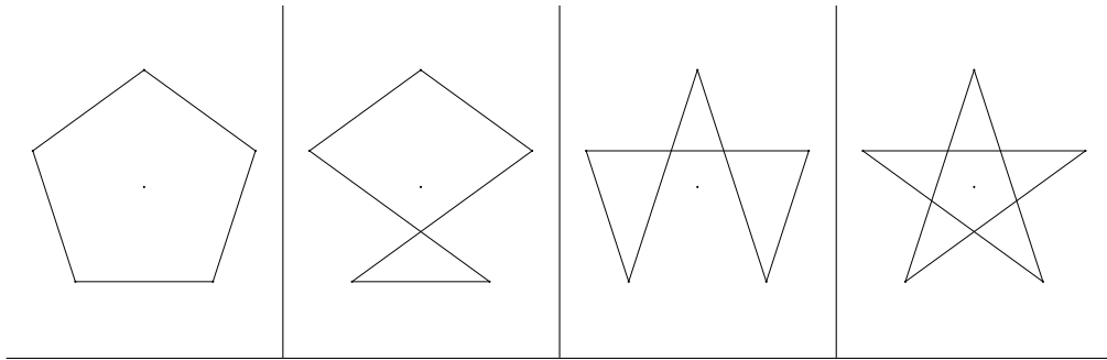
Figure 4: representatifs of the 4 equivalence-classes of the 5-polygons
