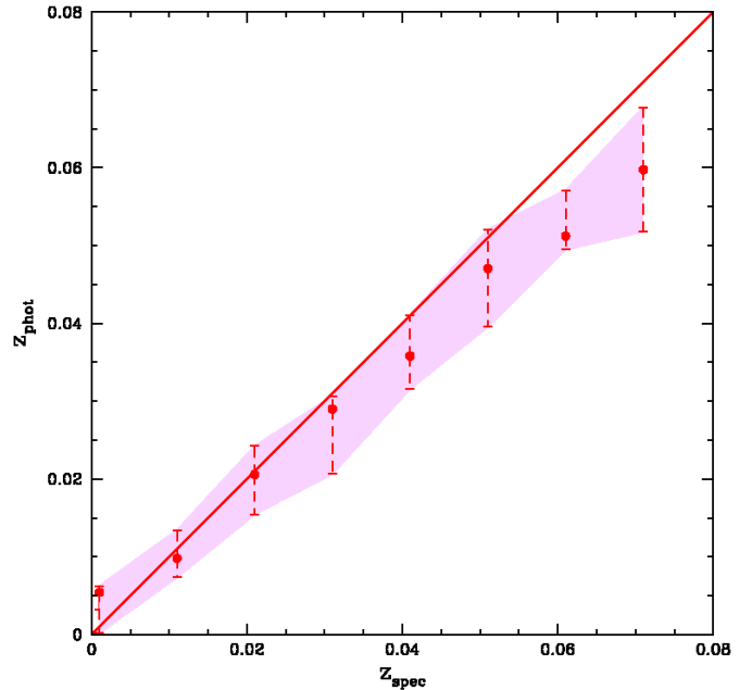
Fig. 4. Calibration results for the ANNz code. The solid line indicates the one-to-one relation between spectroscopic and photometric redshifts. The red points represent the mean photometric redshift within each spectroscopic redshift bin, with error bars indicating the standard deviation. The pink shaded region shows the calculated uncertainties in the distribution.
