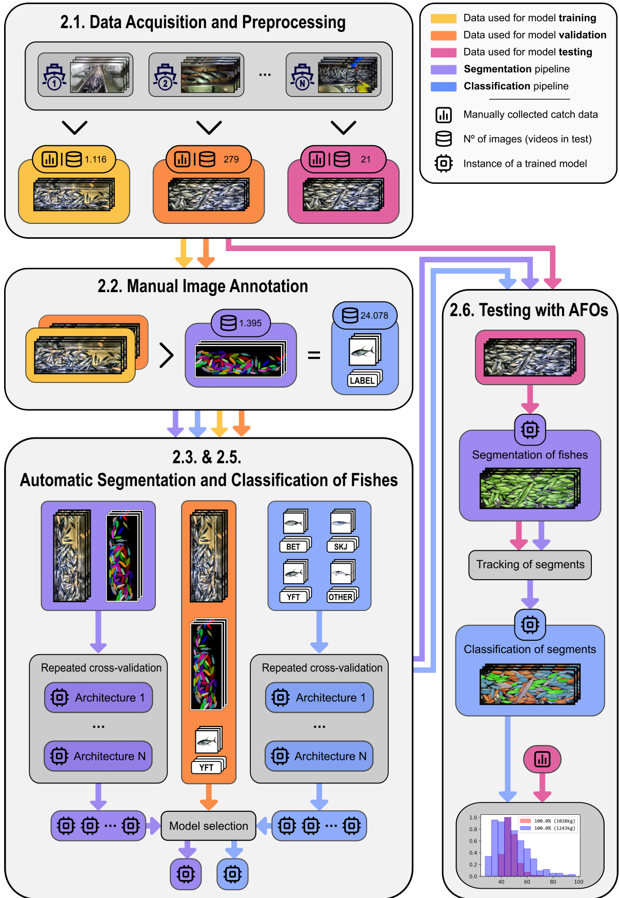
Figure 1. Workflow that outlines the pipeline for fish image analysis. It begins with the collection and manual annotation of images, followed by model training using cross-validation to select the best-performing architecture. The selected model is then used to automatically segment and classify fish in images. Finally, the pipeline is tested on real-world data. This process ensures robust and accurate fish identification.
