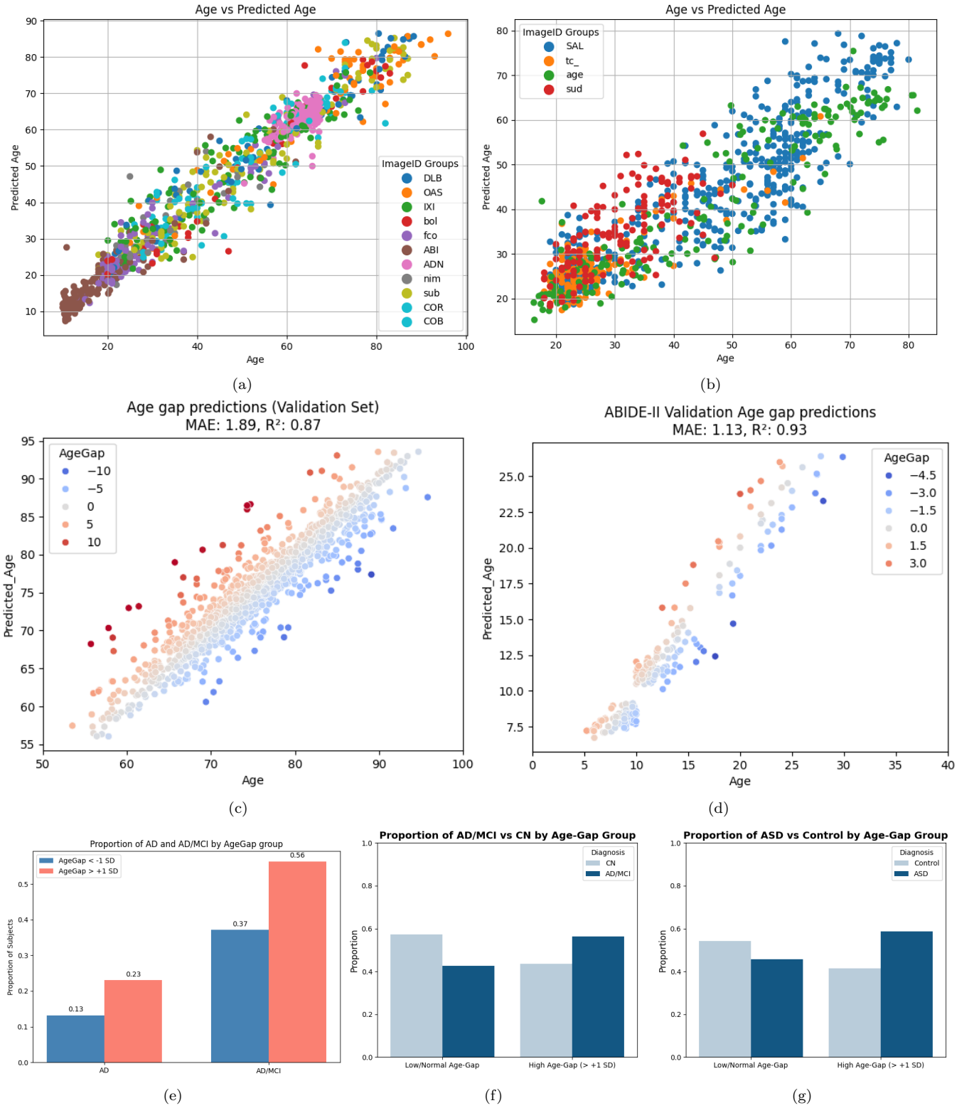
Figure 3: (a) : Scatter plot of predicted age of validation samples from 11 datasets (MAE = 3.34 years, Pearson r = 0.98 , Spearman \rho = 0.97 , R^2 = 0.95 ). (b) : Scatter plot of predicted age of independent test samples from 4 datasets (MAE = 4.72 years, Pearson r = 0.88 , Spearman \rho = 0.90 , R^2 = 0.83 ). (c) : Scatter plot of validation on 5,581 ADNI subjects only. (d) : Scatter plot of validation on 1,141 ABIDE-II subjects only. (e) : Proportion of AD and AD/MCI subjects with extreme positive aging ( BAG > 1std.dev. ) and extreme negative aging ( BAG < -1std.dev. ) visualized. (f) Proportion of AD/MCI subjects with extreme positive aging ( BAG > 1std.dev. ) visualized against other AD/MCI subjects in ADNI. (g) Proportion of ASD subjects with extreme positive aging ( BAG > 1std.dev. ) visualized against other ASD subjects in ABIDE-II.
