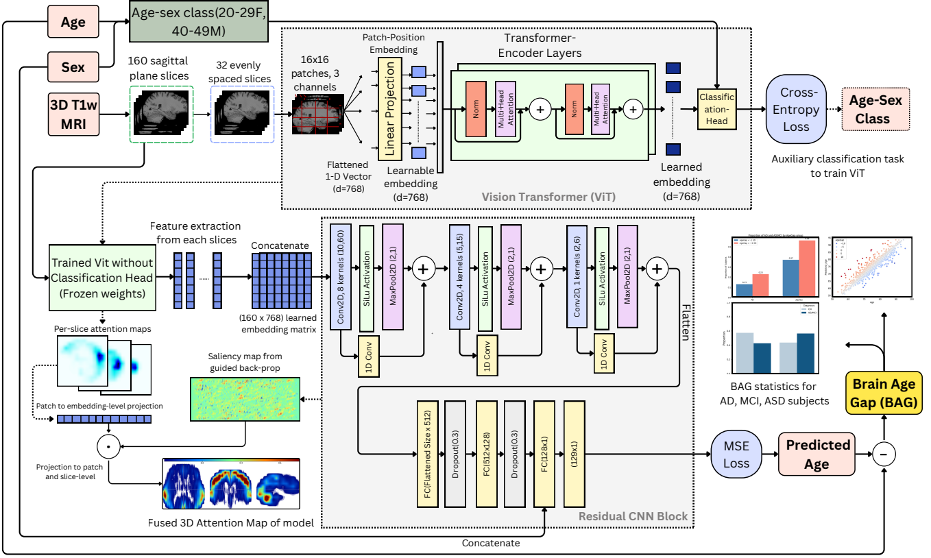
Figure 1: Overview of the proposed framework for 3D brain MRI analysis. The model integrates a Vision Transformer (ViT) encoder to extract slice-level embeddings with a lightweight 2D convolutional regression head to aggregate volumetric information. By applying convolutions over transformer-derived embeddings, the framework jointly models global contextual and local spatial patterns, enabling subsequent analyses on brain age gaps and thus linking aging with neurological conditions such as Alzheimer’s disease, mild cognitive impairment, and autism spectrum disorder.
