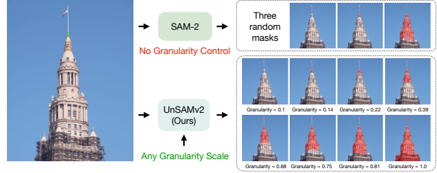
Figure 3. From ambiguity to control. Without granularity input, SAM-2 yields up to three masks per point, requiring users to manually choose one. UNSAMv2 resolves this ambiguity by introducing a continuous granularity variable, allowing users to obtain the intended object at any scale with a single prompt. This simple addition turns segmentation from a discrete guess into a continuous, controllable reasoning process.
