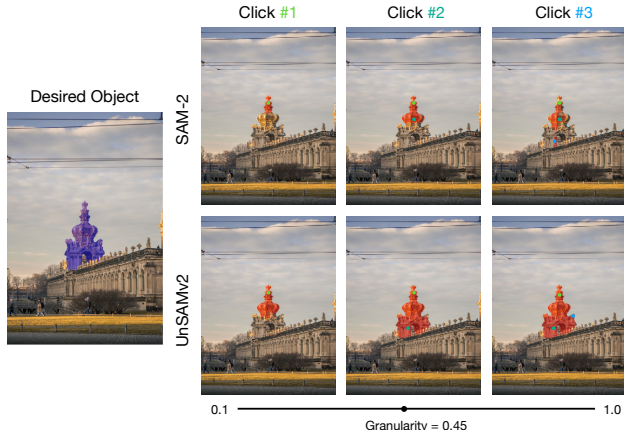
Figure 11. Fewer prompts, more control. SAM-2 often needs multiple clicks to isolate the target object. With a single granularity value, UNSAMv2 finds the correct mask efficiently, and it can also work with multi-point prompts for finer control.
