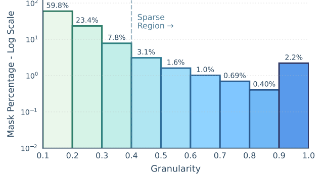
Figure 4. Granularity distribution of discovered masks. Our divide-and-conquer pipeline produces a rich, left-tailed hierarchy of pseudo-masks, dominated by fine-grained structures. Despite this imbalance, UNSAMv2 learns stable semantics across all scales. Hierarchical perception can emerge from unlabeled data!
