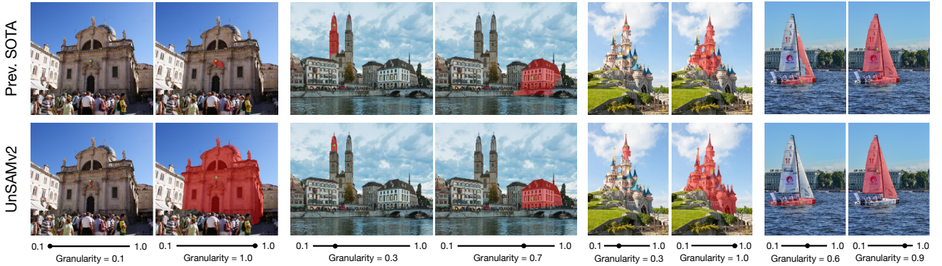
Figure 7. Qualitative comparison with the previous state-of-the-art method [58]. Each scene shows results at different target granularity values. Prior methods often break one object into parts at high granularity or include extra regions at low granularity. In contrast, UNSAMv2 produces clear and consistent masks with smooth transitions across scales.
