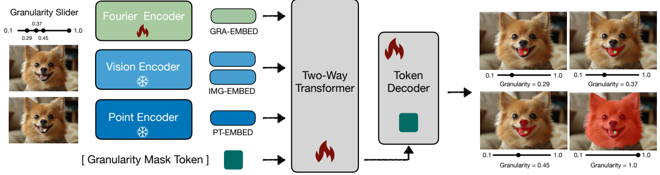
Figure 6. Architecture of UNSAMv2. Built on SAM-2, UNSAMv2 introduces a Fourier-based granularity encoder and a granularity-aware mask token to enable segmentation at arbitrary granularity. A scalar granularity input g \in [0.1, 1] is mapped to a high-dimensional embedding via Fourier transformation and an MLP, then injected into the transformer alongside the sparse point prompt embedding and dense image embedding. The granularity-aware mask token attends to image, point, and granularity embeddings, and is finally decoded by a token decoder into a mask at the requested granularity.
