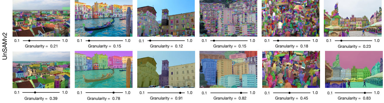
Figure 8. Visualizations for whole-image segmentation. Low granularity reveals fine parts, while higher values recover whole objects. UNSAMv2 offers controllable, scalable whole-image segmentation capability, even for scenes with many densely packed entities.
