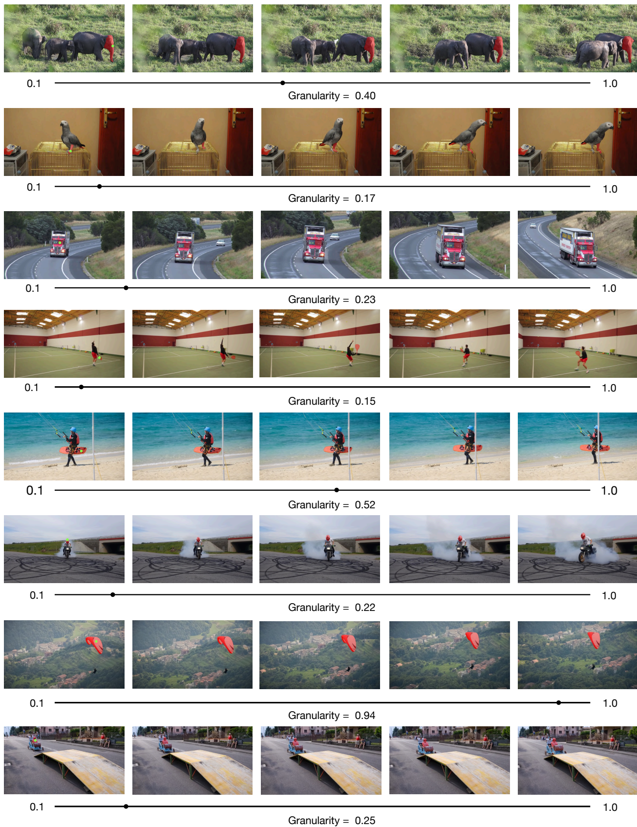
Figure A3. UNSAMv2's interactive video segmentation results on YoutubeVIS dataset at various granularity levels.
