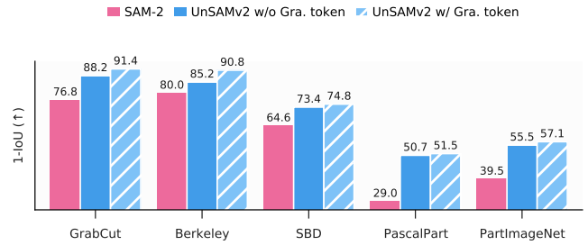
Figure 10. Ablation of granularity-aware mask token. Directly finetuning the original SAM-2 mask tokens leads to limited gains, suggesting they already encode strong mask priors. Adding our granularity-aware token enables efficient learning of granularity.
