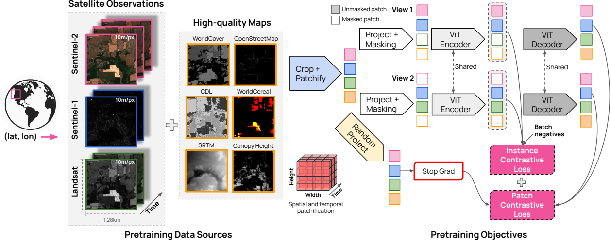
Figure 3 We train OlmoEarth with a combination of satellite observations and high-quality maps. After tokenizing these inputs, we: (1) apply a modality-aware masking strategy to define which tokens are inputs vs. targets, (2) pass the target tokens through fixed random projections to construct targets, (3) pass the input tokens through our learned encoders, and then (4) through a decoder which predicts the target tokens and (5) apply a modality-aware patch discrimination loss between the predicted and target tokens. Steps 1-5 are applied twice on the same data to then (6) apply an instance contrastive loss over the aggregated tokens per instance.
