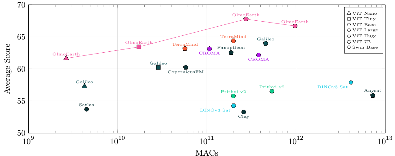
Figure 1 OlmoEarth defines a Pareto optimum of performance vs. computational efficiency averaged across 13 embedding tasks (measured by kNN and linear probing) 1 . The chart shows average multiply-accumulate operations to encode one example across all tasks (input size varies by task). See Table 2 for full results.
