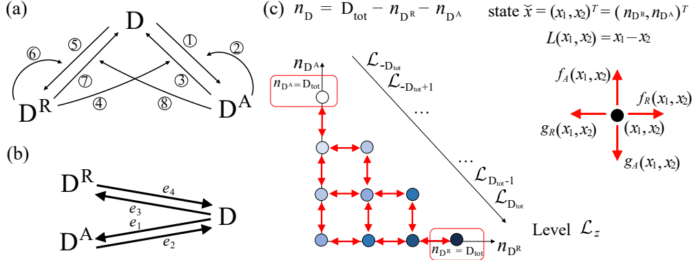
Fig. 4: Chromatin modification circuit including only histone modifications: reaction diagram, graph \mathcal{G} and associated Markov chain. (a) Chemical reaction system diagram. The numbers on the arrows correspond to the reactions associated with the arrows as described in (5.1) in the main text. (b) Graph \mathcal{G} associated with the chemical reaction system in panel (a). (c) State space and transitions of the projected continuous time Markov chain \tilde{X} = \{(X_1(t), X_2(t))^T : t \geq 0\} , which keeps track of (n_{D^R}, n_{D^A}) through time. Here, we consider D_{\text{tot}} = 3 and we use dots to represent the states, and red double-ended arrows to represent transitions in both directions. Additionally, we use shades of blue to distinguish the level to which each state belongs. The function L associated with the coclique level structure is L(x_1, x_2) = x_1 - x_2 . The rates associated with the one-step transitions for the projected Markov chain \tilde{X} are given in (5.2).
