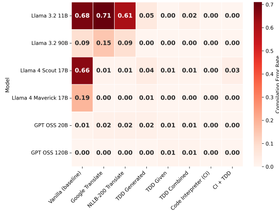
Figure 7: Compilation error rate heatmap of models in different approaches.
