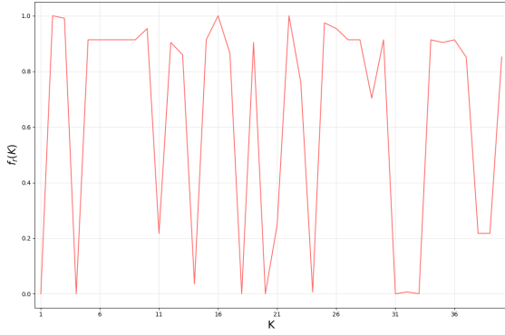
Fig. 4. Dependence of the red fraction of nodes f_r(K) on PageRank index K for the case of Fig. 2 ( K is obtained at damping factor \alpha = 0.85 ).
