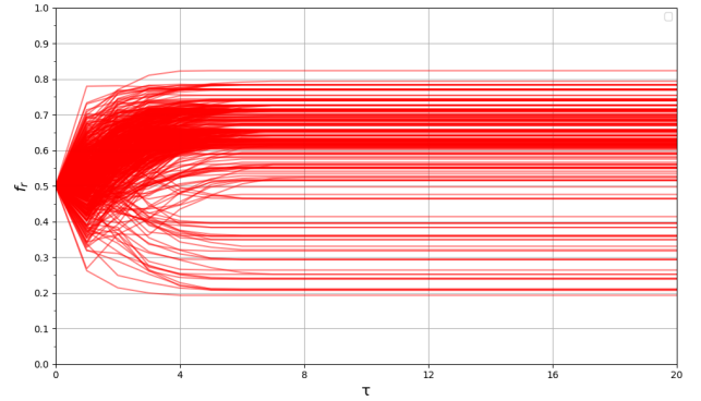
Fig. 1. Evolution of the fraction of red nodes f_r for N_r = 500 random pathway realisations. An initial condition has one red fixed node (Newman) and one blue fixed node (Barabasi); they remain fixed during an asynchronous Monte Carlo evolution based on the relation (1); all other nodes are initially white ( \sigma_j = 0 in (1)). Here x -axis represents time \tau of Monte Carlo process, where each unit of \tau marks one complete update of all nodes/spins following the INOF/GINOF model (here Z_c = 0; W = 0 ); steady-state configurations are reached at \tau = 20 (or earlier).
