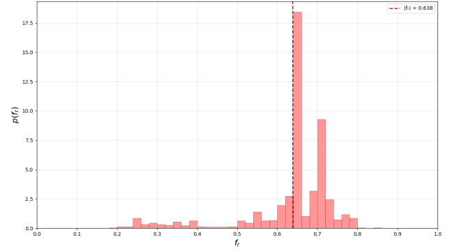
Fig. 2. Probability distribution p(f_r) of red node fractions; the histogram of f_r values is obtained with 50 cells 1 \leq m \leq 50 with normalization \sum_m f_r(m) = 1 , average red value is \langle f_r \rangle = 0.638 . Here there are N_r = 10^5 pathway realizations. Fixed nodes are Newman (red) and Barabasi (blue), all other nodes are white (spin zero). Initially all non-fixed nodes are white for the INOF model [or for the GINOF model at W = 0; Z_c = 0 ]. Vertical dashed line marks the average red value \langle f_r \rangle .
