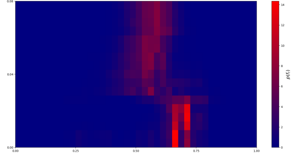
Fig. 7. Probability of red nodes p(f_r) shown by color as the function of x = f_r (taken for 40 columns in the range 0 \leq f_r \leq 1 ) and y = W (taken for 17 W equidistant values in the range 0 \leq W \leq 0.08 ) for the case with the opinion conviction threshold Z_c = 0.1 in the GINOF model (there are in total N_{cell} = 680 cells). Data are obtained with N_r = 10^4 pathway realizations for each W value.
