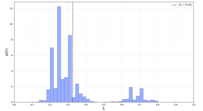
Fig. 3. Same as Fig. 2, but with initial state of node Sole being blue; \langle f_r \rangle = 0.326
