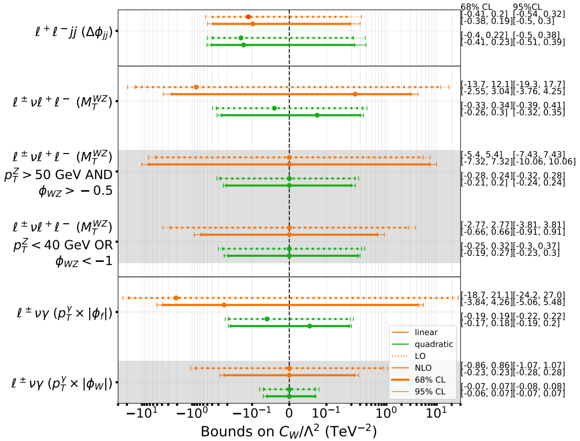
Figure 4.12: 68% and 95% CL bounds on C_W/\Lambda^2 at LO (dotted) and NLO (continuous), with the inclusion of the quadratic term or without, for the processes presented in this chapter. The variables we used are noted next to the process names: there are two different ones for W\gamma . The limits in the inclusive case and over the regions (4.7) are shown for WZ . The limits with gray background come from comparison with the best SM distributions, the others with real data; a summary of the experimental measurements can be found in Table 4.5. The numerical values are on the right
