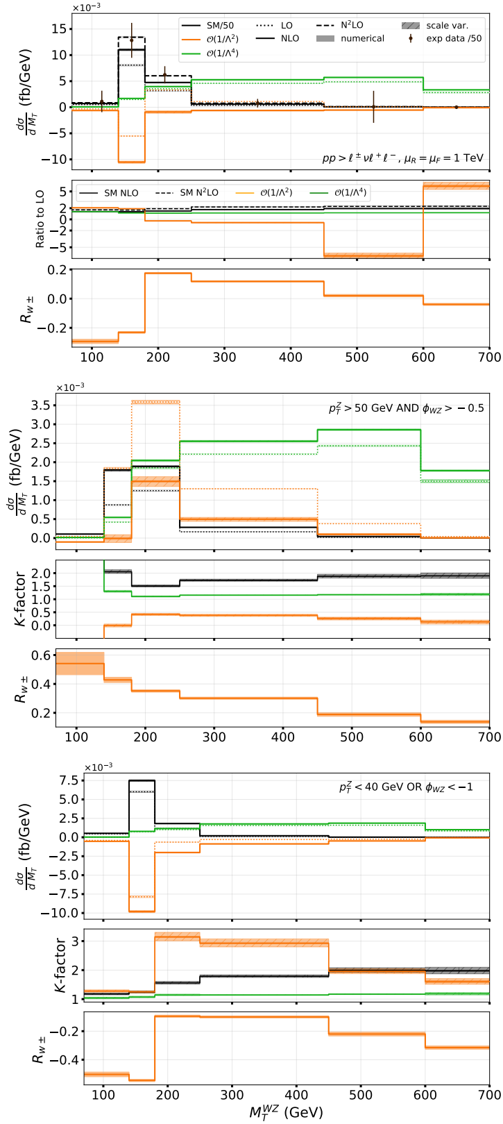
Figure 4.8: Same as Fig. 4.7 but for the transverse mass of the WZ system. In the top plot, the N^2LO results at FO for the SM and the experimental data are also shown. The last bin contains the overflow
