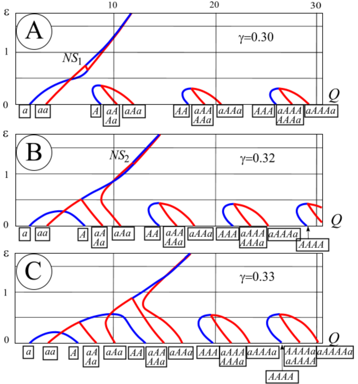
FIGURE 2. Bifurcations of branches of ILMs for the case (p, q) = (3, 4) : Panel A: \gamma \approx 0.30 ; panel B: \gamma \approx 0.32 ; panel C: \gamma \approx 0.33 . Values of \varepsilon are shown versus Q(\mathbf{u}) = \sum_{n \in \mathbb{Z}} u_n^2 . Parts of the branches that correspond to stable (unstable) solutions are shown in blue (red).
